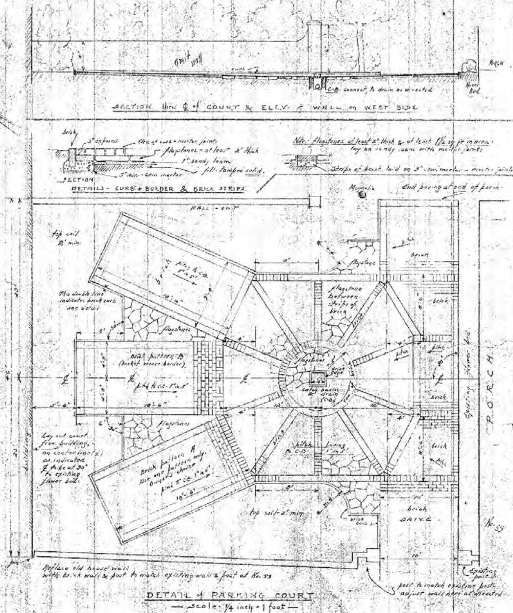
CONSTRUCTION PLAN & GROUNDS — at 59 Church St. — Charleston, S.C. — for Mr. & Mrs. Henry P. Staats.
