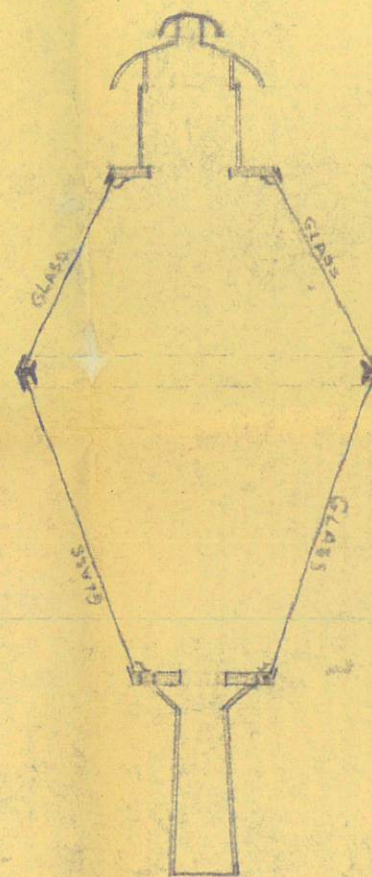
GROSS SECTION
