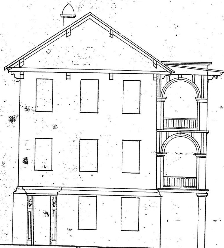
— Grand Elevation —
