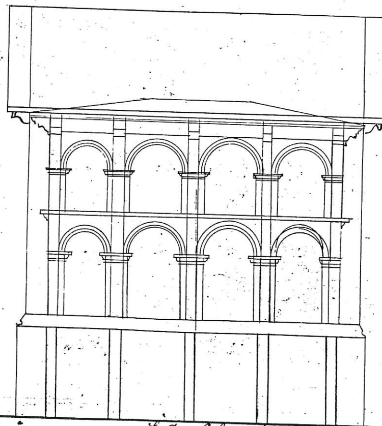
Side Elevation
