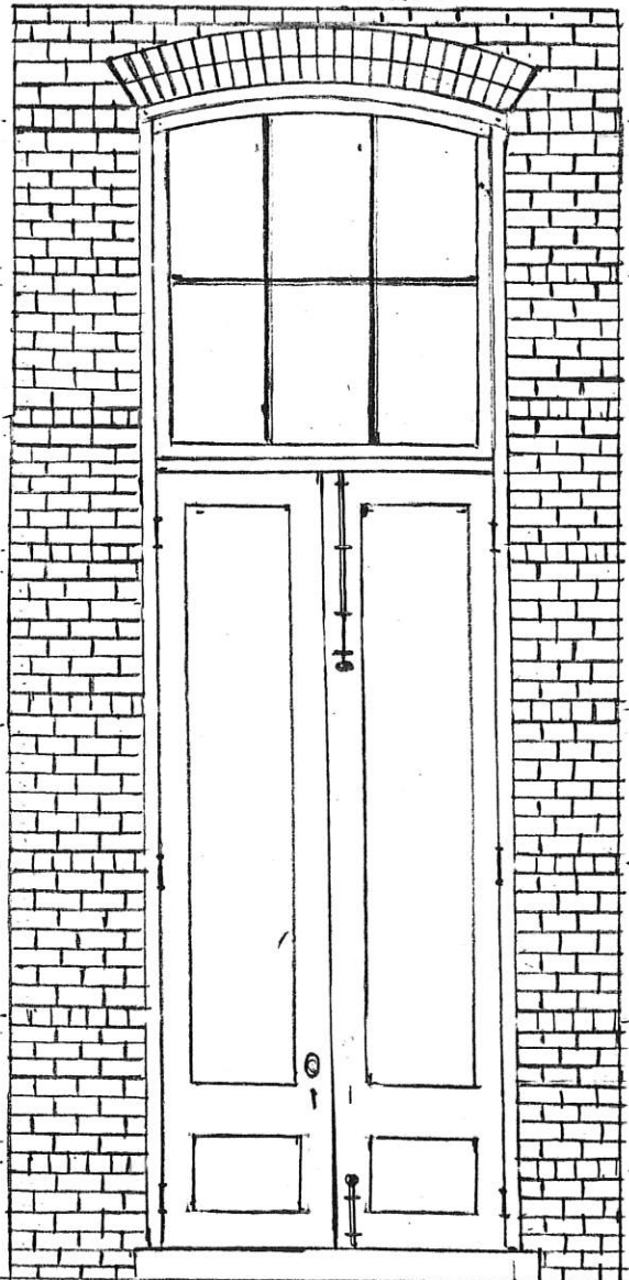
BACK·VIEW
