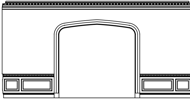
I9/A3.1 1/2" = 1'-0"
