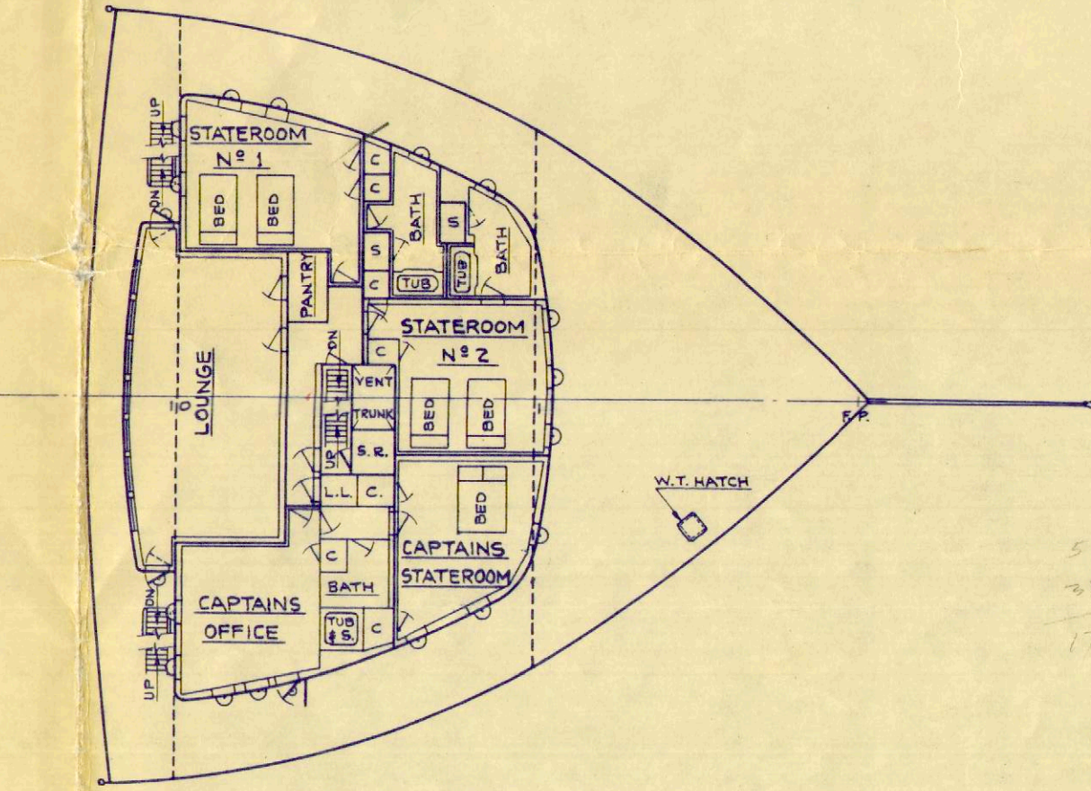
FORECASTLE DECK
