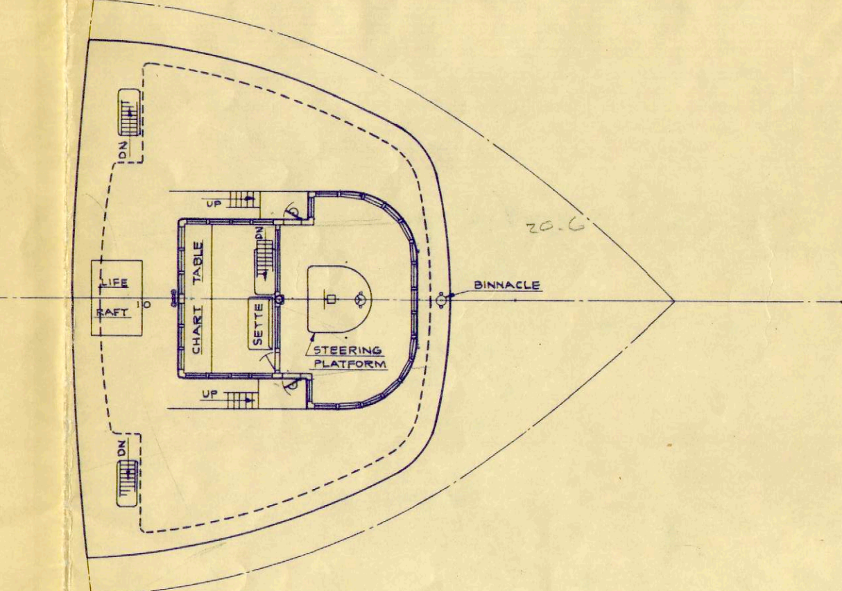
TEXAS DECK
