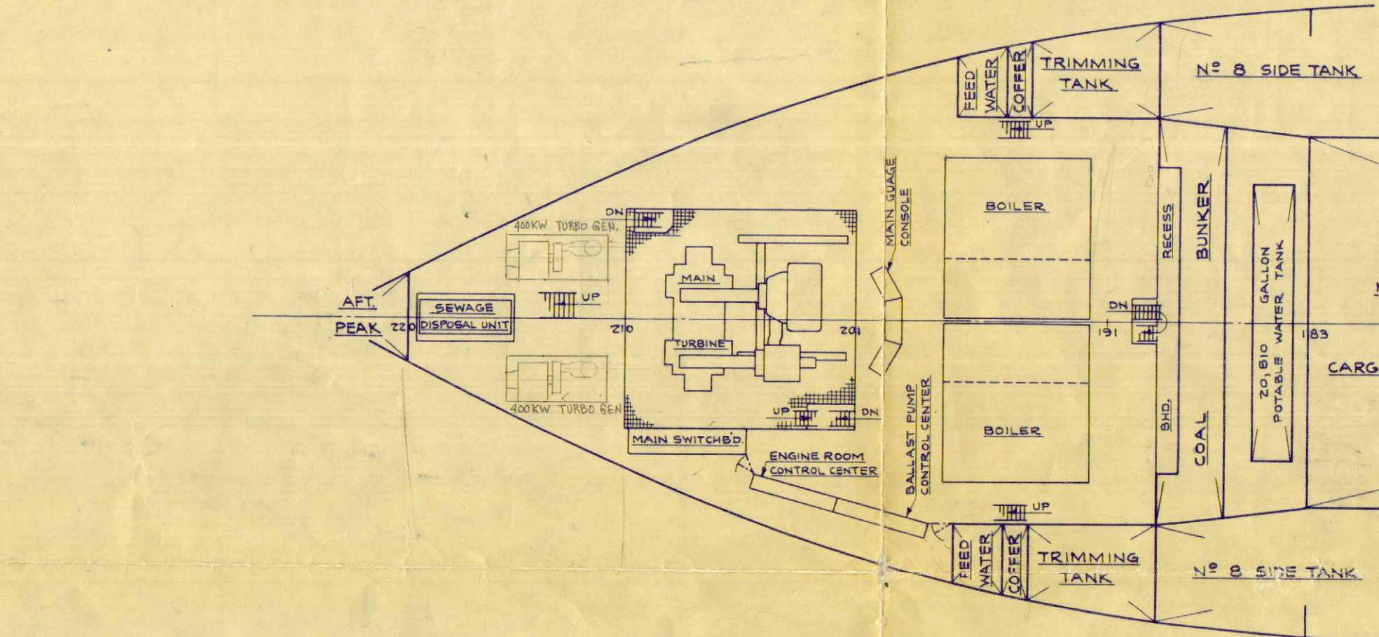
OPERATING DECK
