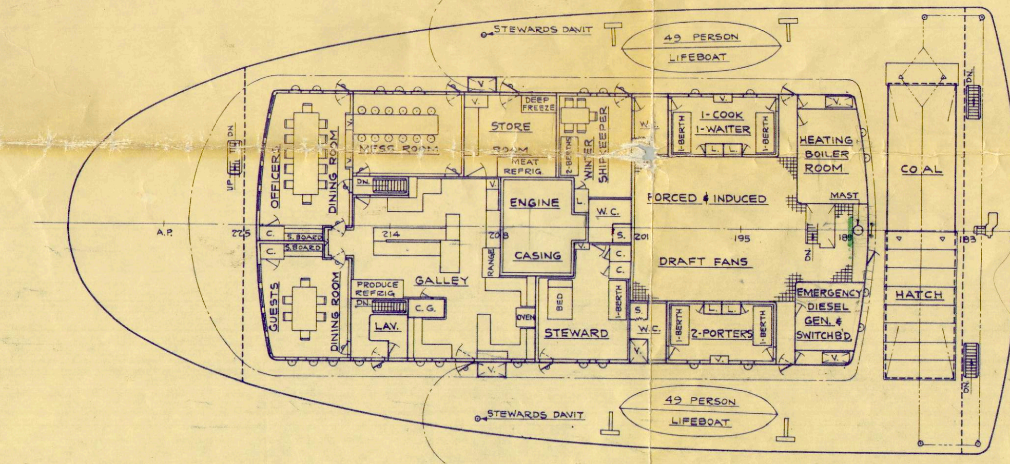
POOP DECK
