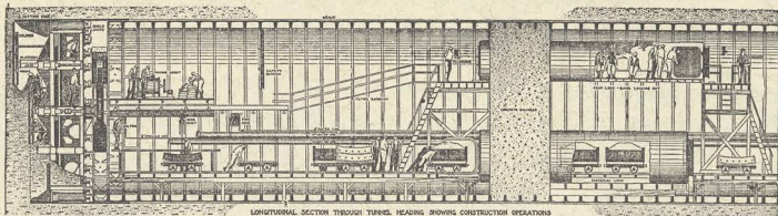
LONGITUDINAL SECTION THROUGH TUNNEL HEADING SHOWING CONSTRUCTION OPERATIONS
