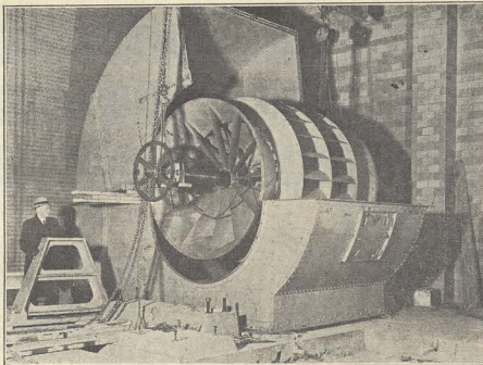
One of the 32 huge ventilation fans is shown as it was being installed in the Weehawken ventilation building. A portion of the outer casing has been removed to show the many-finned wheel which forces fresh air through the mile-long tube. The size of the fan can be seen by comparing it to the size of the man standing at the left of the photo. These fans can supply the South or completed tube with a maximum of 1,736,000 cubic feet of air per minute. The fan motors have a maximum operating horsepower of 2,237.
