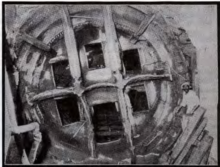
Inside the burrowing shield that bored the H & M tubes beneath the Hudson River.
