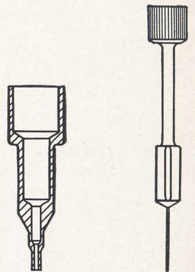
Leroy Lettering Pen enlarged two and a half times, showing tube and cleaner
