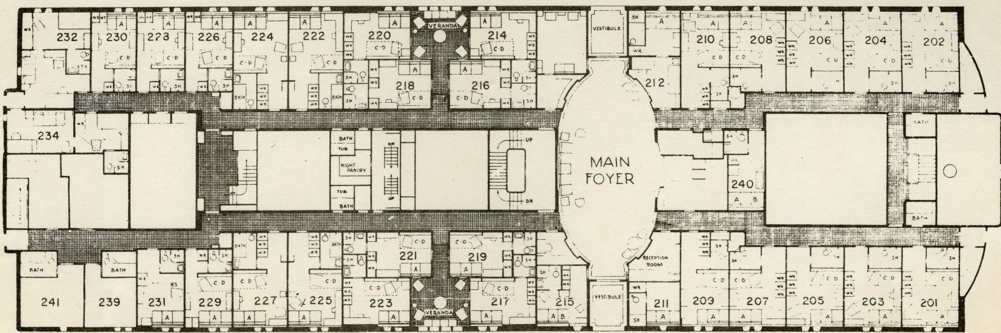
"A" DECK GANGWAY
