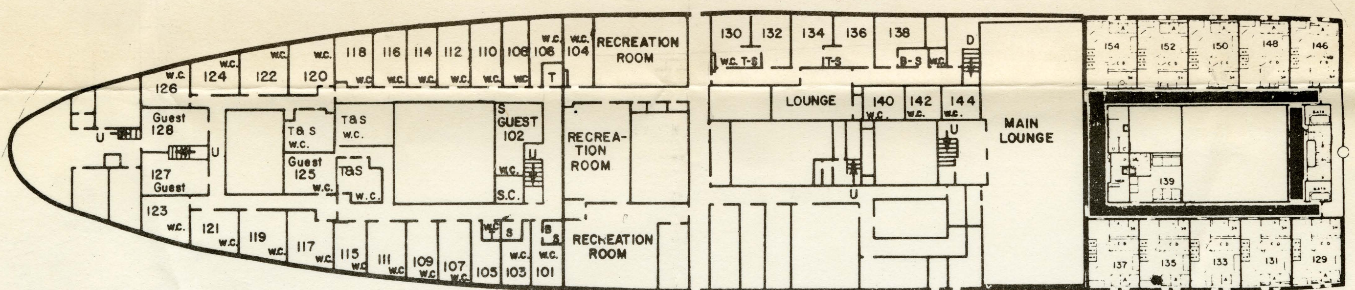
"B" Deck
