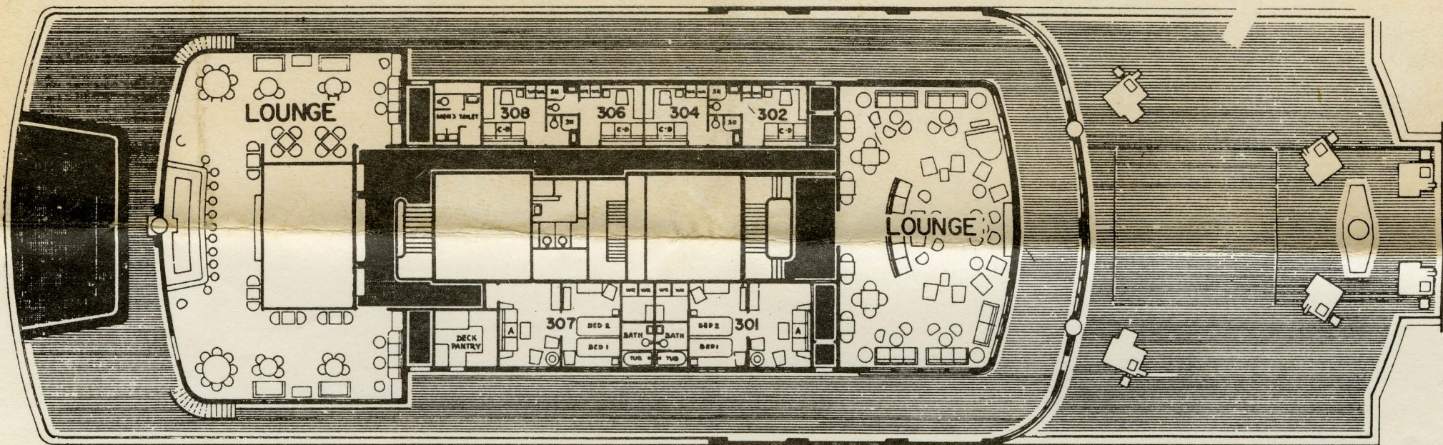
PROMENADE DECK
