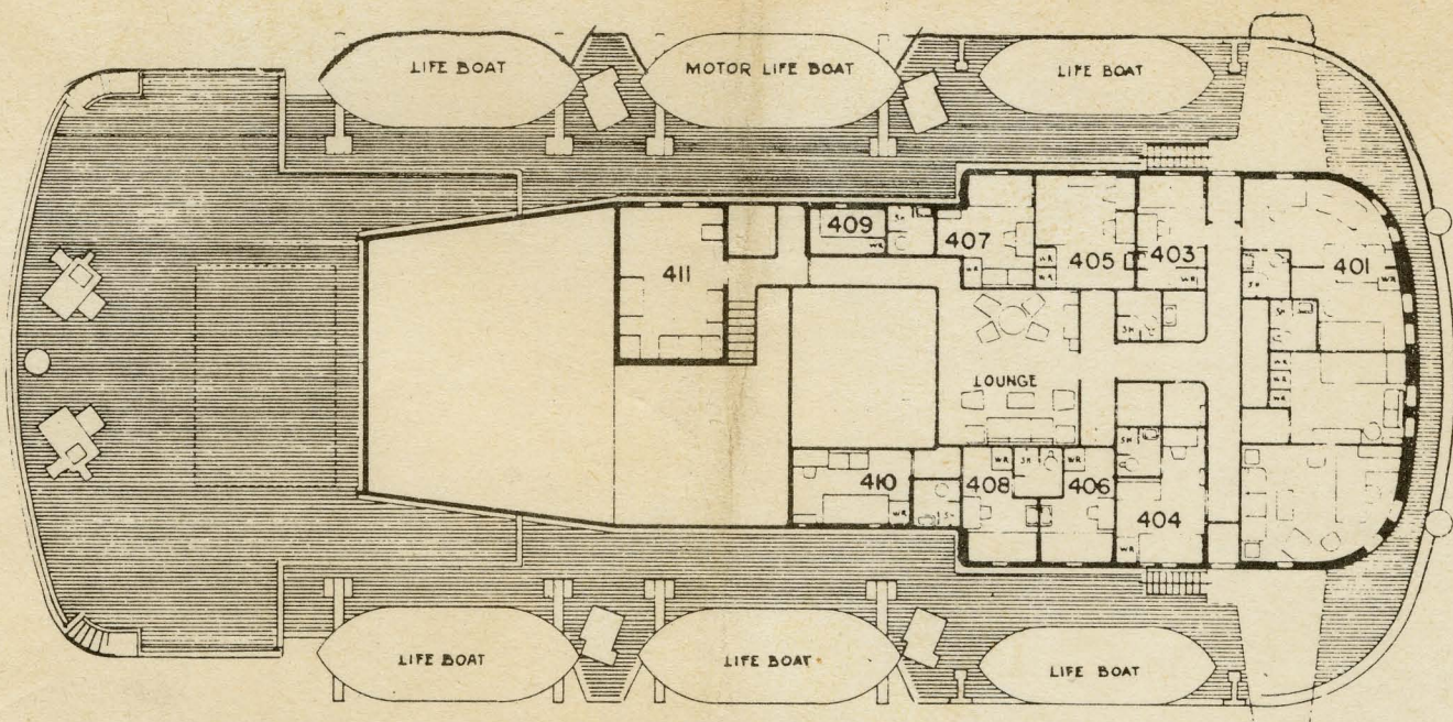
BOAT DECK
