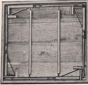
Cross Cleats Locked into Frame by Steel Plates
