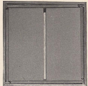
Showing Cross Cleat Supporting Top
