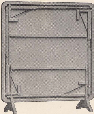
Cross Cleats Locked into Frame by Steel Plates
