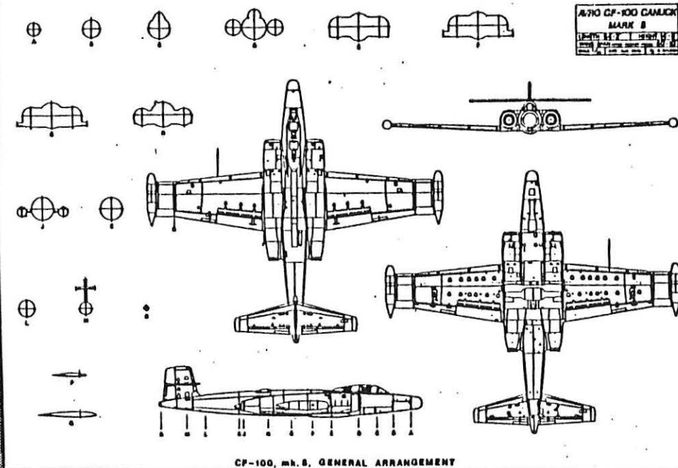
CP-100, mk. 5, GENERAL ARRANGEMENT
