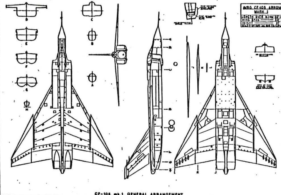
CF-105, mk. 1, GENERAL ARRANGEMENT
