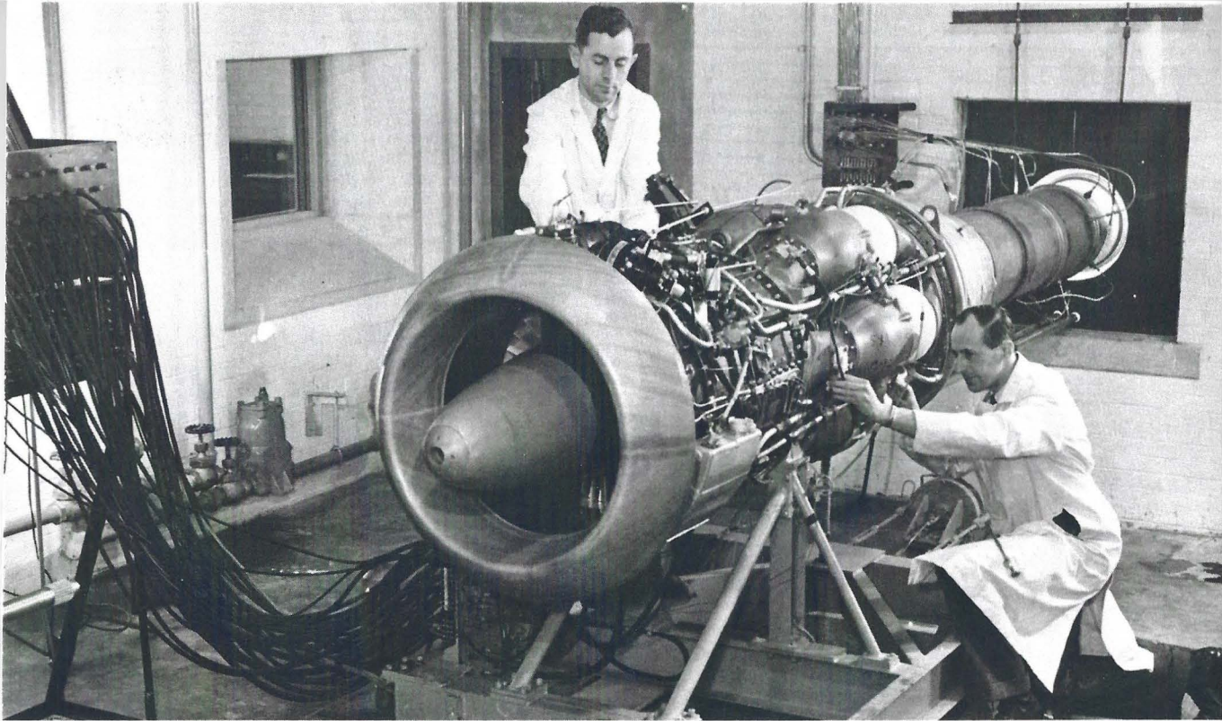
First Chinook gas turbine engine under test with Ed Caswell on the left and Max Nerriere on the right.
