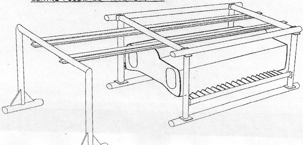
CENTRE FUSELAGE ASSEMBLY JIG
