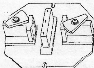
③ COMPLEX PART MADE FROM BAR STOCK, THIS PART REQUIRES THE USE OF MORE COMPLEX TOOLING TO ENSURE THE NECESSARY INTERCHANGEABILITY
