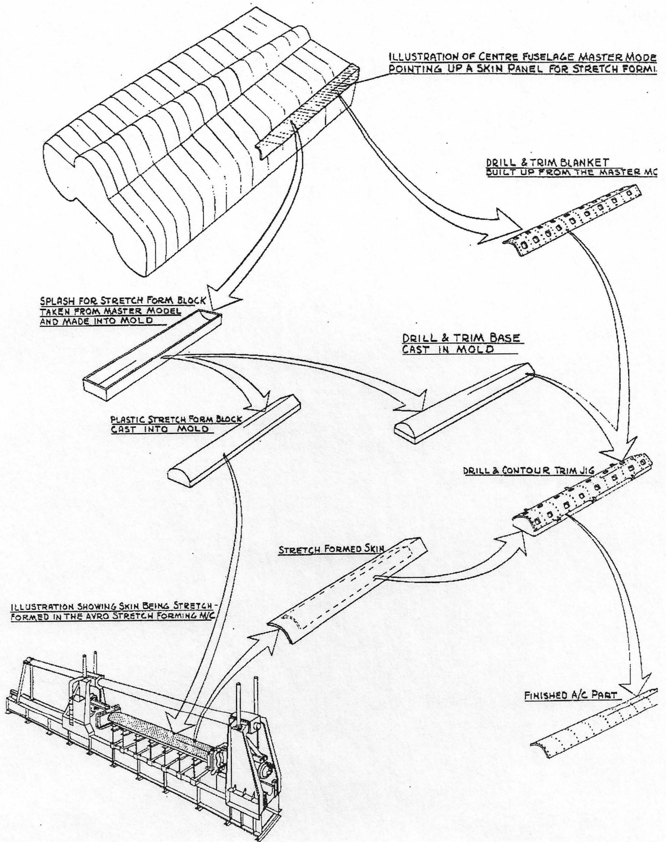
APPLICATION OF MASTER MODEL IN TOOLING FOR DOUBLE CURVATURE SKIN P
