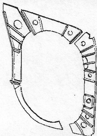
EXPLODED VIEW OF STA. 268
