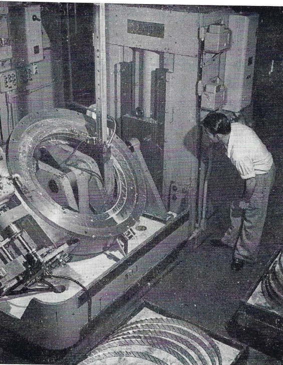
Broaching machines on stator blade rings.
