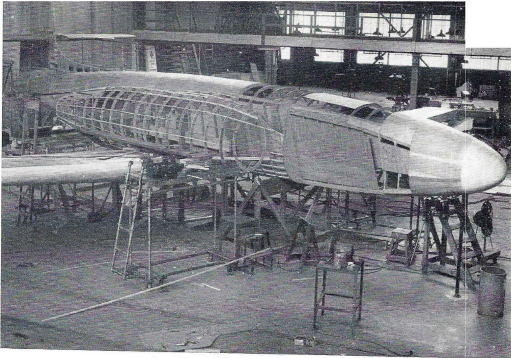
CF-100 wooden mockup— . . . essential stage in aircraft development began in 1947.
