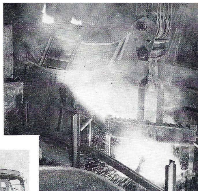
Tapping an electric furnace.
