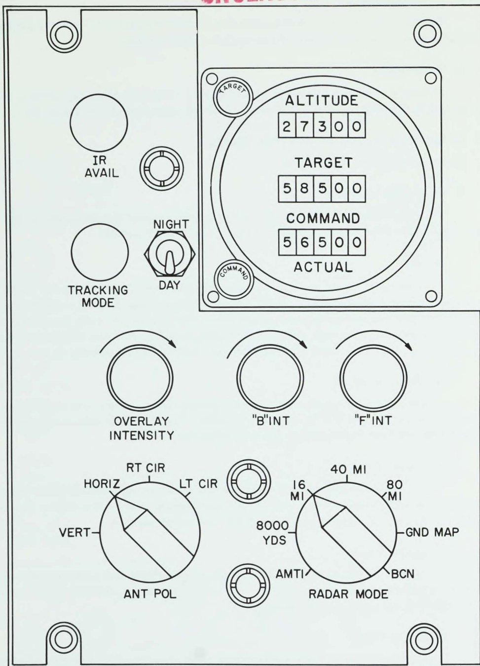
Figure 47. Observer's Radar/IR Controls
