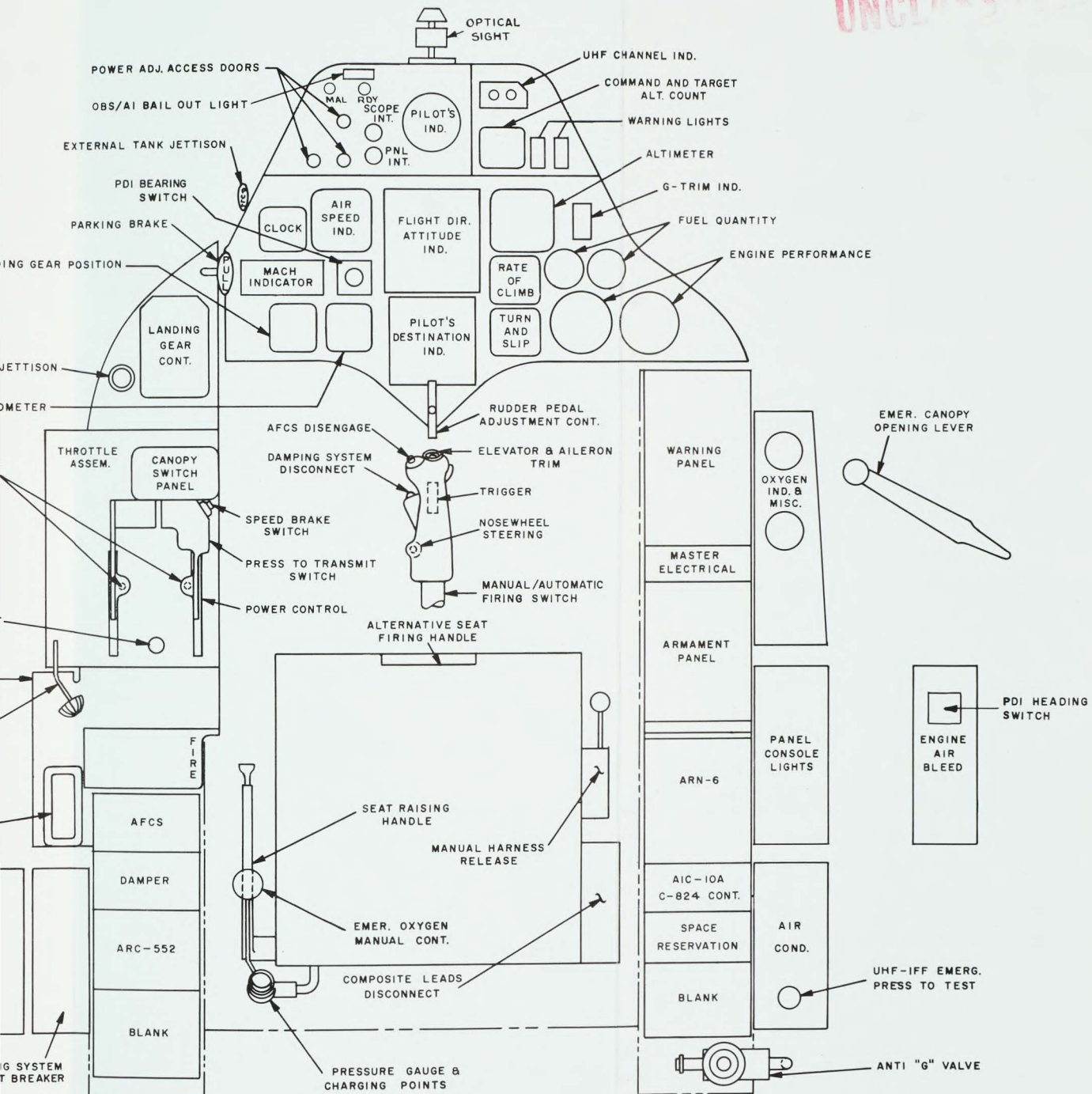
Figure 1. Layout of Pilot's Cockpit
