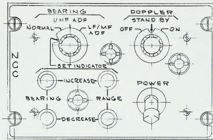
Figure 58. Navigation-Computer Control Panel
