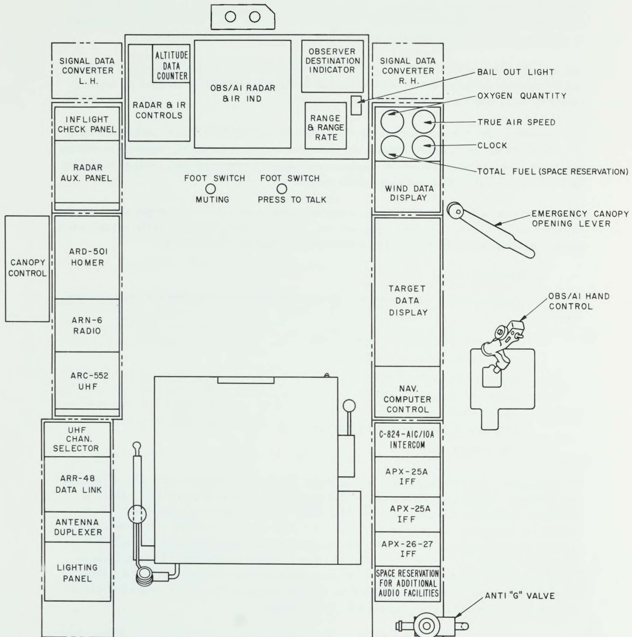
Figure 2. Layout of Observer's Cockpit
