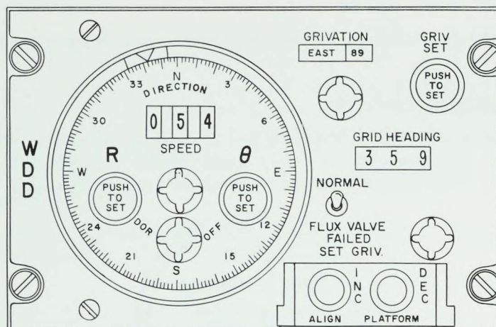
Figure 56. Wind-Data Display
