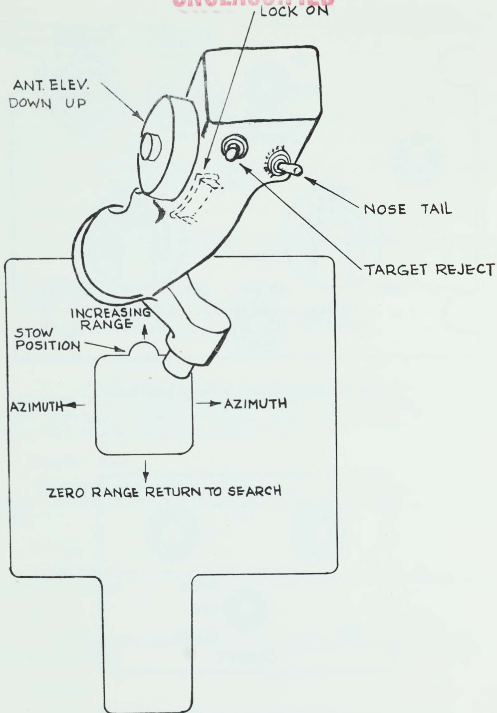
Figure 64. Radar Hand Control
