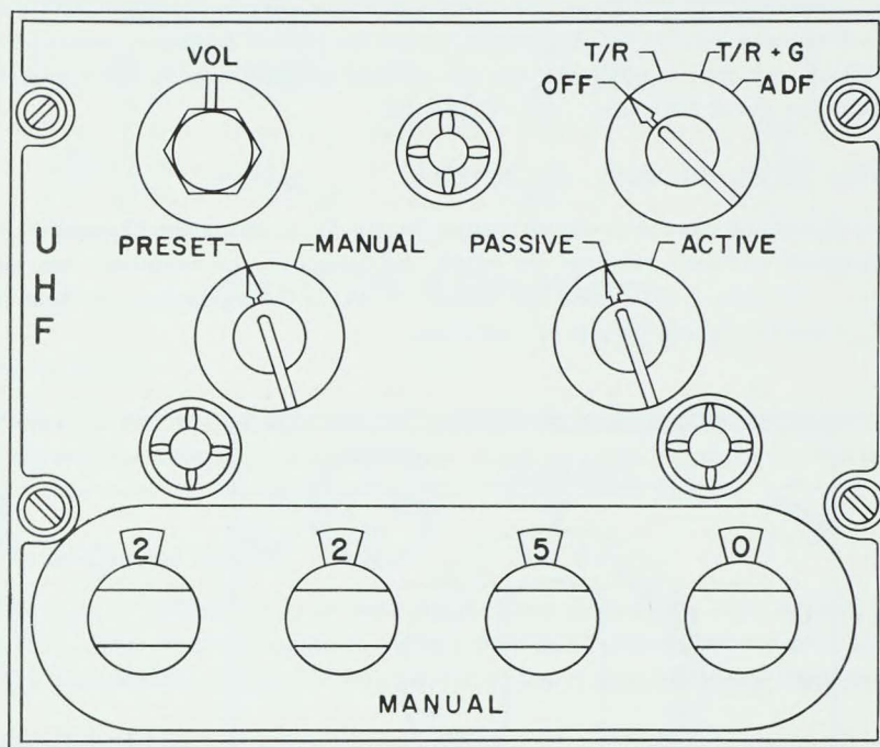
Figure 51. ARC-552 Control Panel (OBS/AI)
