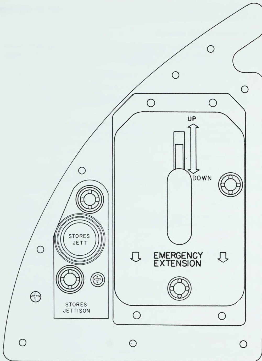
Figure 30. Landing-Gear Control and Stores Jettison Button
