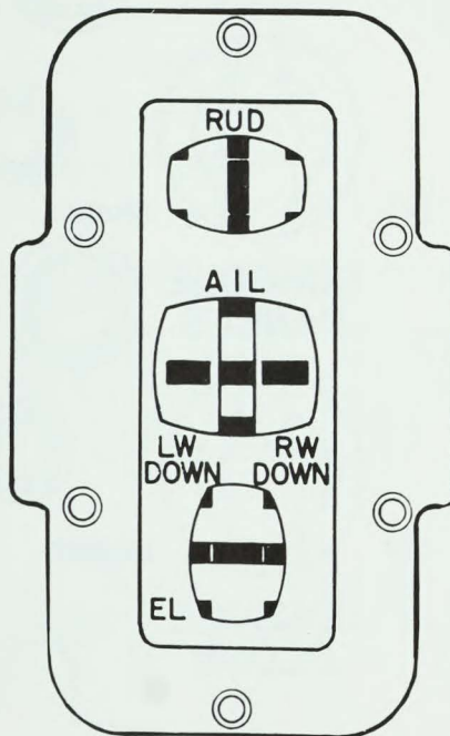
Figure 36. Control-Surface Position Indicator
