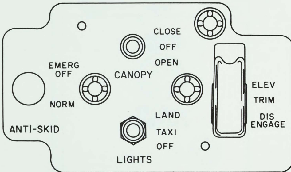
Figure 42. Pilot's Canopy Switch Panel
