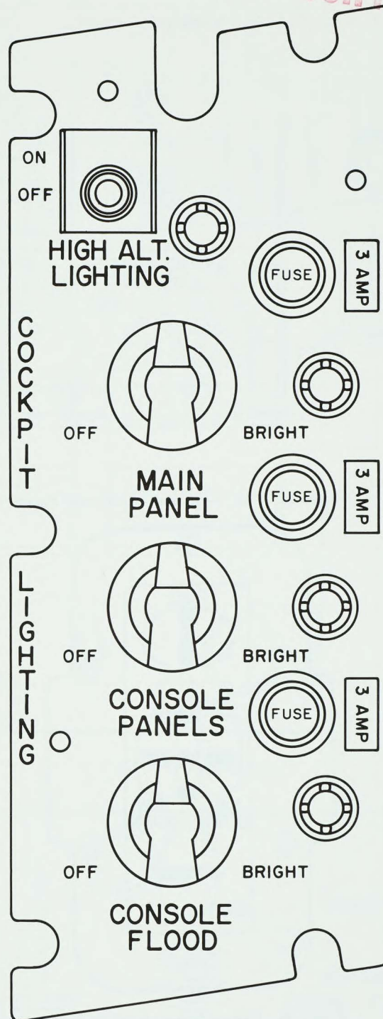
Figure 34. Pilot's Panel and Console-Lights Control Panel
