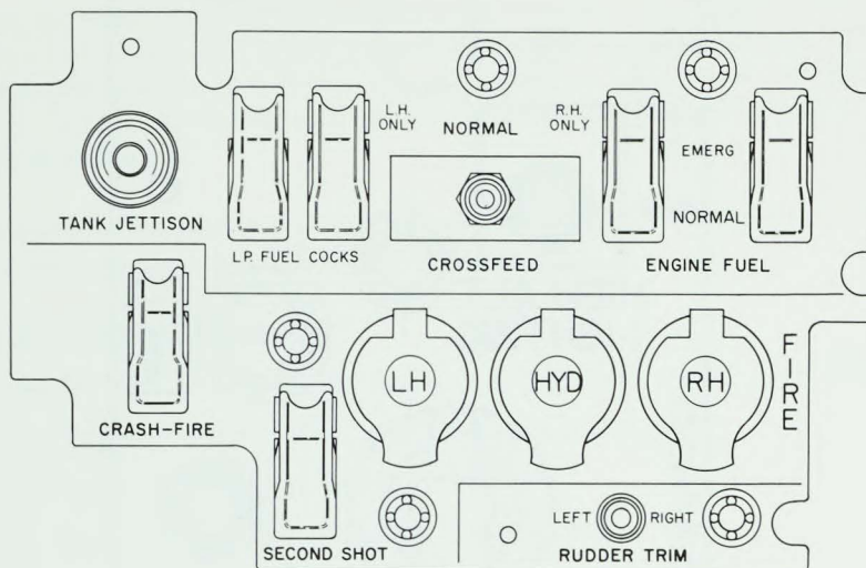
Figure 35. Fire, Fuel, and Trim-Control Panel
