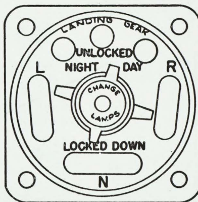
Figure 21. Landing-Gear Position Indicator
