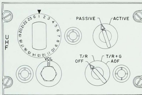
Figure 28. ARC-552 UHF Control Panel (Pilot)
