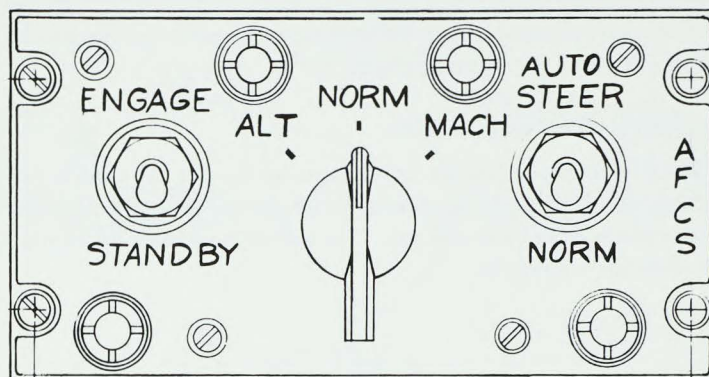
Figure 26. AFCS Control Panel
