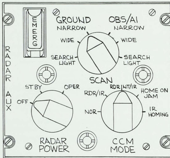
Figure 50. Radar Auxiliary Control Panel
