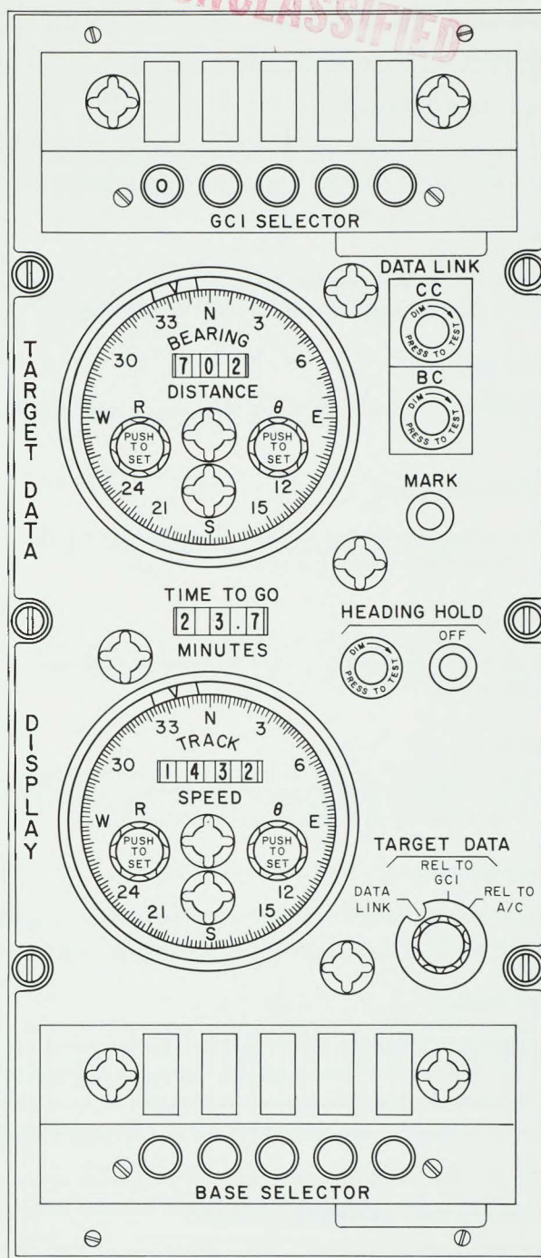
Figure 57. Target-Data Display
