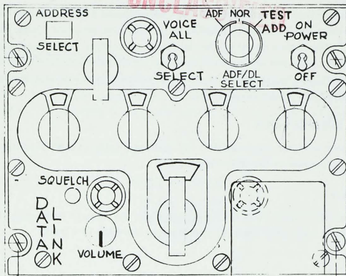
Figure 53. ARR-48 Data-Link Control
