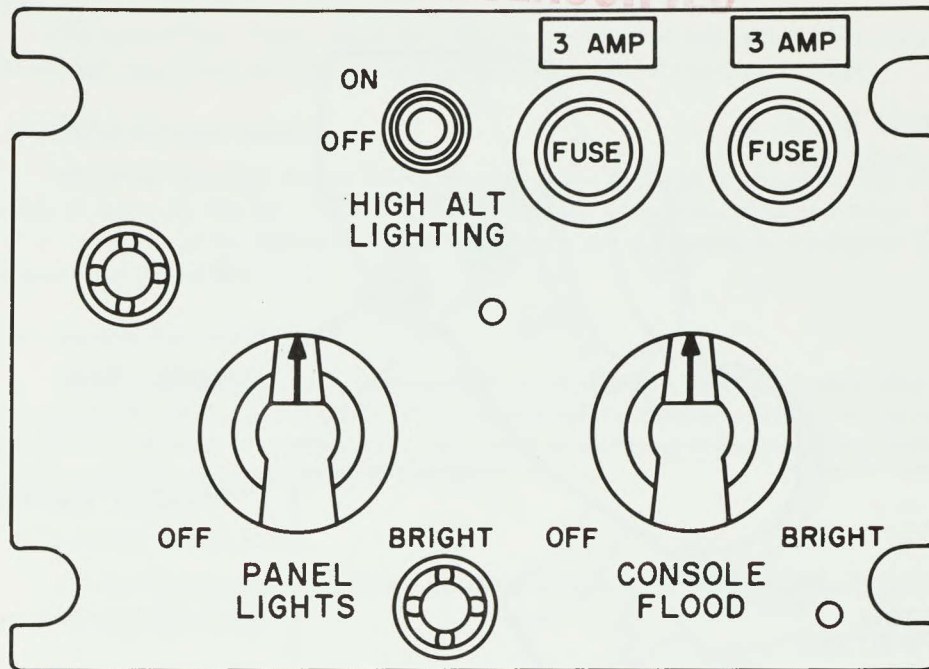
Figure 62. Observer's Panel and Console Lights Control
