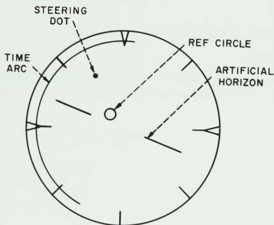
Figure 4. Display for a Lead-Collision Attack with Rockets
