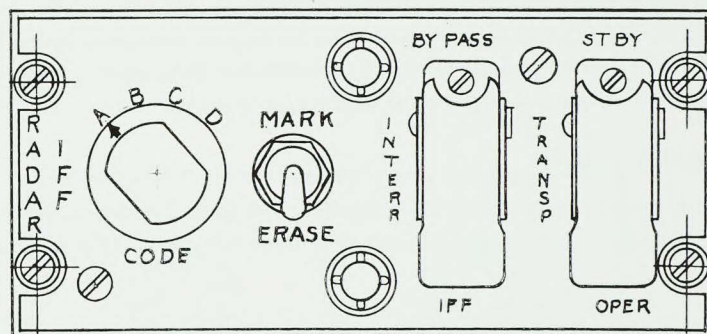
Figure 61. APX-26/27 Control Panel
