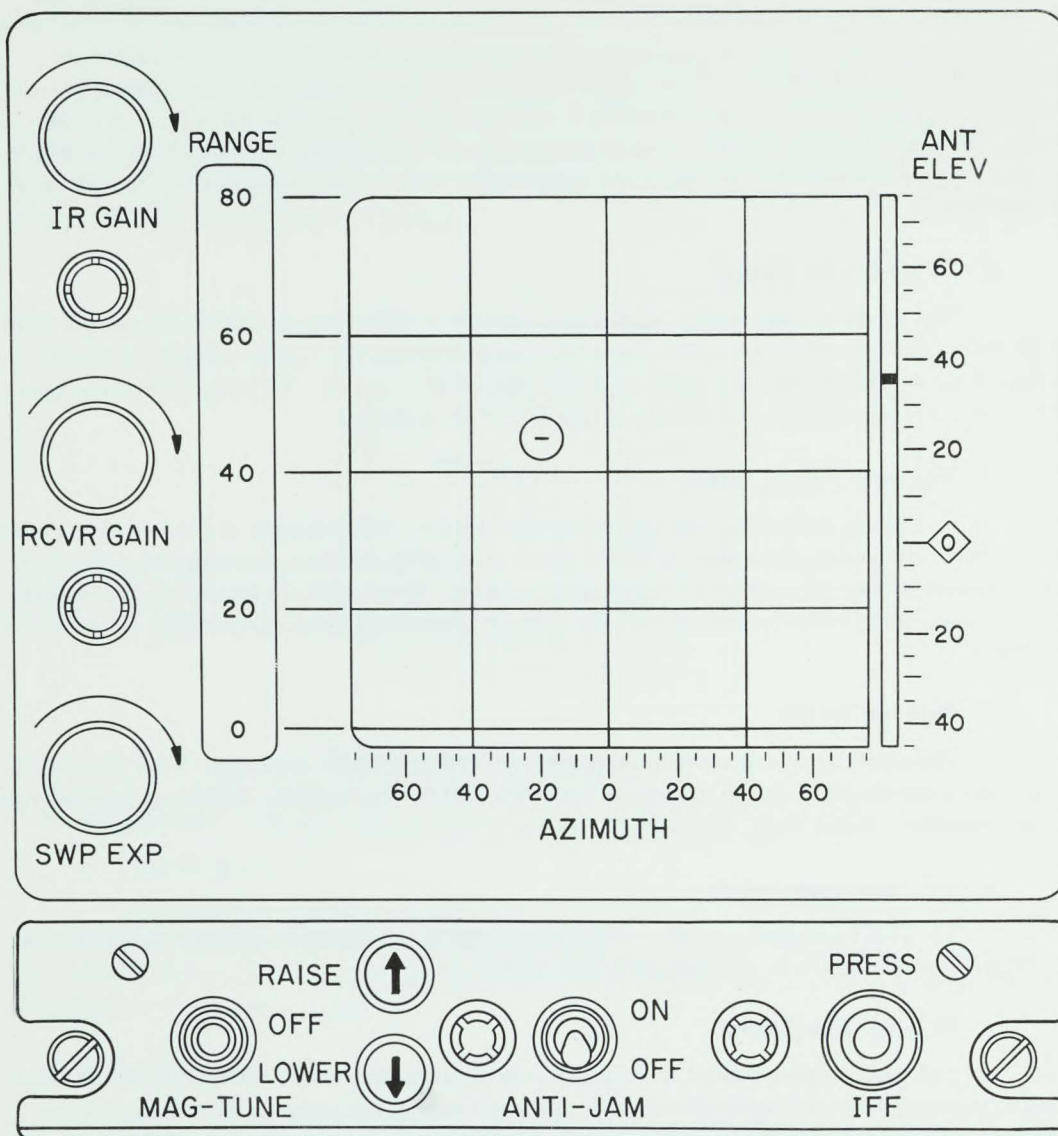
Figure 46. Observer's Radar and IR Indicator and Controls
