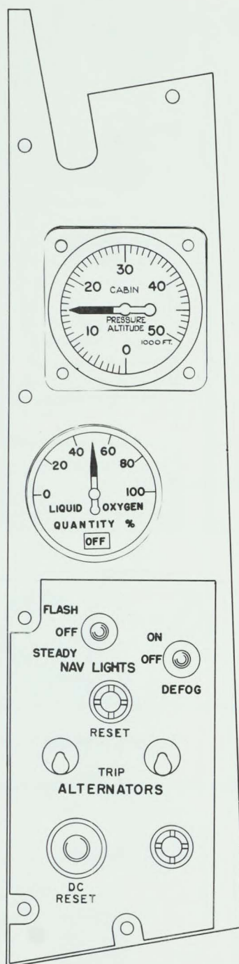
Figure 39. Oxygen Indicator and Miscellaneous Controls
