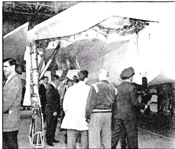
Main undercarriage twists and shortens when retracting. Main gear is by Dowty; nose gear by Jarry. Note extended and notched leading edge. Depth of wheel well is indication of wing's extreme thinness.
