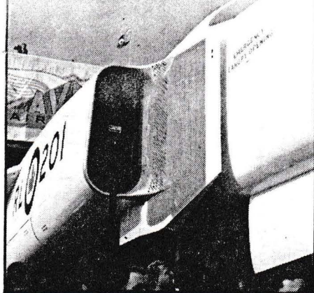
Chisel-edged intake ramp has multitude of approximately \frac{1}{2} in. diameter holes at inlet's lip, probably comprising some form of boundary layer bleed.
