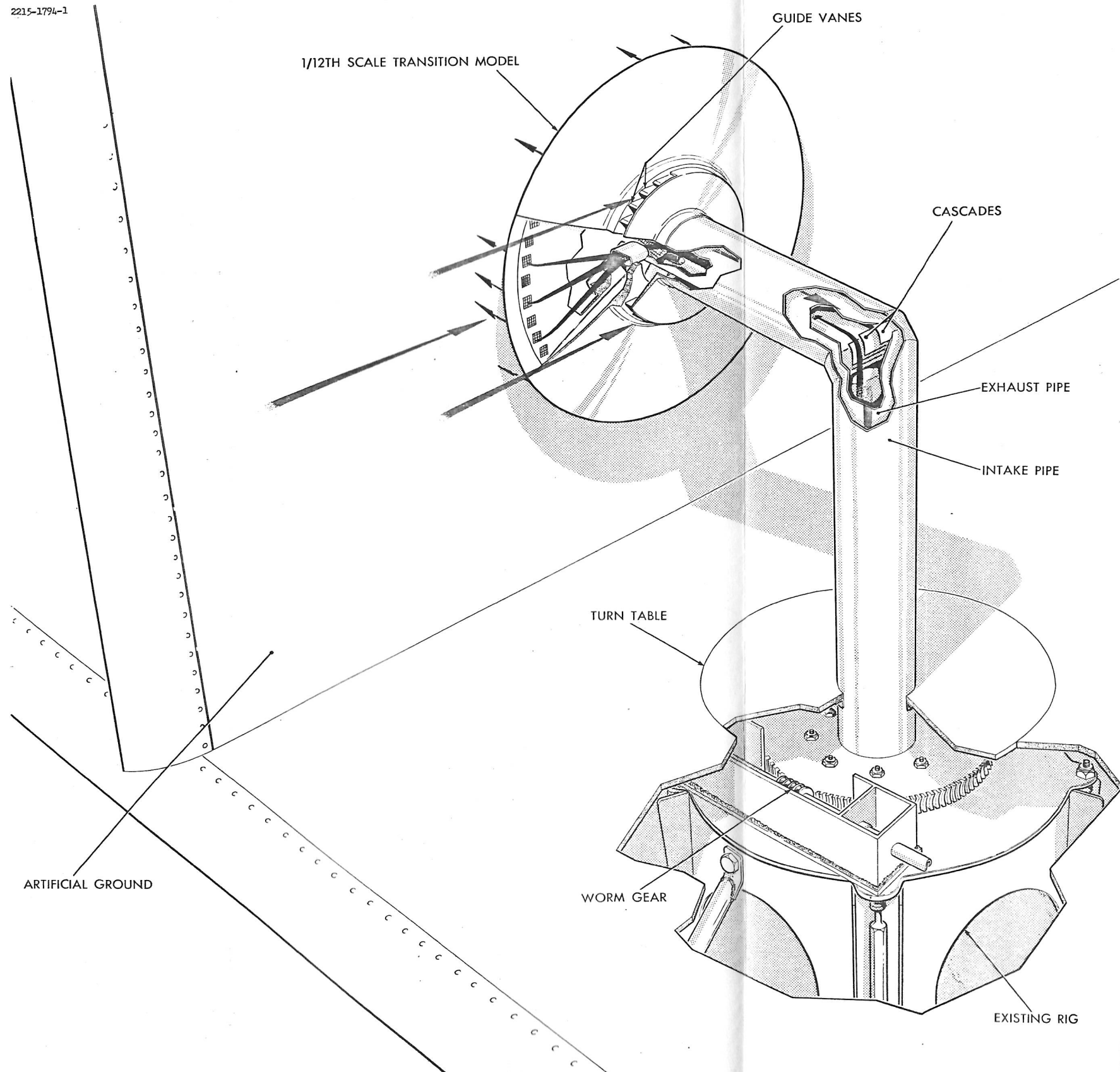
FIG. 11 PROPOSED 1/12TH SCALE TRANSITION MODEL
