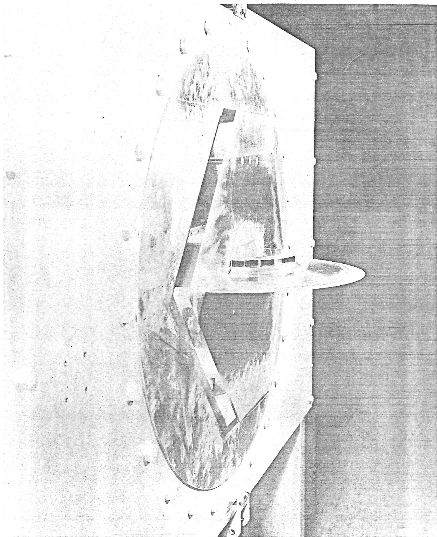
FIG. 21 1/23 SCALE SUPERSONIC MODEL
