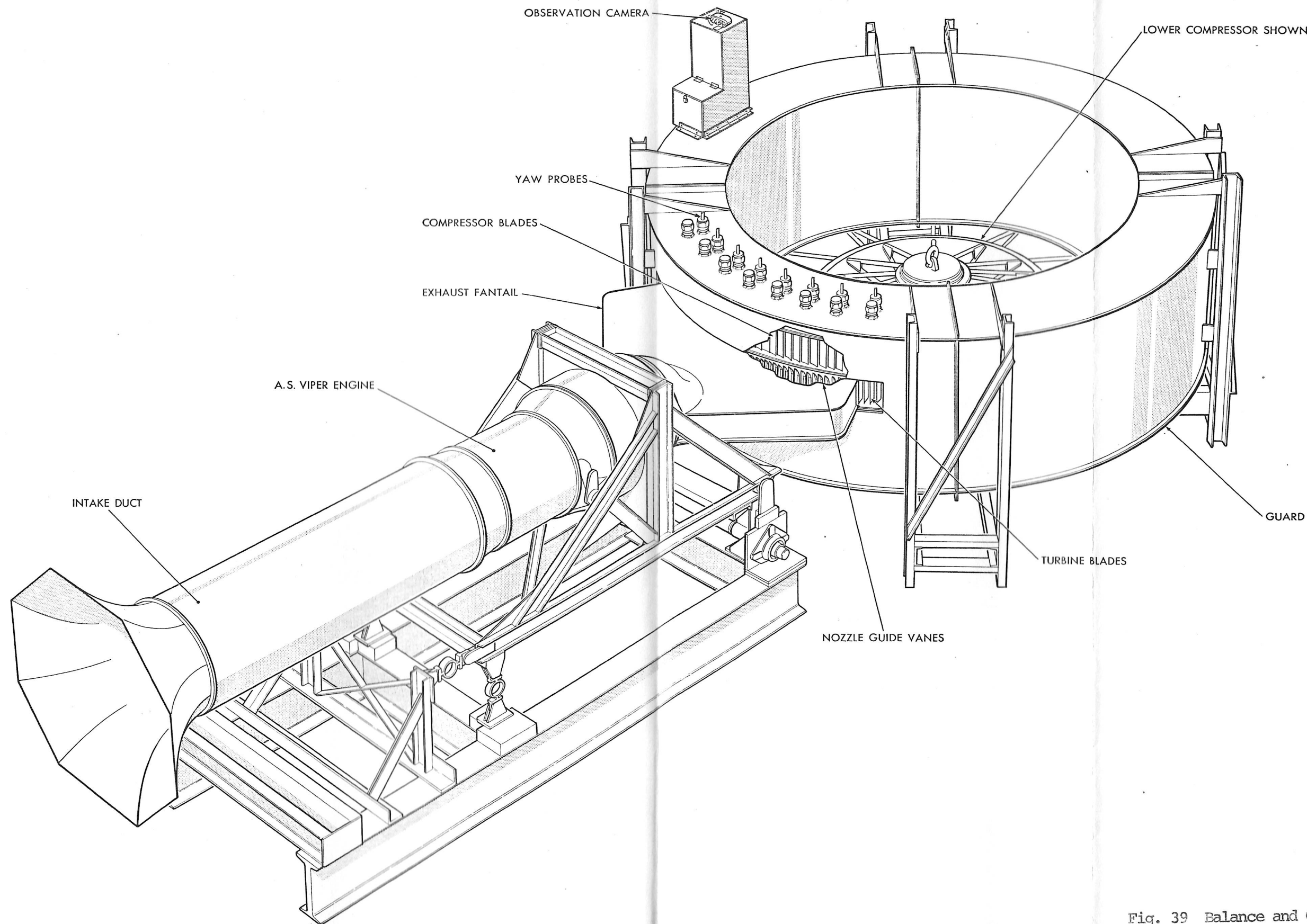
FIG. 39 BALANCE AND OVERSPEED RIG
