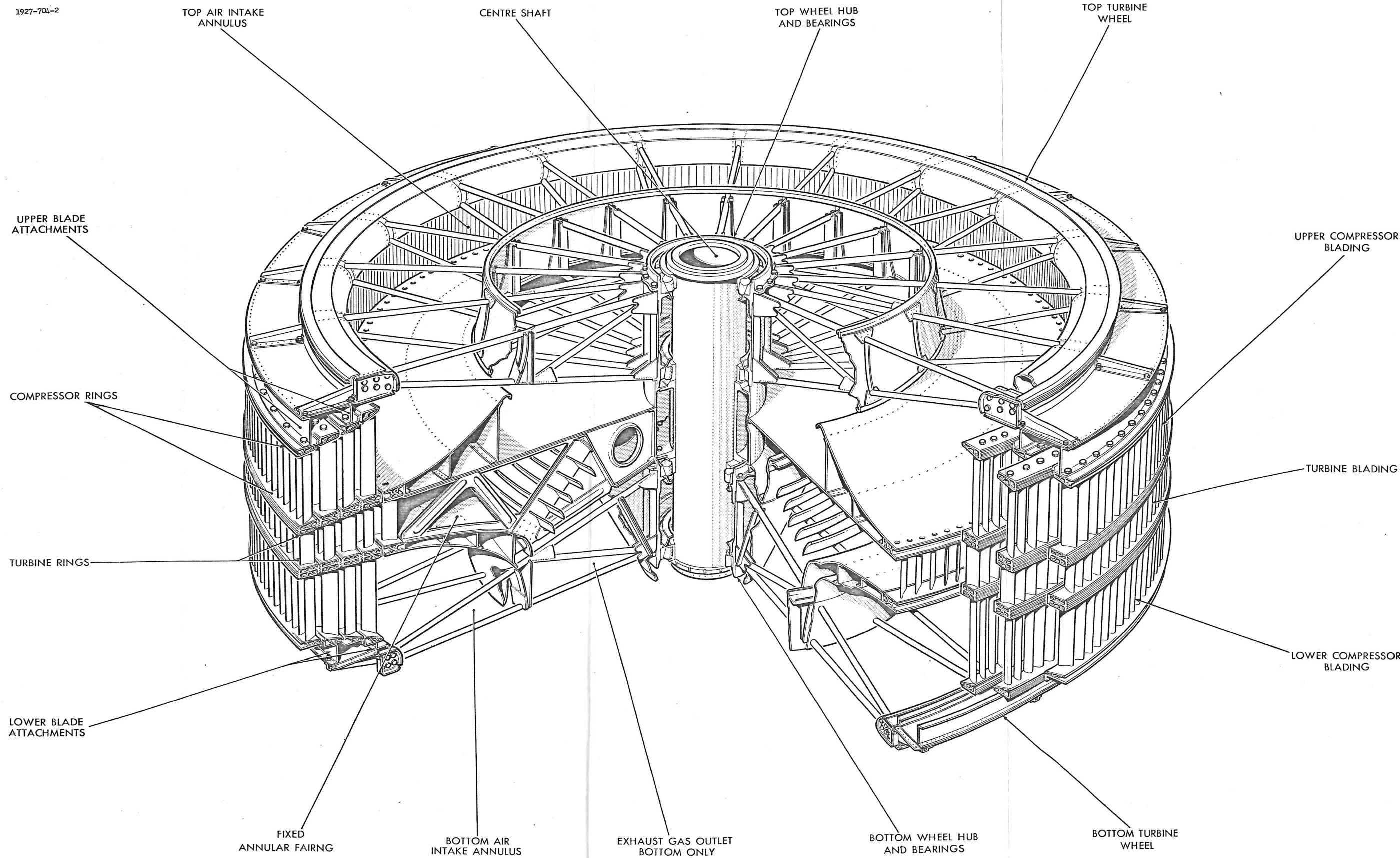
FIG. 3 TURBINE-COMPRESSOR ASSEMBLY
