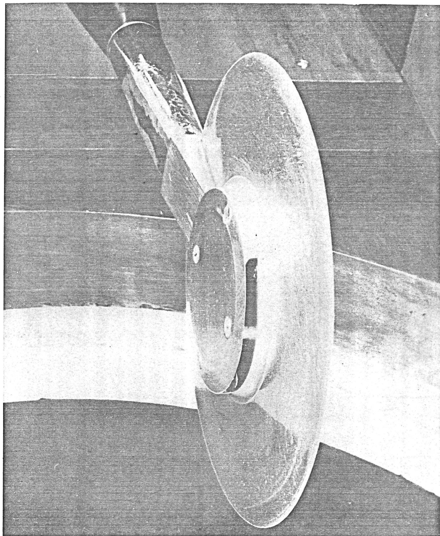
FIG. 19 1/40 SCALE STING MOUNTED MODEL
