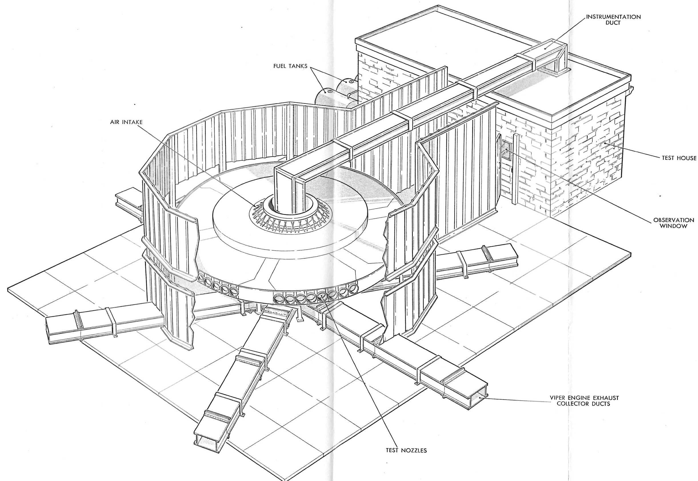
FIG. 40 TEST HOUSE AND SIX VIPER TEST RIG
