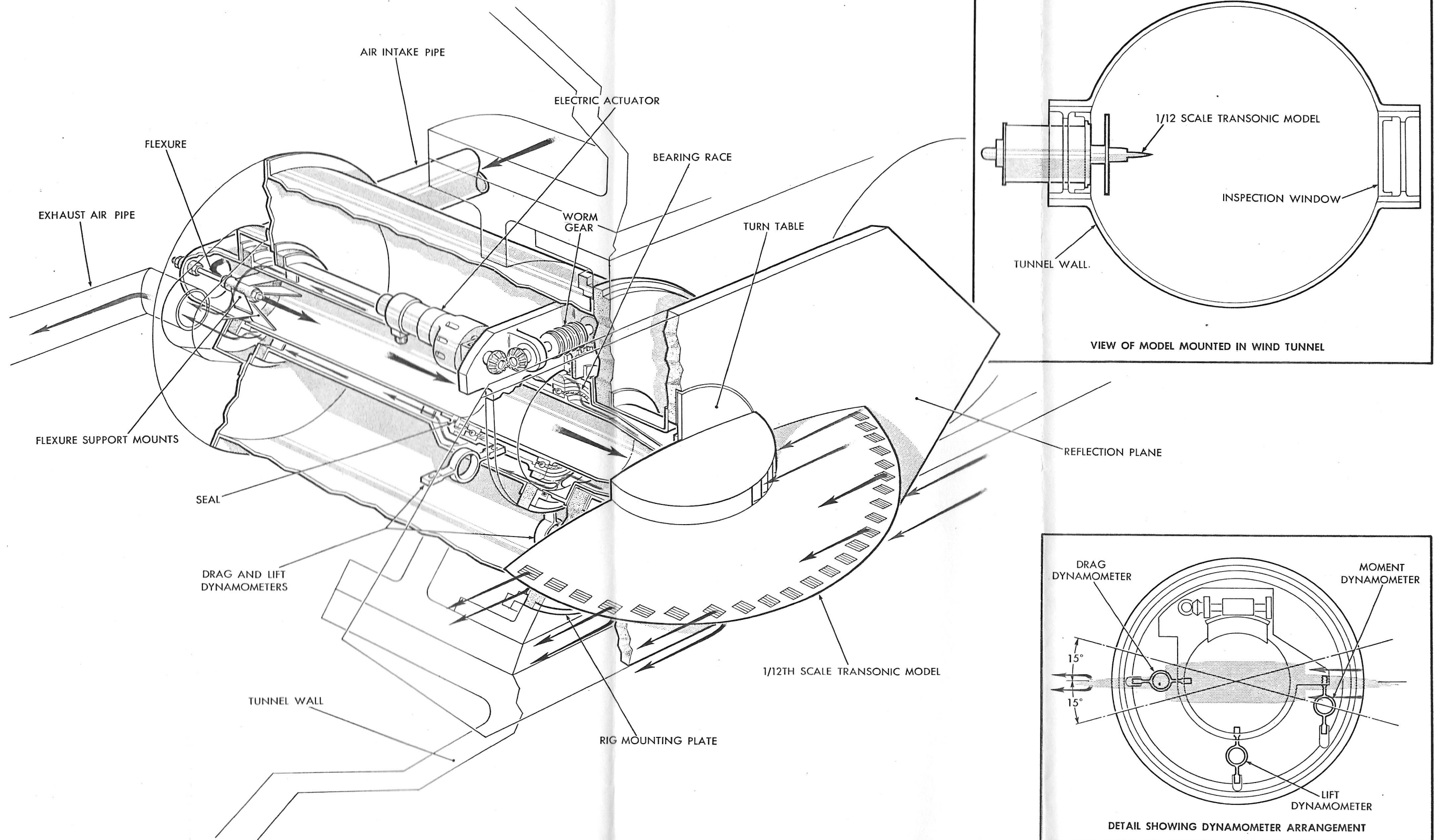
FIG. 14 PROPOSED 1/12TH SCALE TRANSONIC REFLECTION PLANE MODEL
