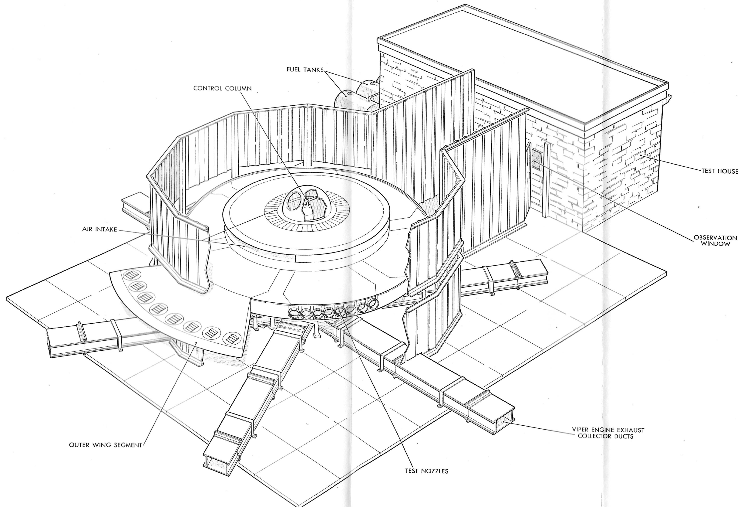
Fig. 44 Six Viper Test Rig with Outer Wing and Cockpit
