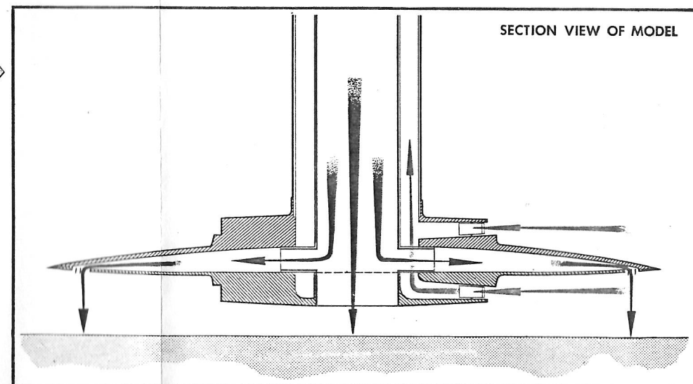
Fig. 11 Proposed 1/12 th Scale Transition Model
