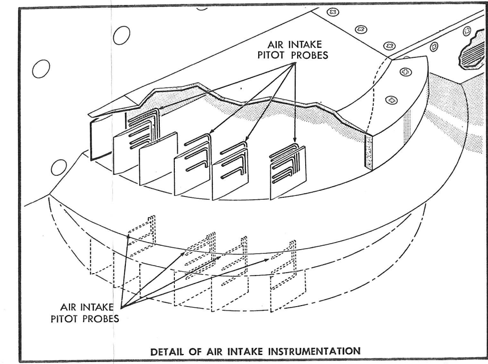
Fig. 16 2/25th Scale Air Intake Model
