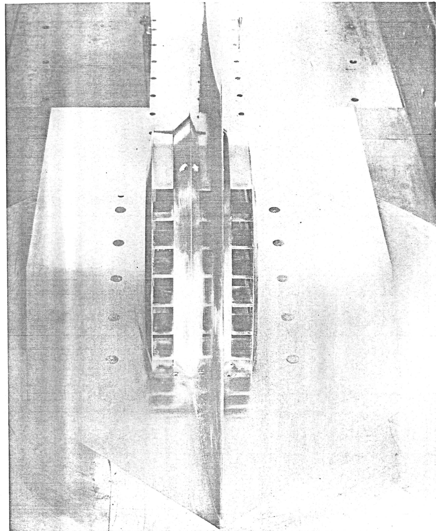
FIG. 15 2/25 SCALE AIR INTAKE MODEL
