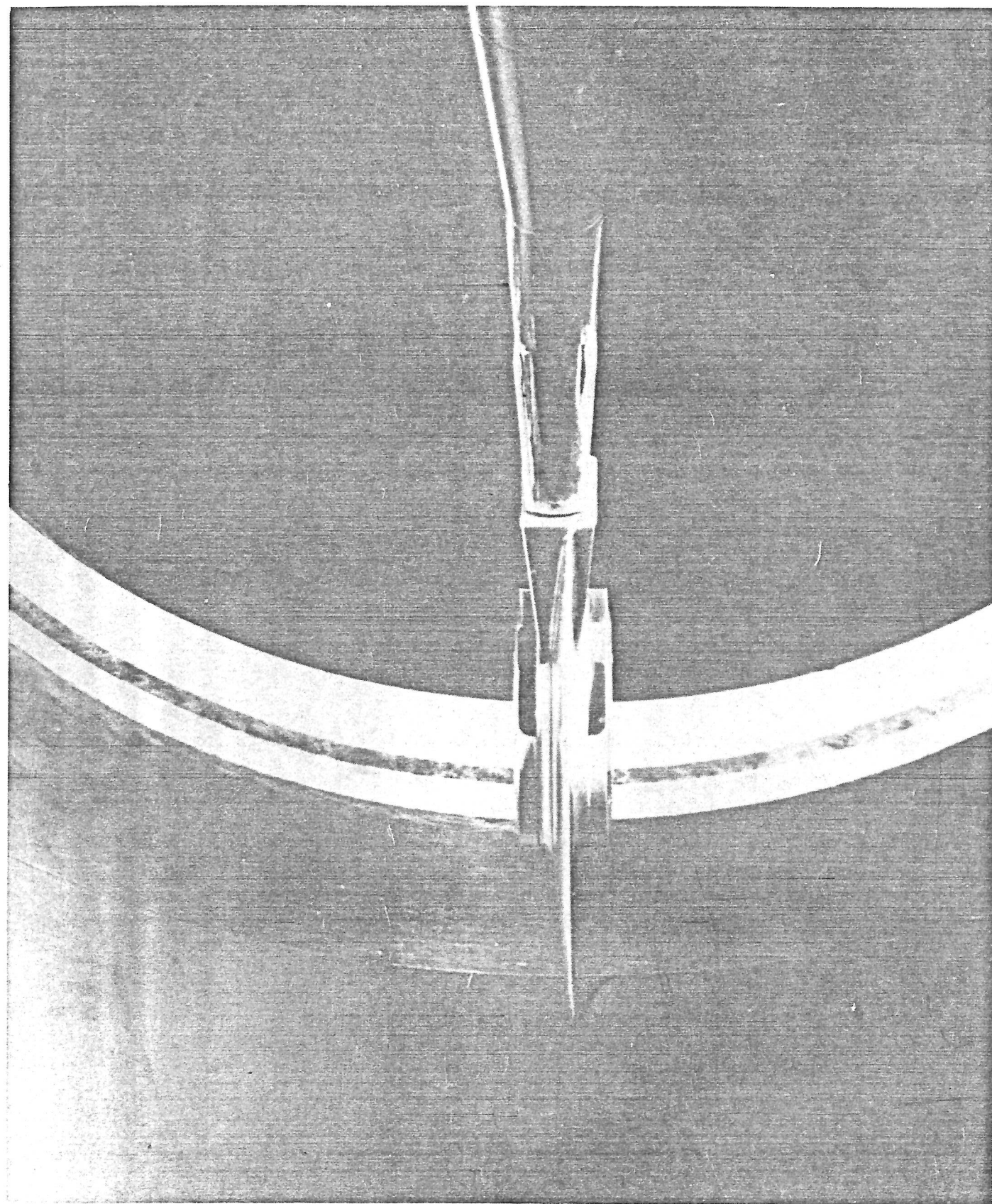
FIG. 18 1/40 SCALE STING MOUNTED MODEL
