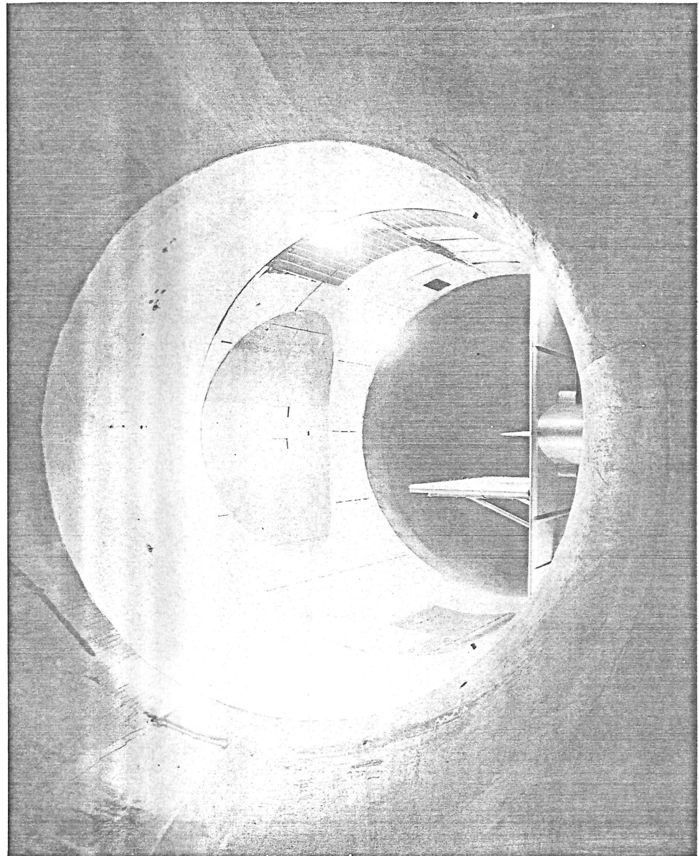
FIG. 12 1/6 SCALE MODEL IN TUNNEL
