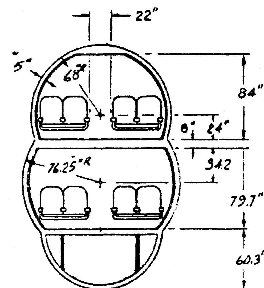
MAXIMUM SECTION
