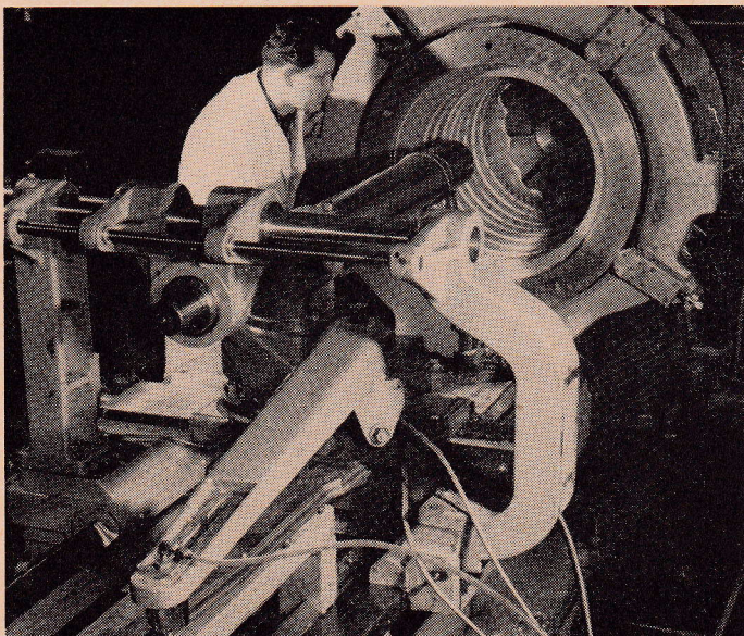
Fig. 5 — Boring compressor stator housing in Air-Gage tracer lathe.
