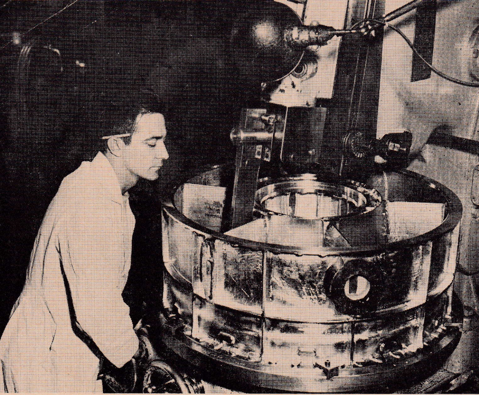
Left: Fig. 3—Compressor intake casting in vertical shaper.
