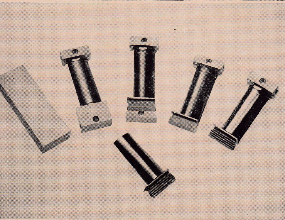
Fig. 17 — Stages in manufacture of turbine blades from bar stock.
