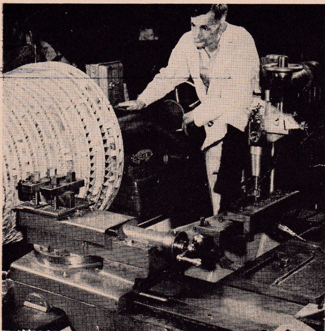
Fig. 10 — Turning blade tips in special Bertram lathe fitted with Turchan follower.
