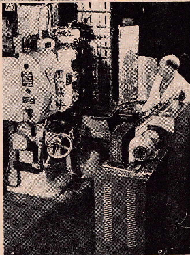
Fig. 18—Kellering three blades at one setting.
