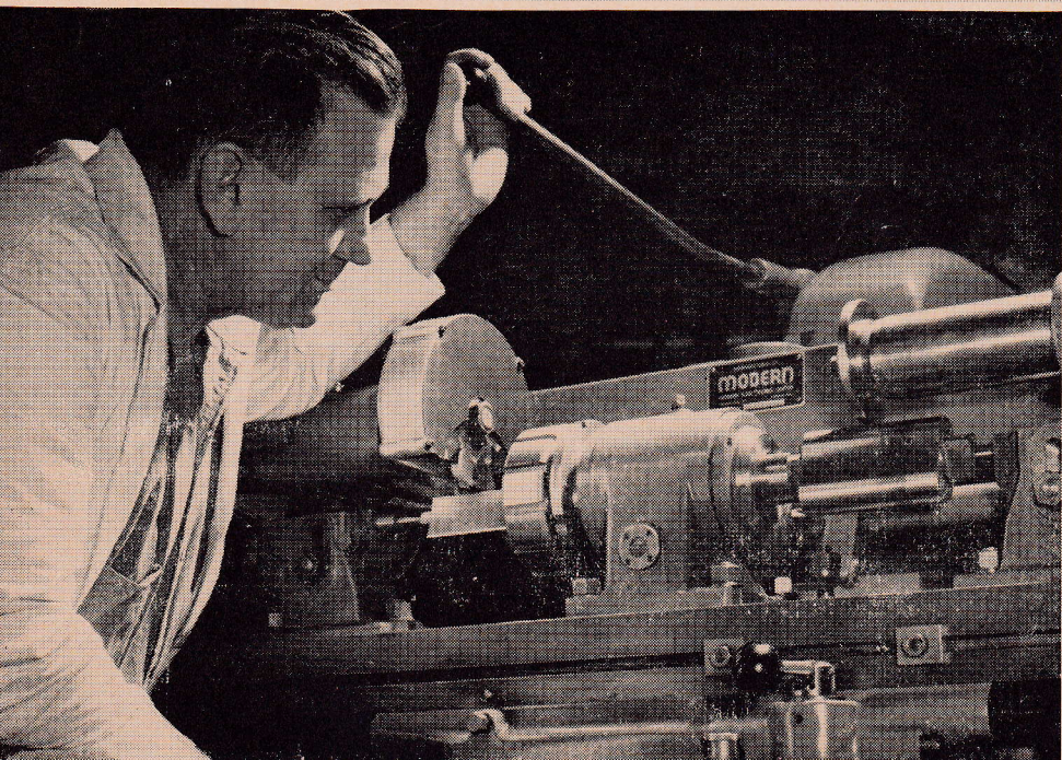
Fig. 19 — Special attachment in Modern milling machine for profiling blades.
