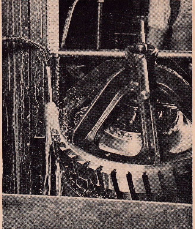
Fig. 8 — Broaching fir-tree slots in compressor disc.
