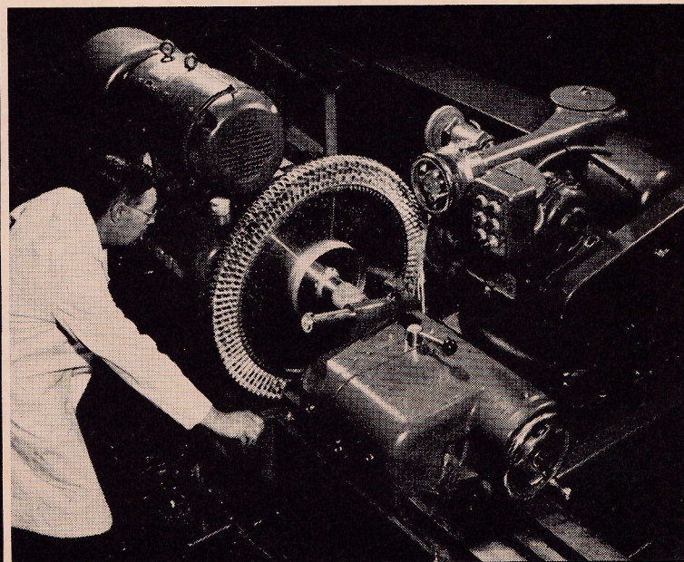
Fig. 13 — Grinding turbine rotor blade tips.
