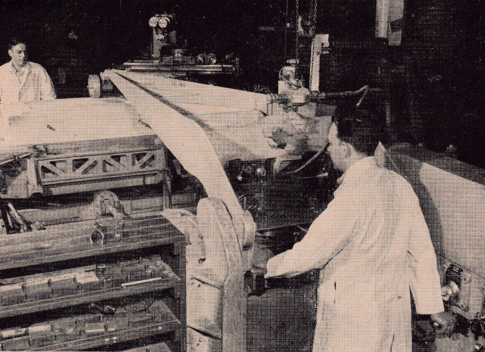
Fig. 16 — Pantograph duplicating machine (Avro Canada patented design) for grinding cavities in blade forging dies.
