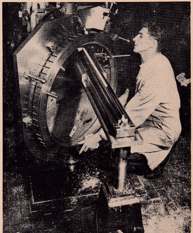
Fig. 7—Broaching internal slots for blades in compressor stator ring.
