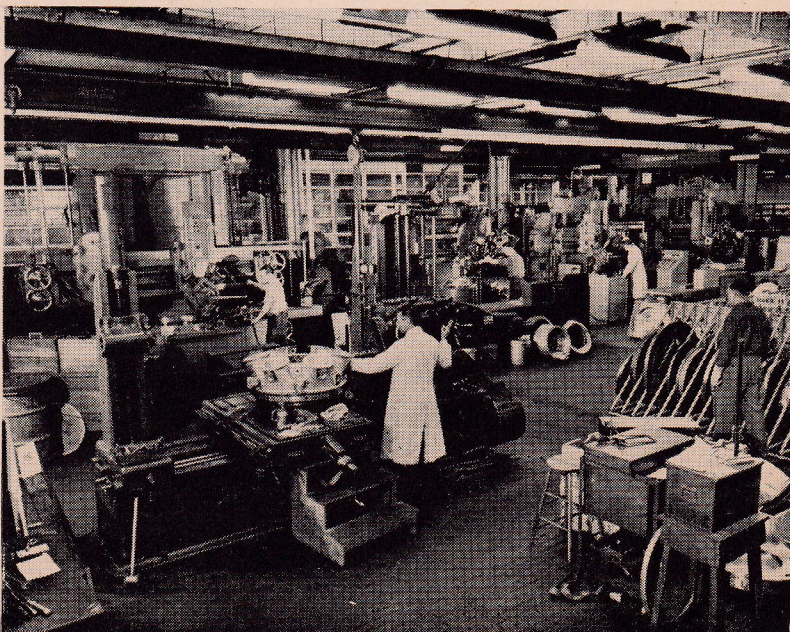
Fig. 11 — In foreground, diffuser casting in horizontal boring machine.
