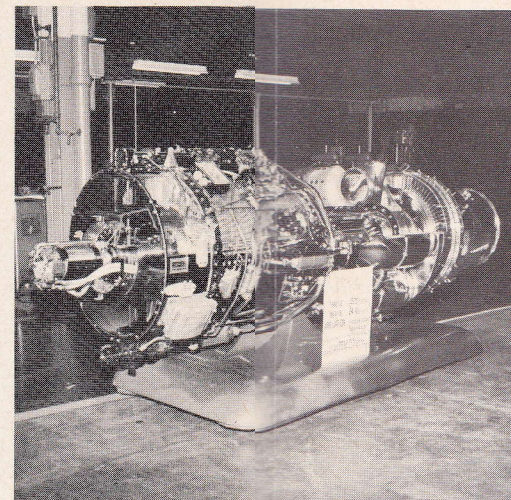
The gleaming Orenda 14 cutaway drew a lot of attention.
