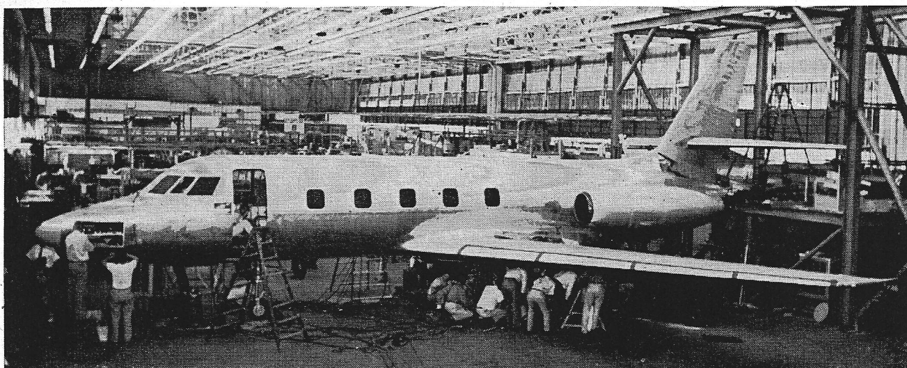
EXECUTIVE JET. This prototype of the ten passenger Lockheed jet transport was built in 30 weeks. It is a contender for the USAF fast multi-purpose jet requirement, but is also designed for commercial service. First flight was made during last month.
