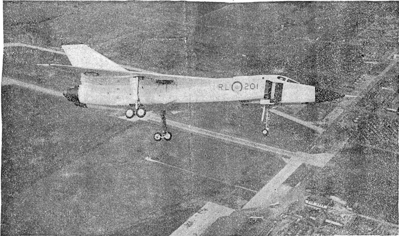
This air-to-air shot of the Arrow over Malton was taken from a chase plane that followed its test flight closely. The successful flight was the culmination of four and a half years of planning and work by engineers and technicians.
