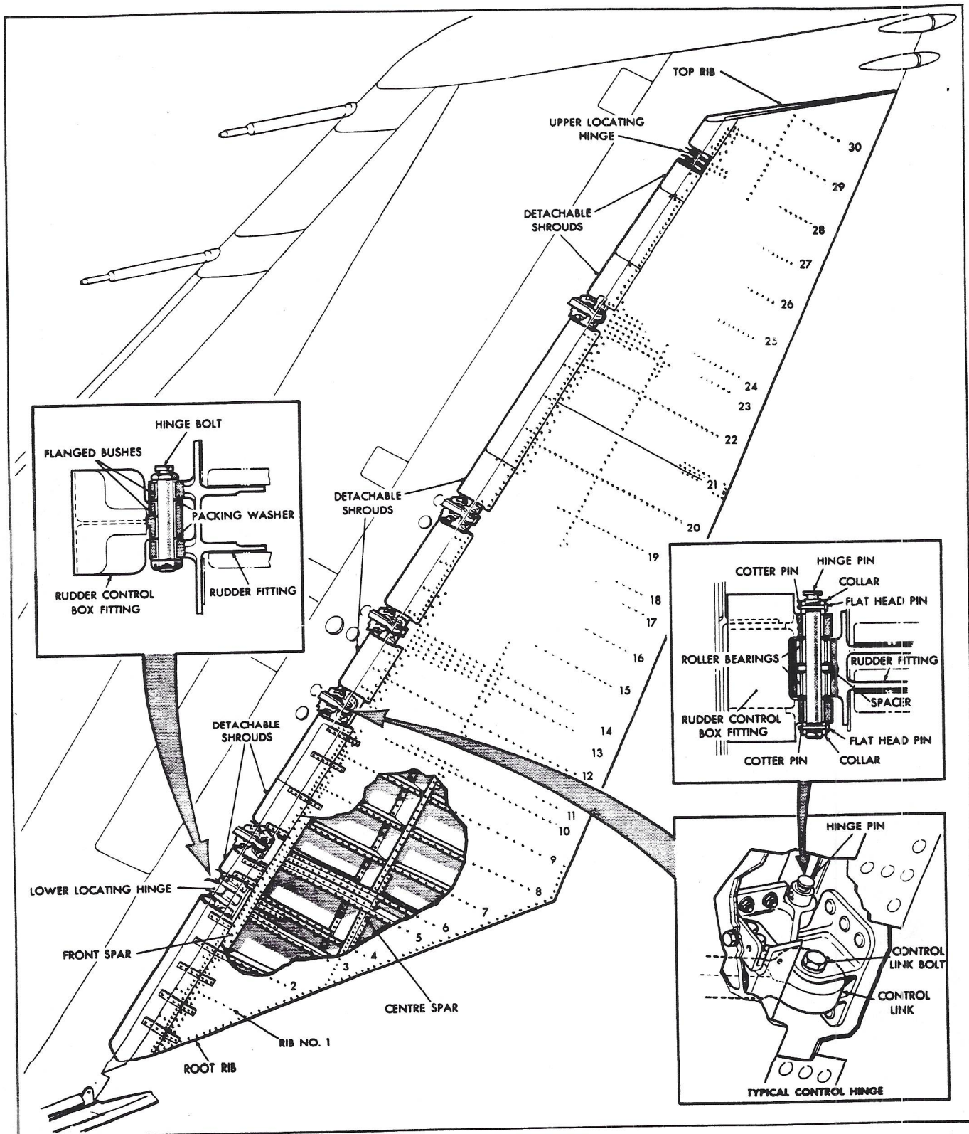
RUDDER STRUCTURE
