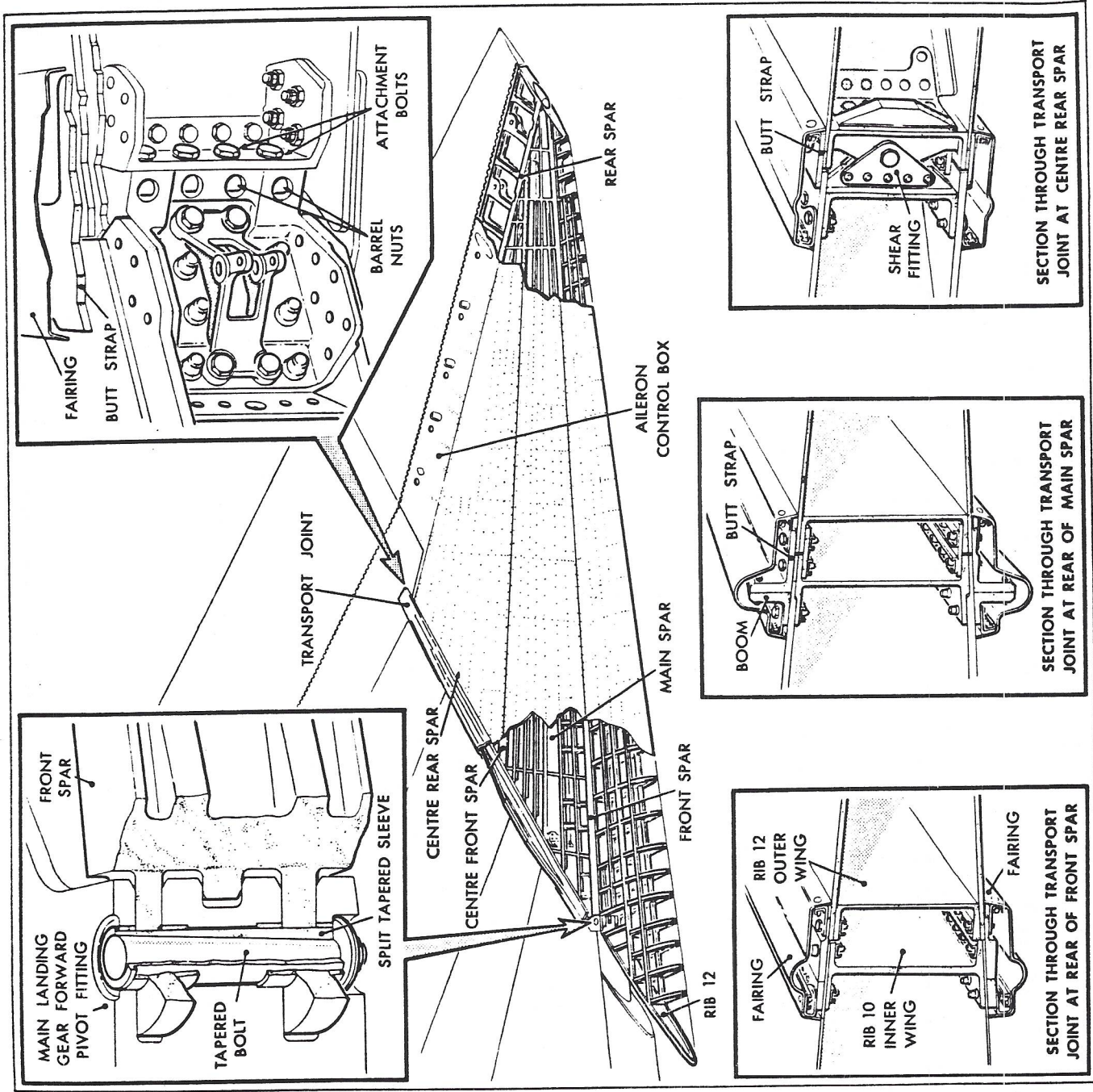
OUTER WING STRUCTURE
