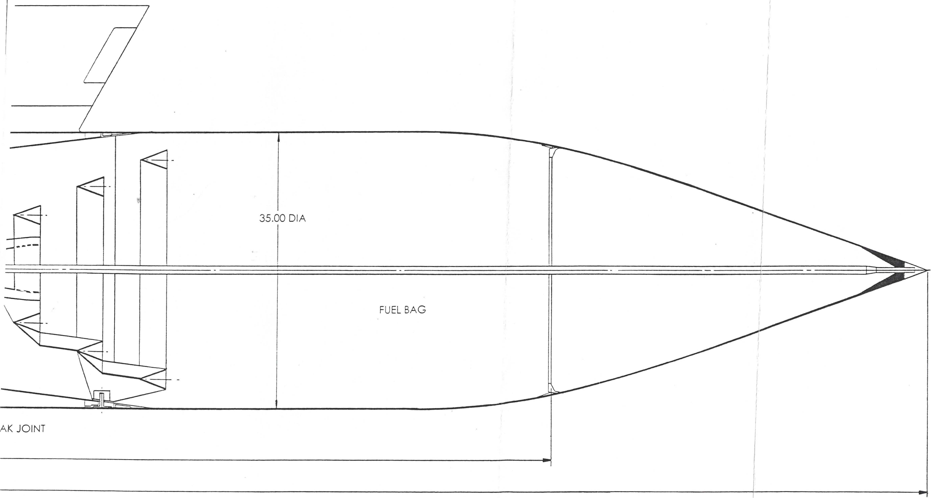
WING TANK RAMJET SCHEME. 35 DIA. (CURTISS-WRIGHT PROPOSAL)
