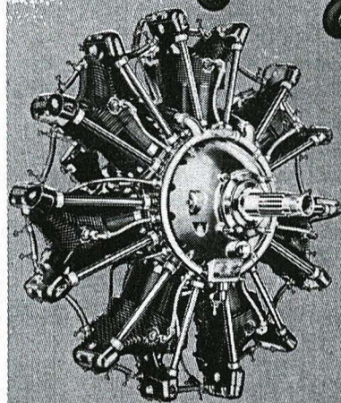
Jacobs Engine Model R-755 A
