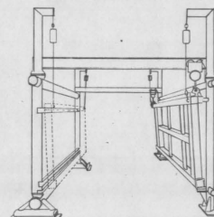
ELEVATOR MAIN ASSY JIG STAGE 1 & 2 LH LENGTH 15'-2" WIDTH 12'-1" HEIGHT 21'-2"
