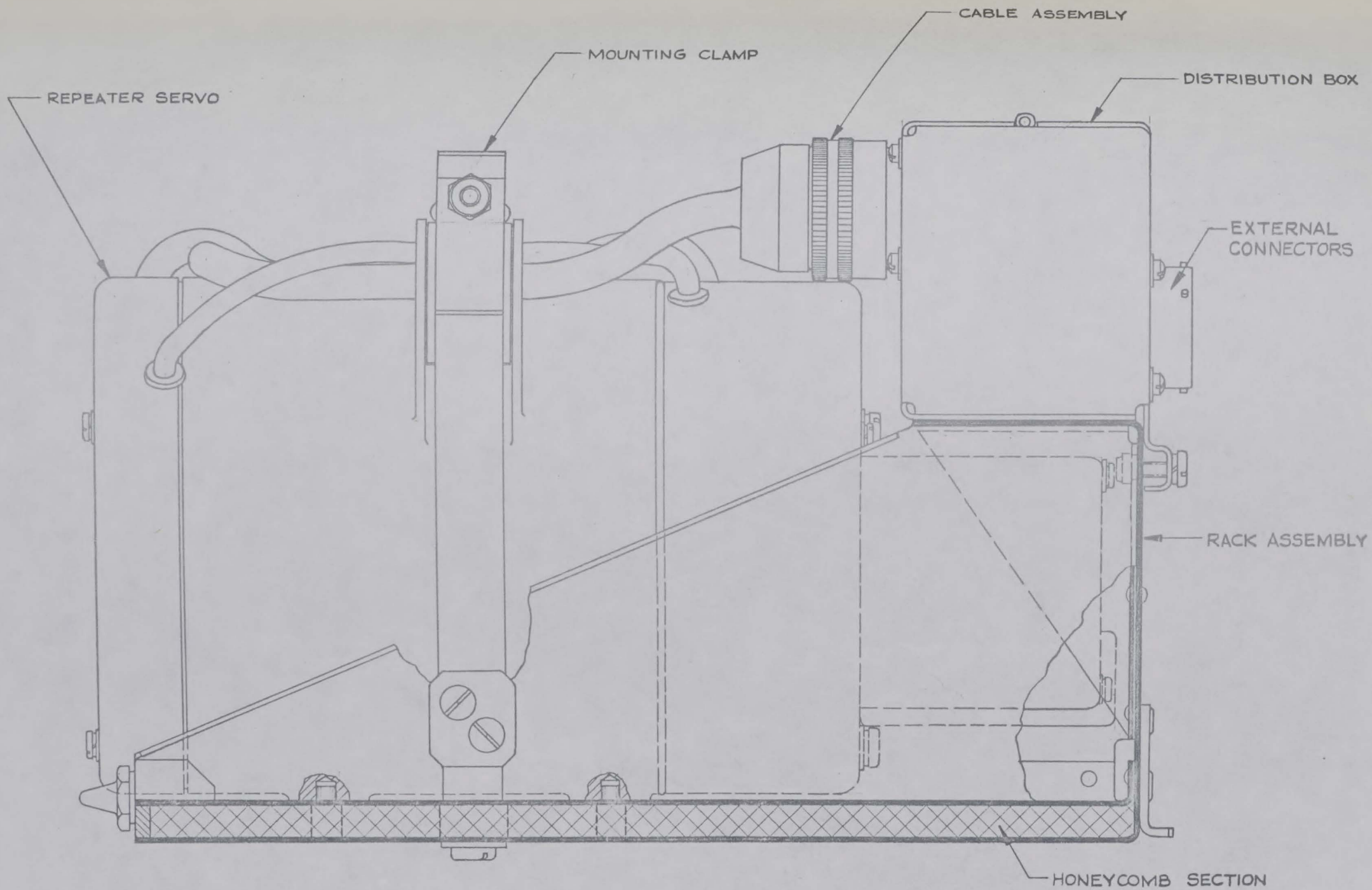
TYPICAL SECTION OF RACK - INDICATING EXPOSED HONEYCOMB, AND WITH A REPEATER SERVO MOUNTED
