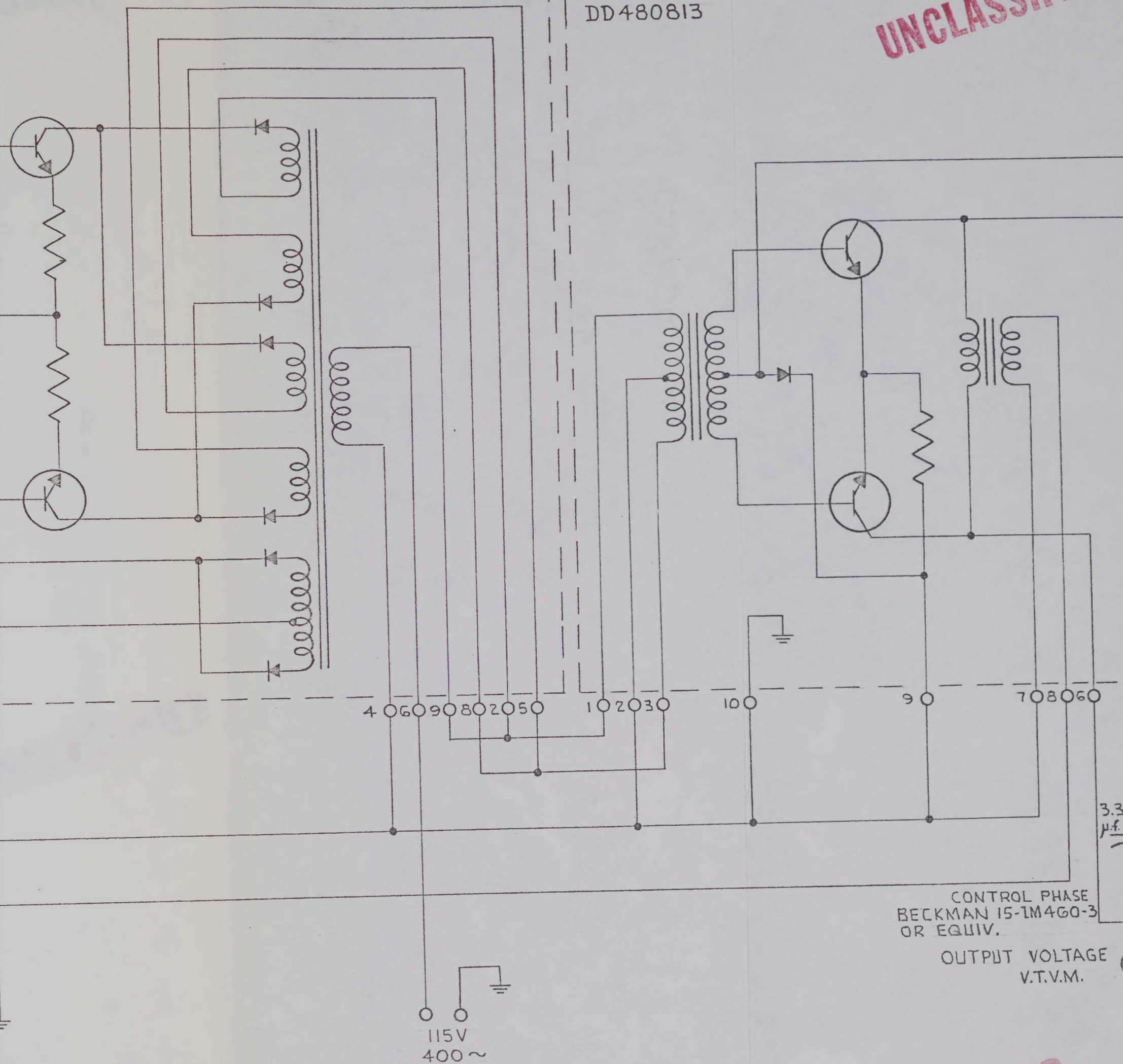
FIG 5.2.1 AMPLIFIER SYSTEM TEST CONNECTIONS
