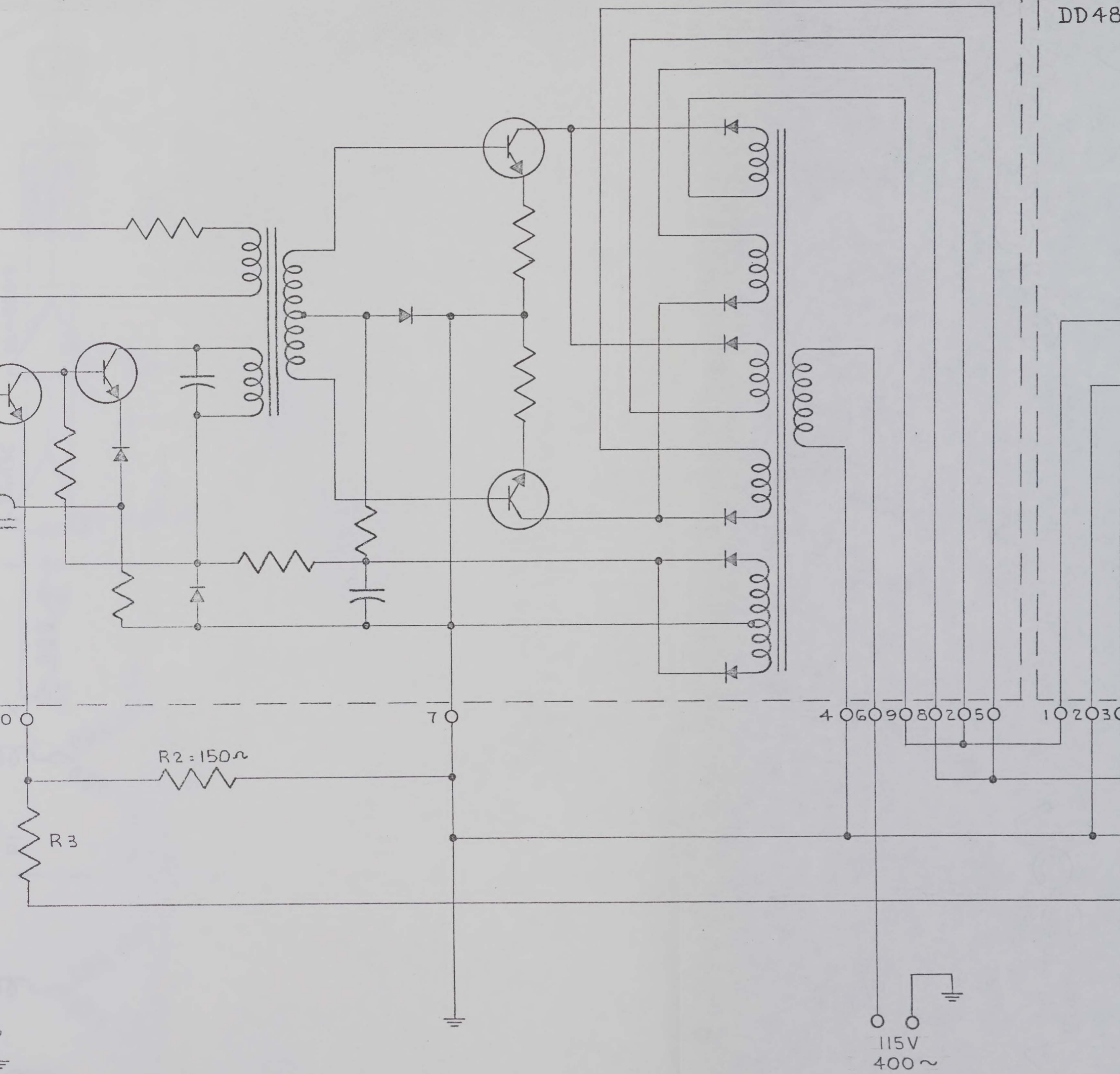
FIG 5.2.1 AMPLIFIER SYSTEM TEST CONNECTION
