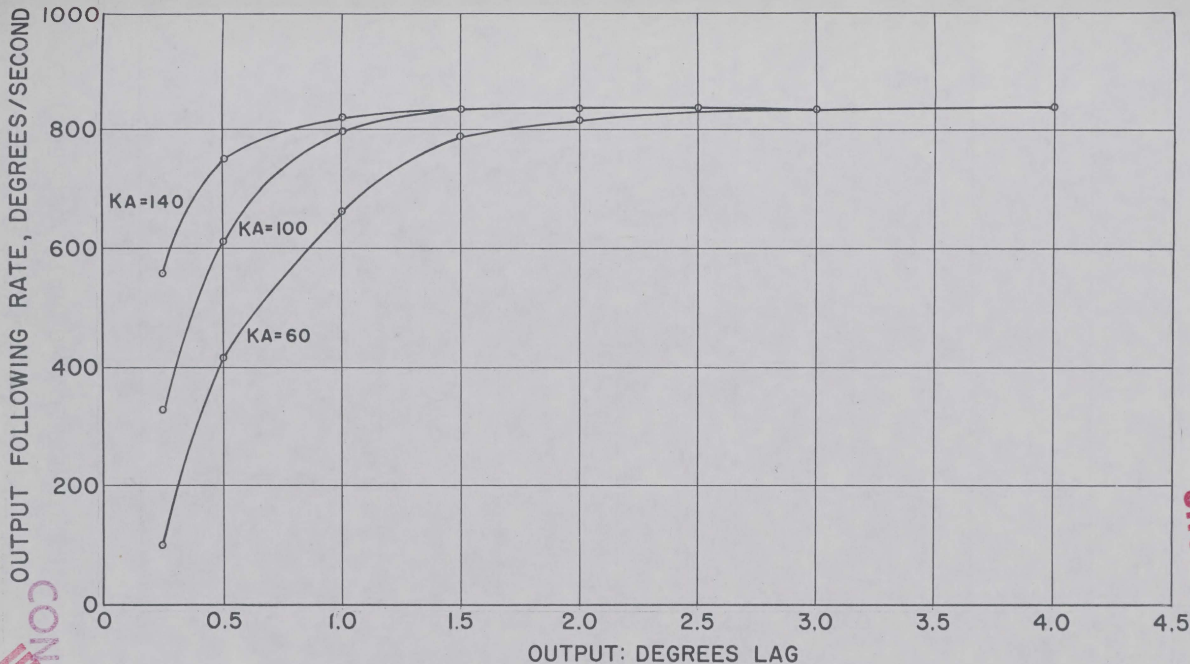
GRAPH #13 FOLLOWING RATE OF D-DG600IB-3 #L-2 ELEVATION AXIS MOTOR PT-0 15IM460-3 AMPLIFIER SYSTEM GAINS AS INDICATED
