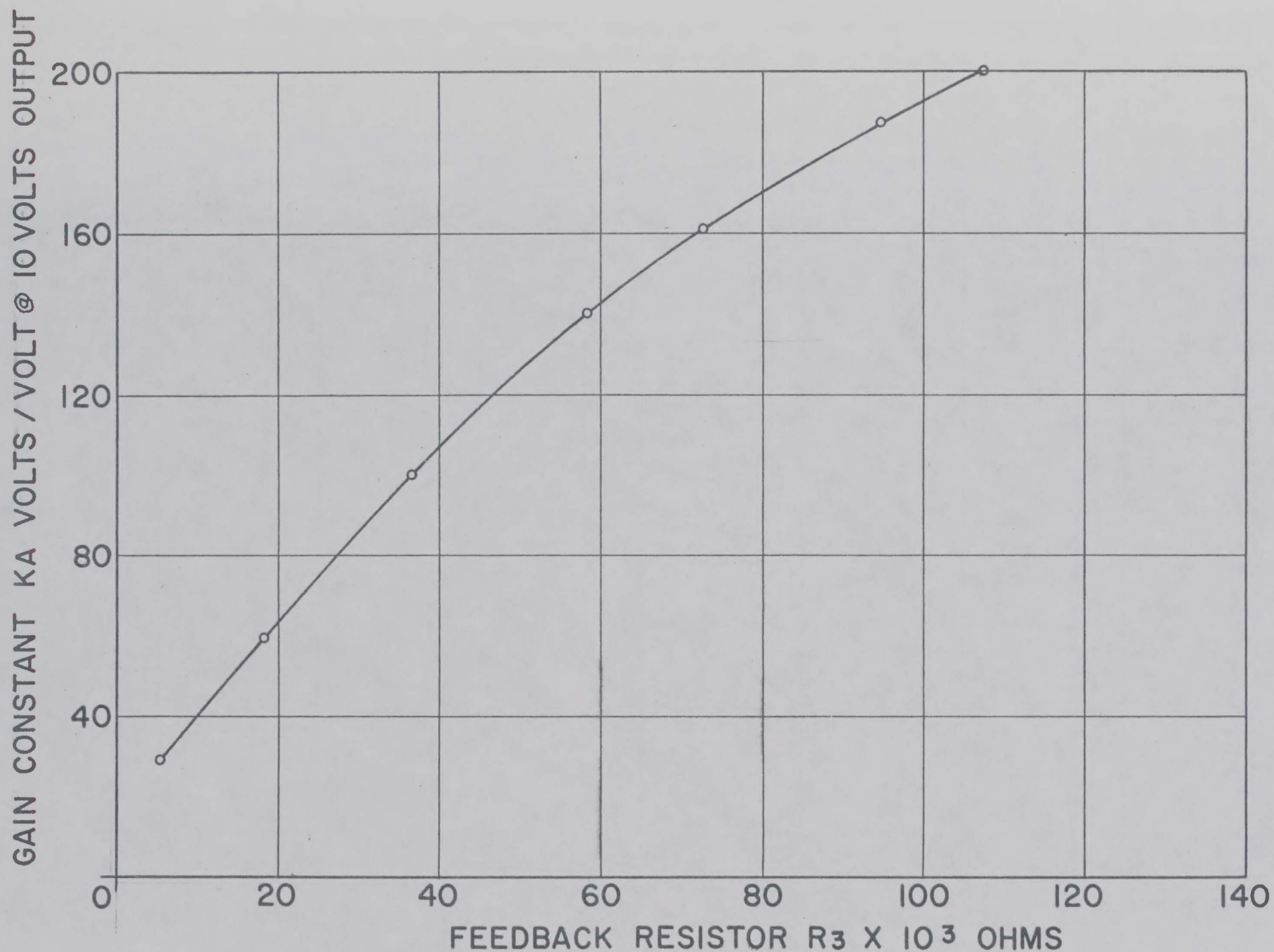
GRAPH # 12 GAIN VS. FEEDBACK RESISTOR R_3 ELEVATION AXIS D-DG6001B-3, L-2 SERIES LOAD MOTOR: BECKMAN 151M460-3 #PT-0 R_2 = 150 OHMS
