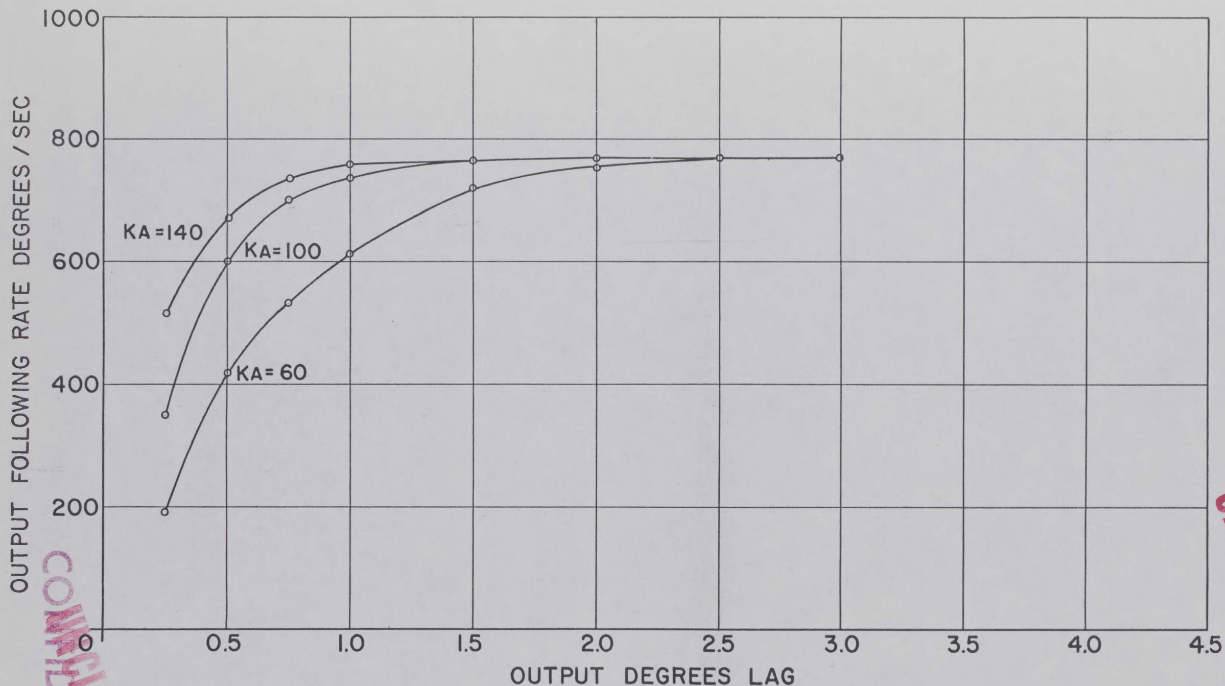
GRAPH # 26 FOLLOWING RATE OF DG6000-G BREADBOARD MOTOR: 15-IM460-3 #PT-0, f_2=643 AMPLIFIER SYSTEM GAINS (KA) AS INDICATED
