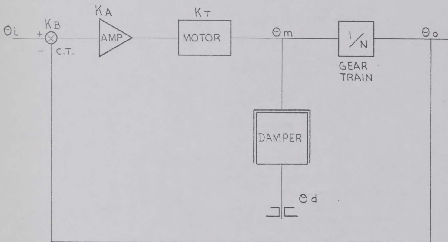
SERVO - LOOP USING INERTIAL DAMPED MOTOR
