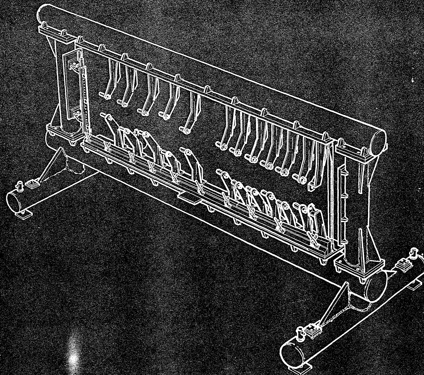
COCKPIT FLOOR ASSY JIG 7-1052-395 A-1 L.H. 7-1052-396 A-1 R.H.
