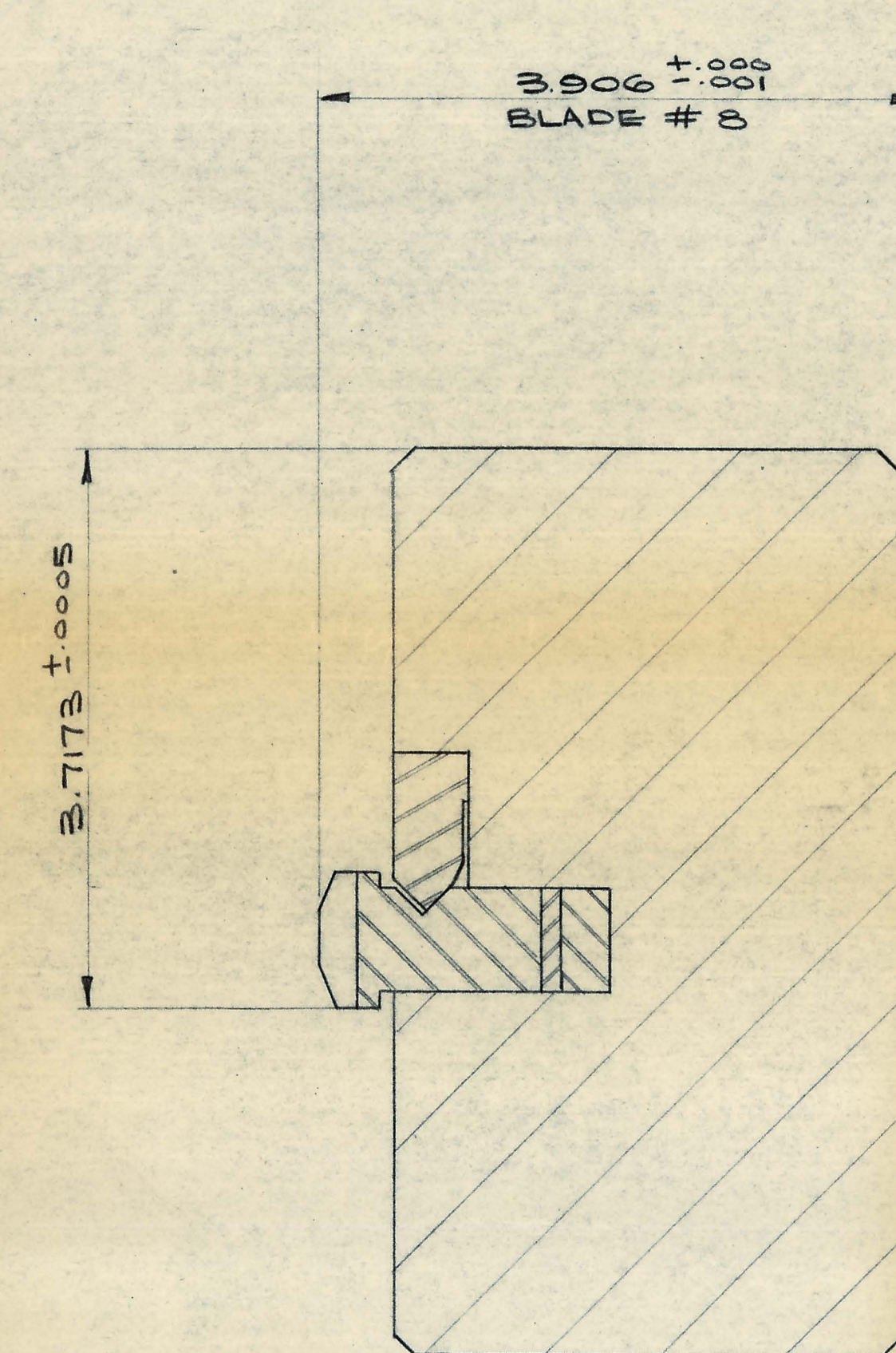
SECTION E-E
