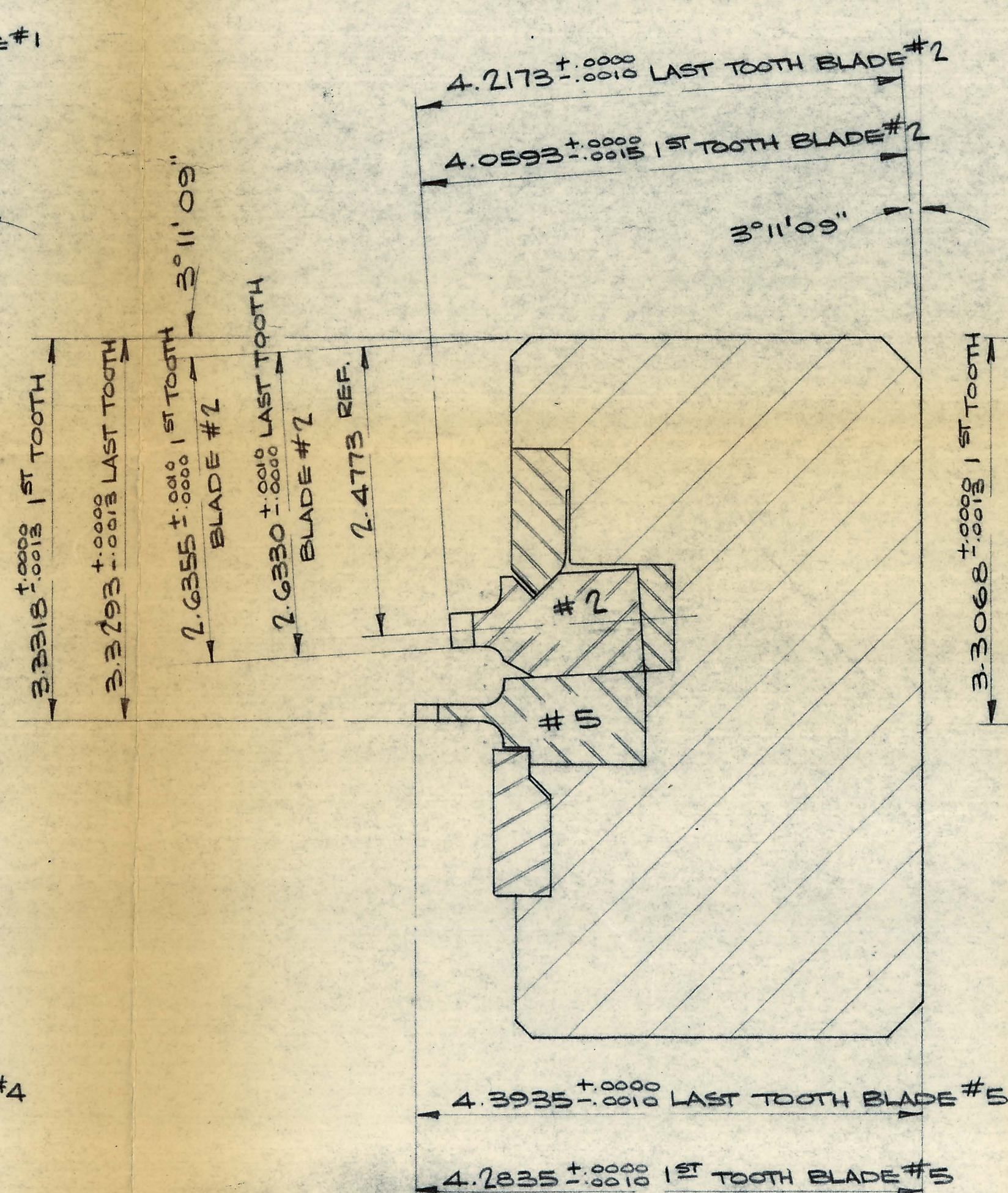
SECTION B-B
