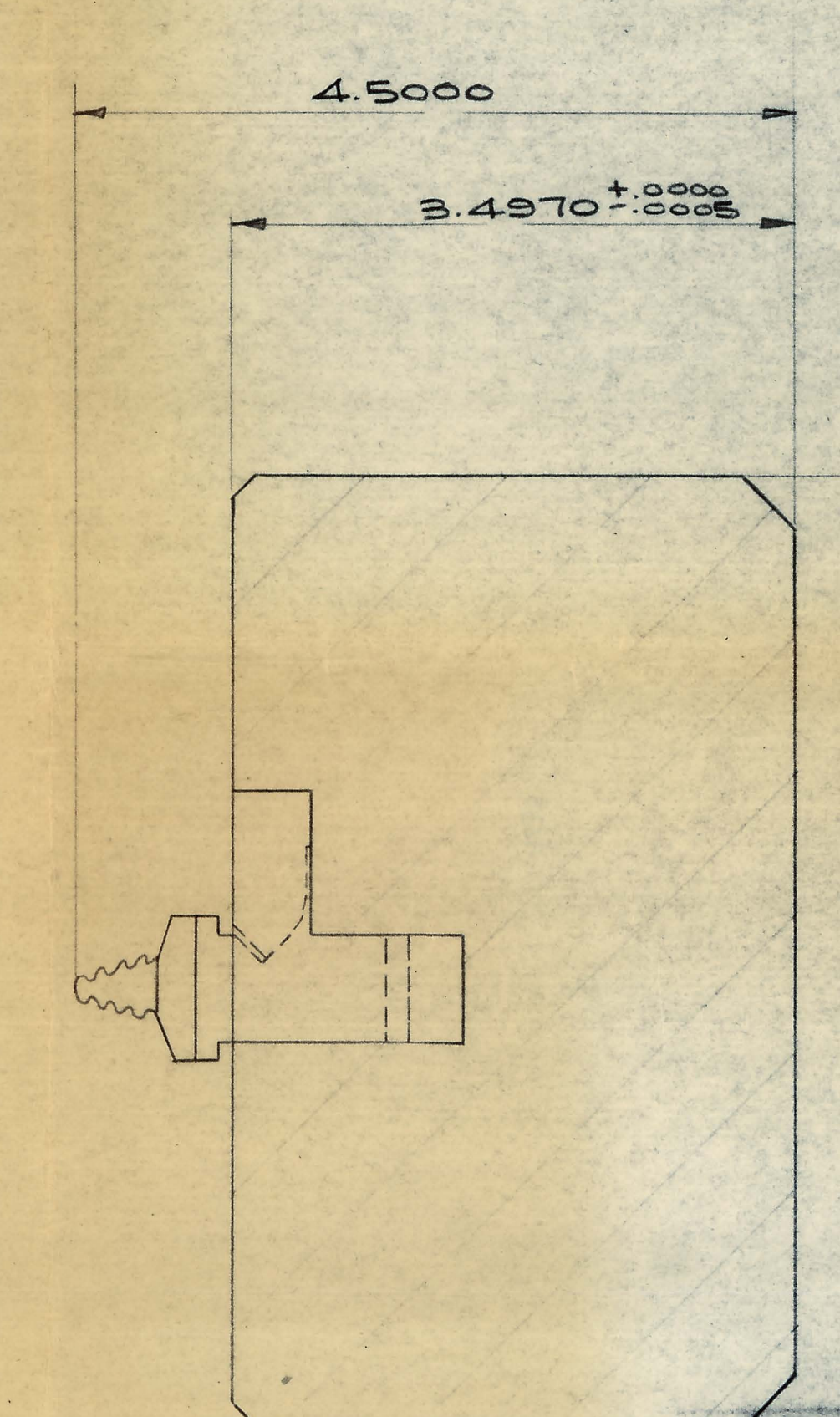
VIEW IN DIRECTION OF ARROW G
