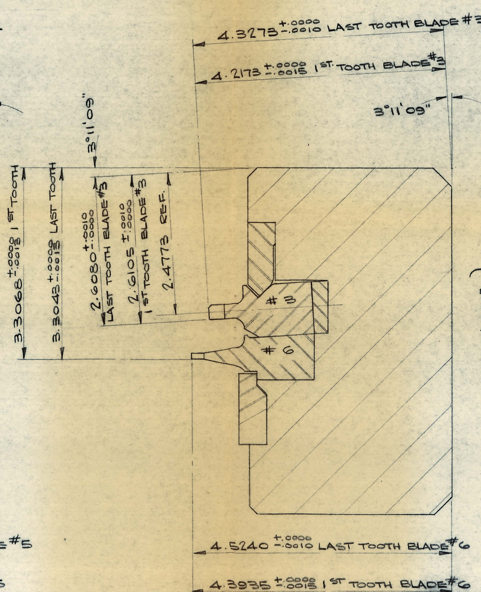
SECTION C-C
