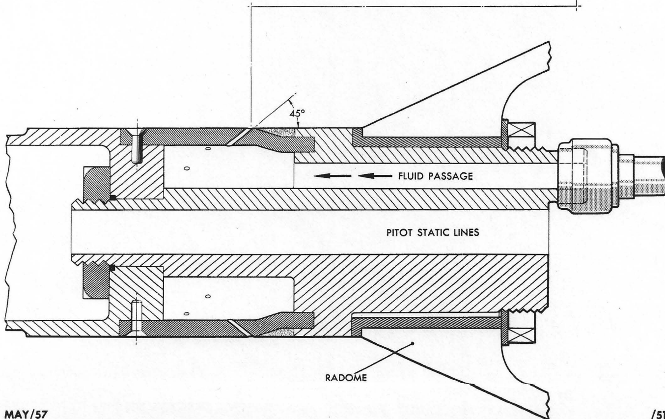
FIG. 8 RADOME FLUID DISTRIBUTOR
