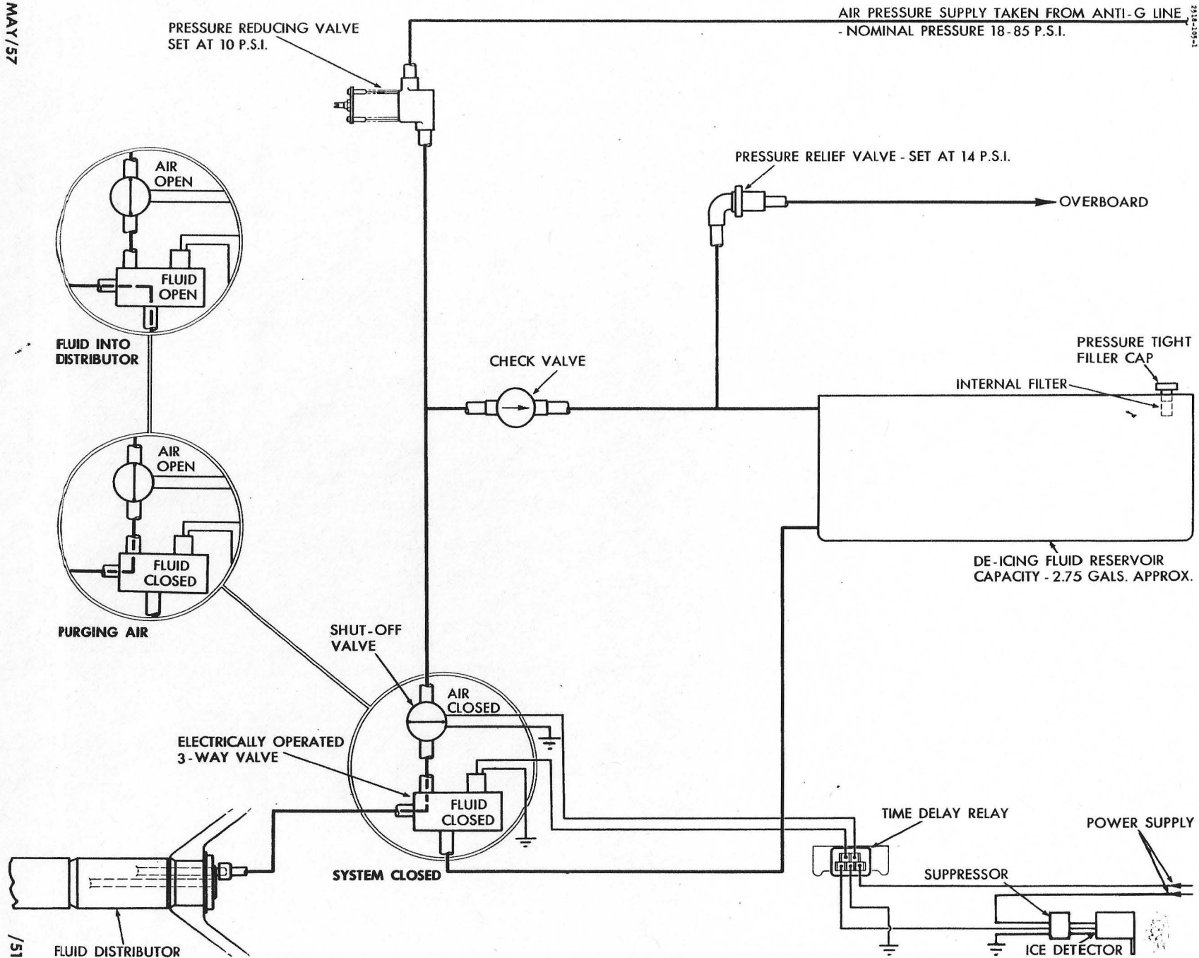
FIG. 7 RADOME DE-ICING SYSTEM
