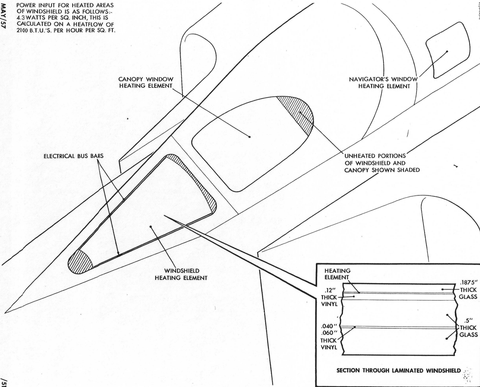
FIG. 1 WINDSHIELD AND CANOPY DE-ICING
