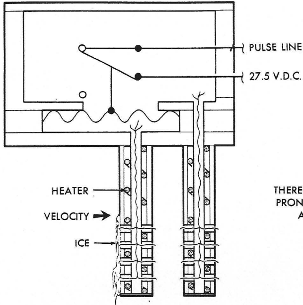
VIEW WITH ONE PRONG MOVED OUT FROM CORRECT POSITION TO SHOW FUNCTION OF SWITCH
