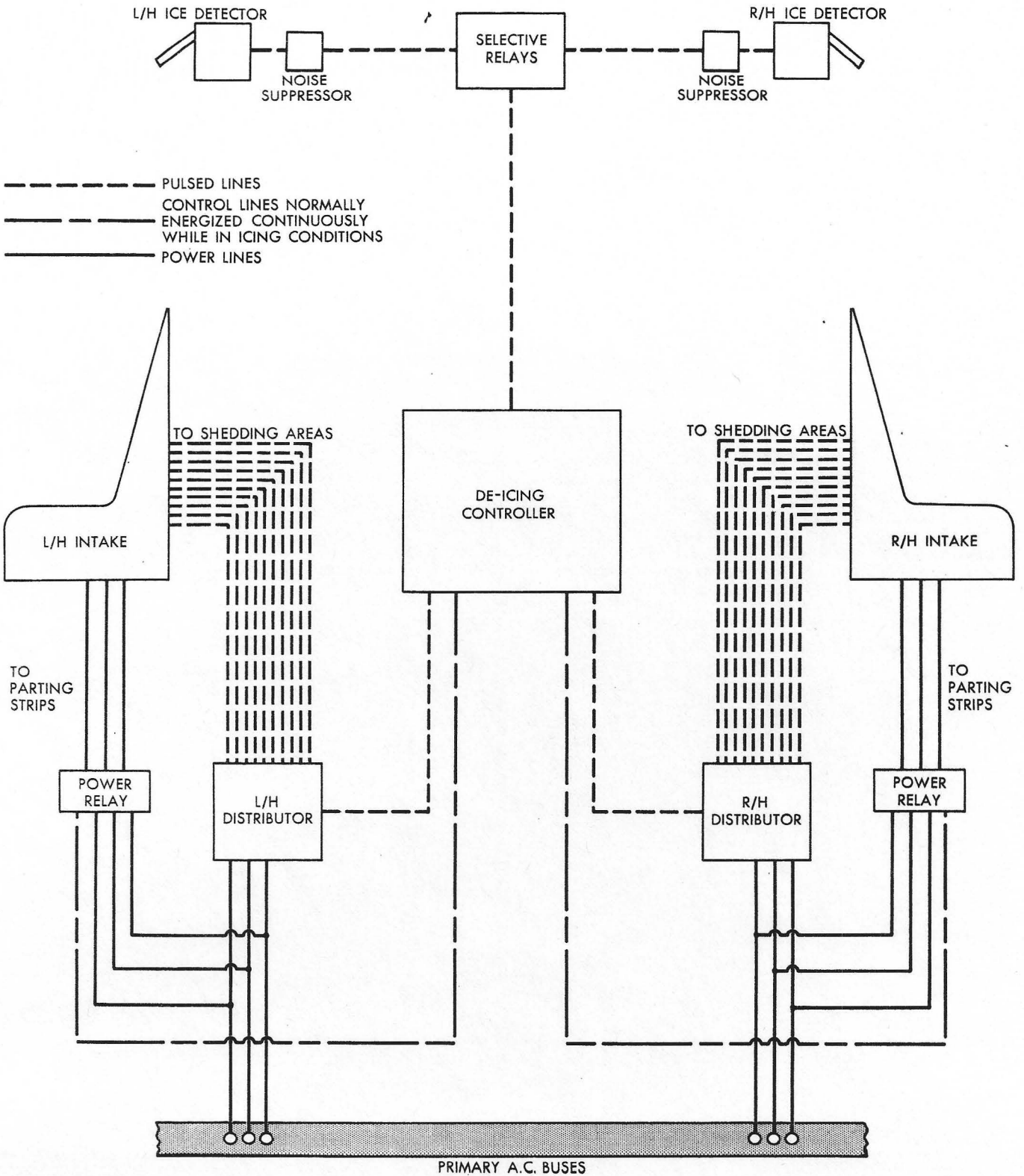
FIG. 3 BLOCK DIAGRAM OF INTAKE DE-ICING
