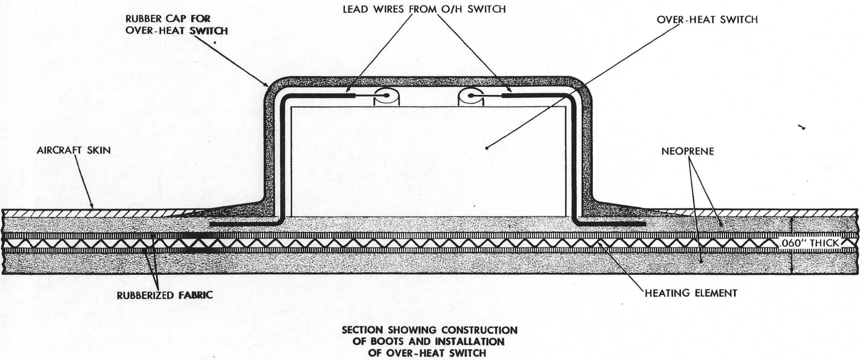
FIG. 6 BOOT CONSTRUCTION AND INSTALLATION OF OVER-HEAT SWITCH
