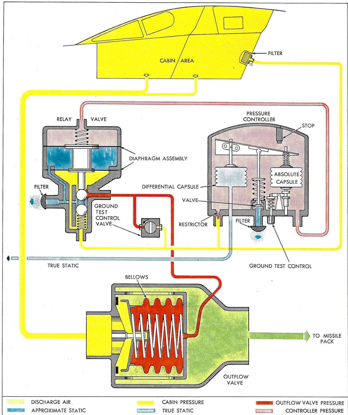
CABIN PRESSURIZATION CONTROLS - SCHEMATIC
