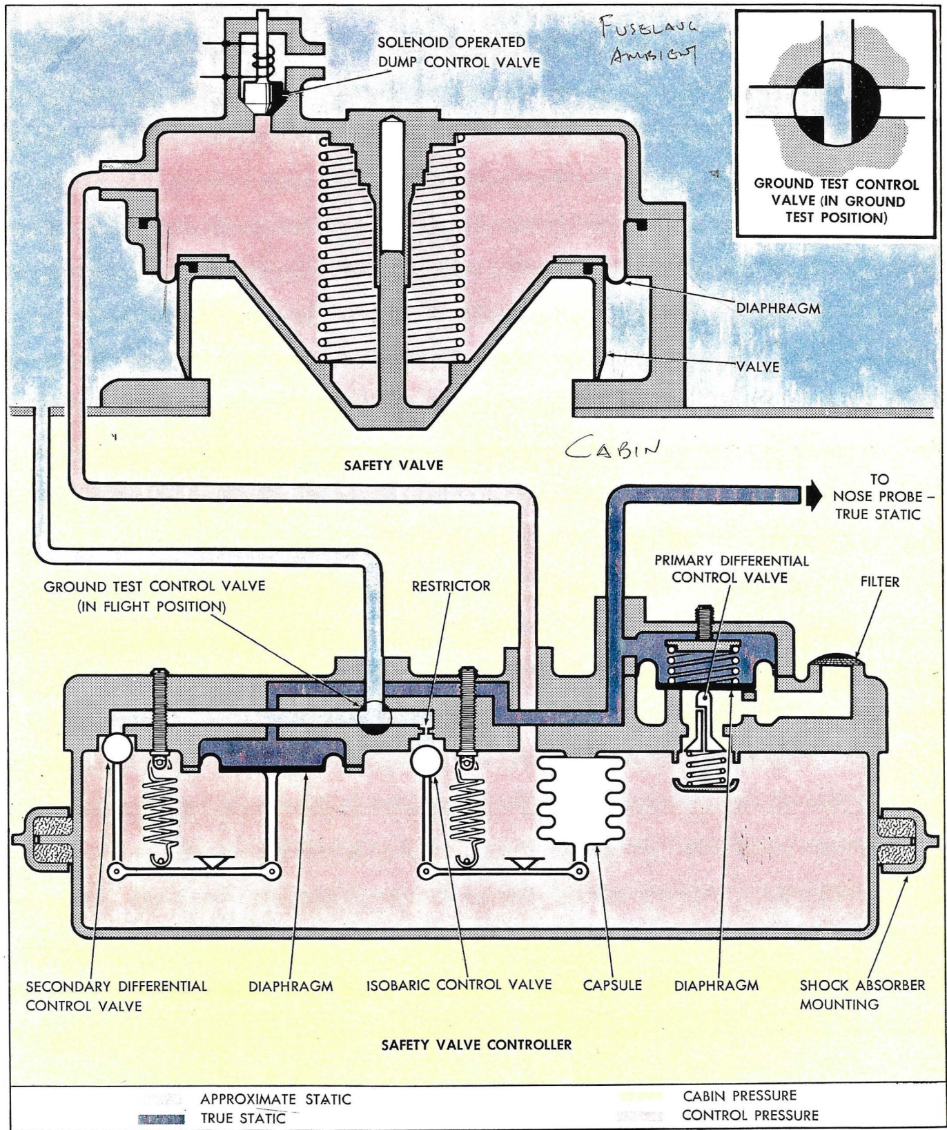
CABIN PRESSURE SAFETY VALVE - SCHEMATIC
