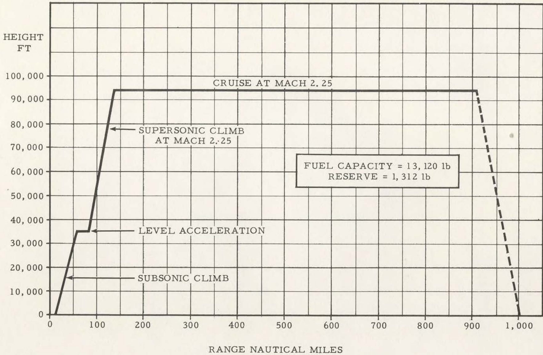
FIG. 11 PROJECT 1794 STILL AIR RANGE
