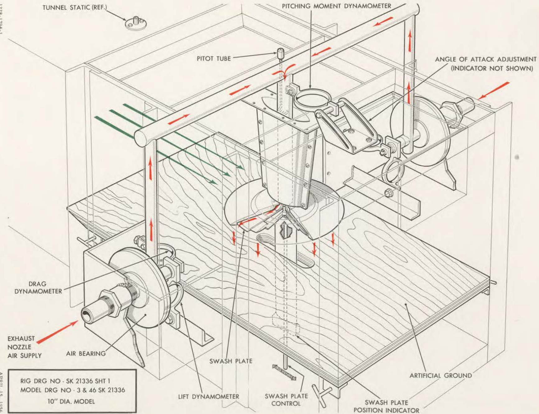
FIG. 31 AIR CUSHION EFFECTS MODEL NO. 1/1/1
