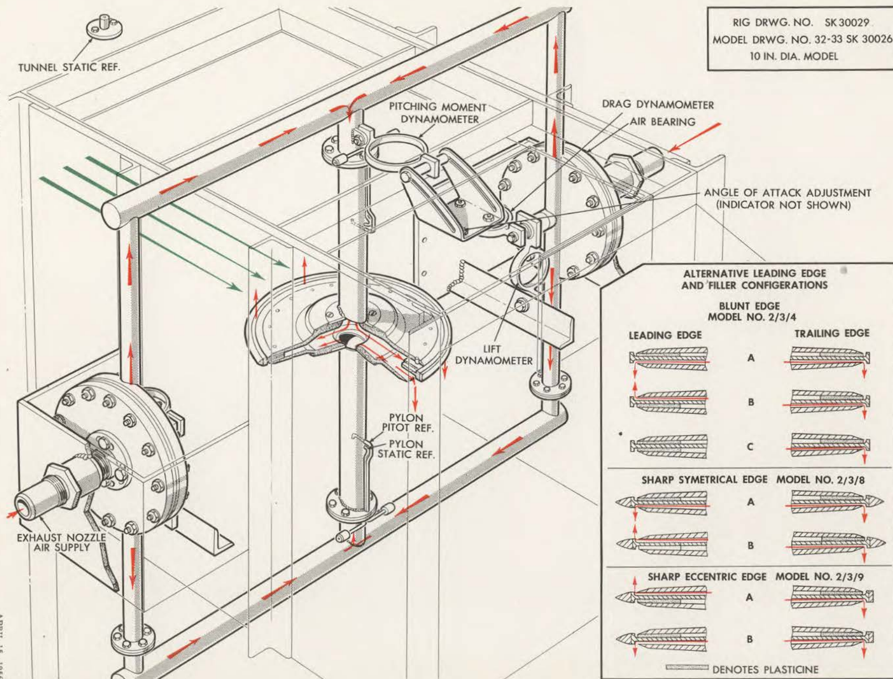
FIG. 32 STABILITY AND CONTROL MODELS NO. 2/3/4, 2/3/8 AND 2/3/9
