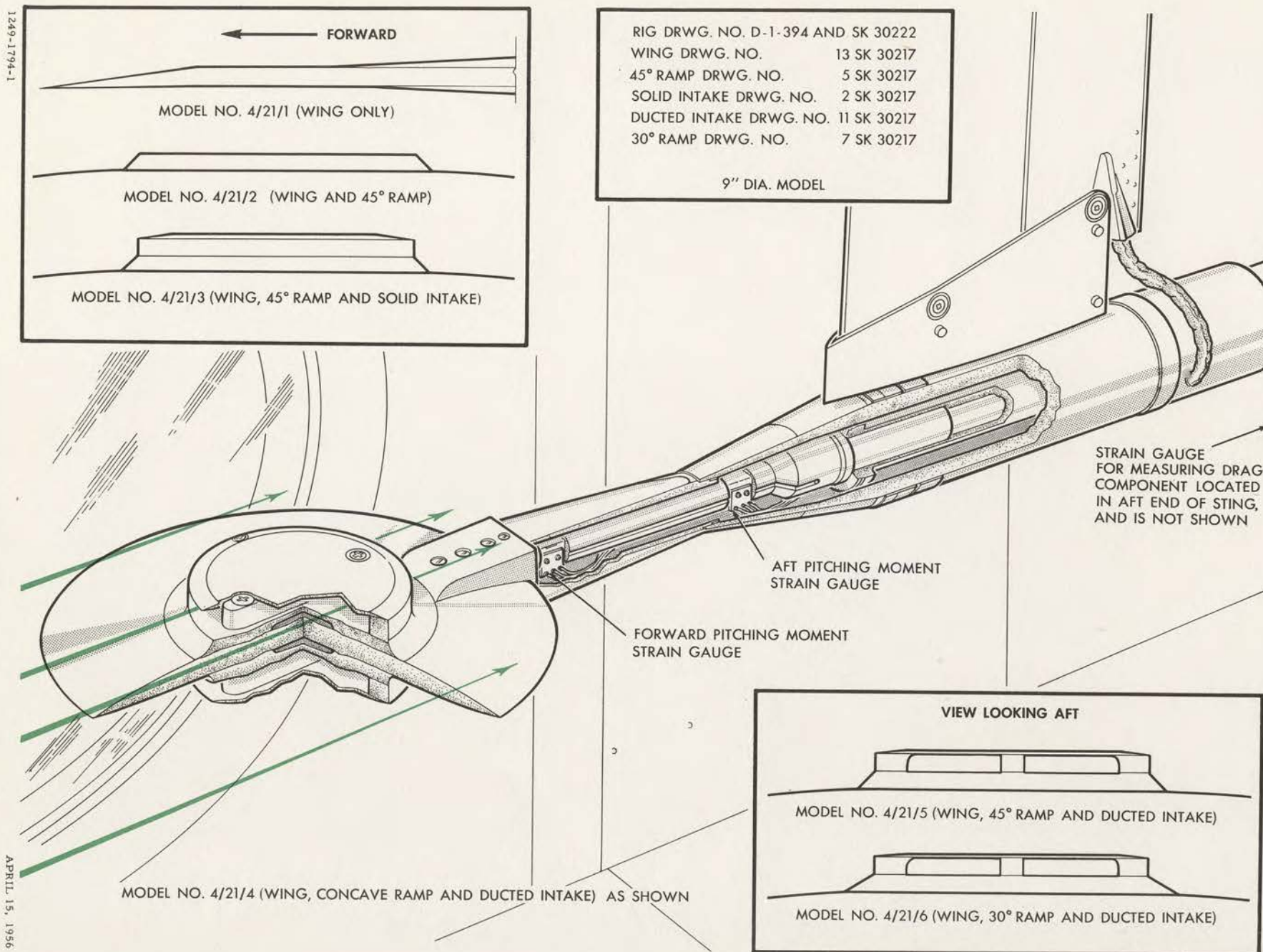
FIG. 19 PERFORMANCE MODEL NO. 4/21
