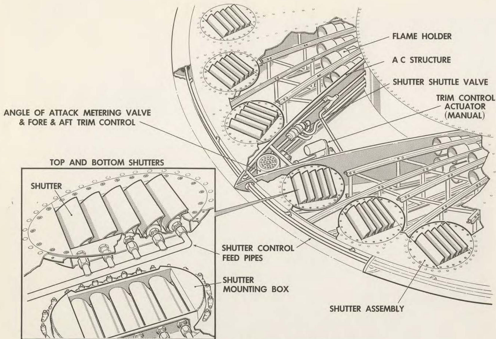
CUTAWAY OF CONTROL SHUTTERS FIG. 7
