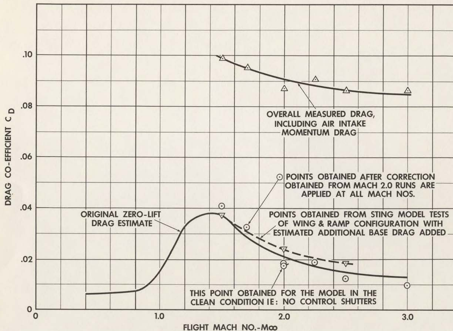
PROJECT 1794 ZERO LIFT DRAG AND MACH NO. FIG. 26
