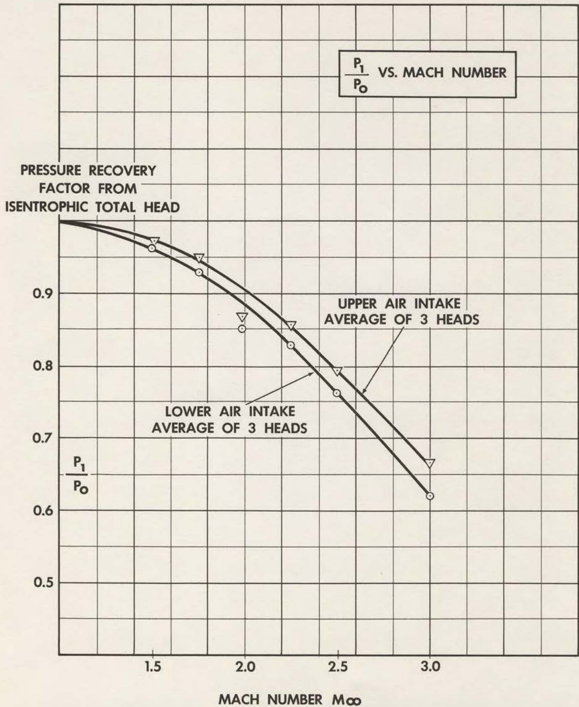
PROJECT 1794 INTAKE PRESSURE RECOVERY FIG. 28
