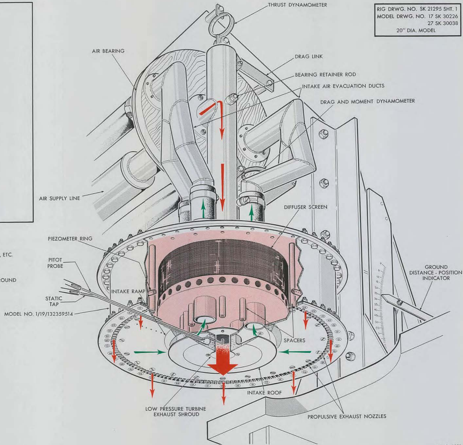
AIR CUSHION EFFECTS MODEL NUMBER 1/9 (CONTINUED)
