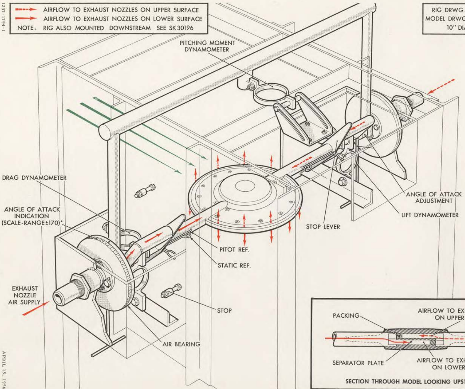
FIG. 34 STABILITY AND CONTROL MODEL NO. 2/4/1
