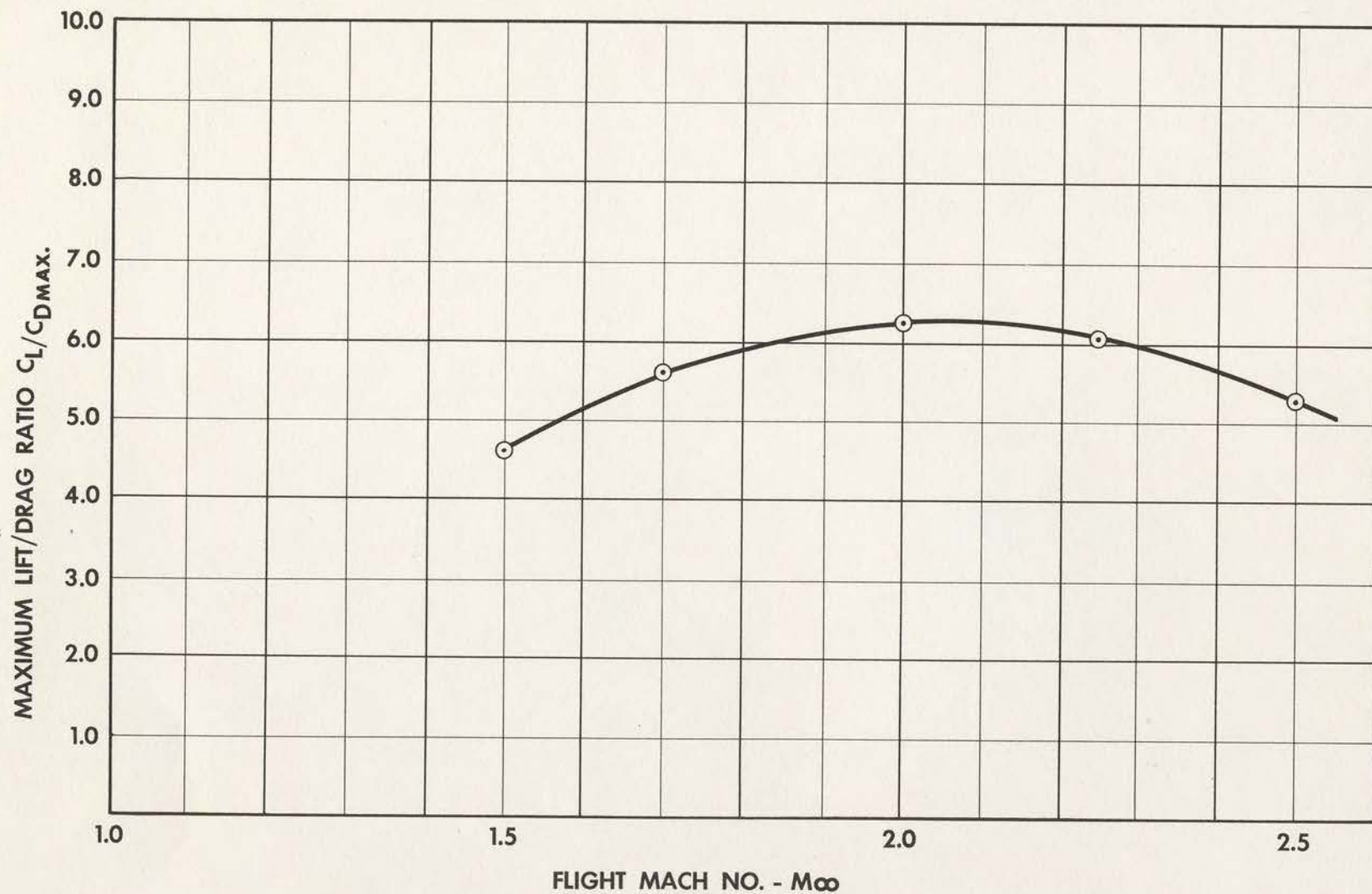
PROJECT 1794 VARIATION OF MAXIMUM LIFT / DRAG RATIO WITH MACH NUMBER FIG. 27
