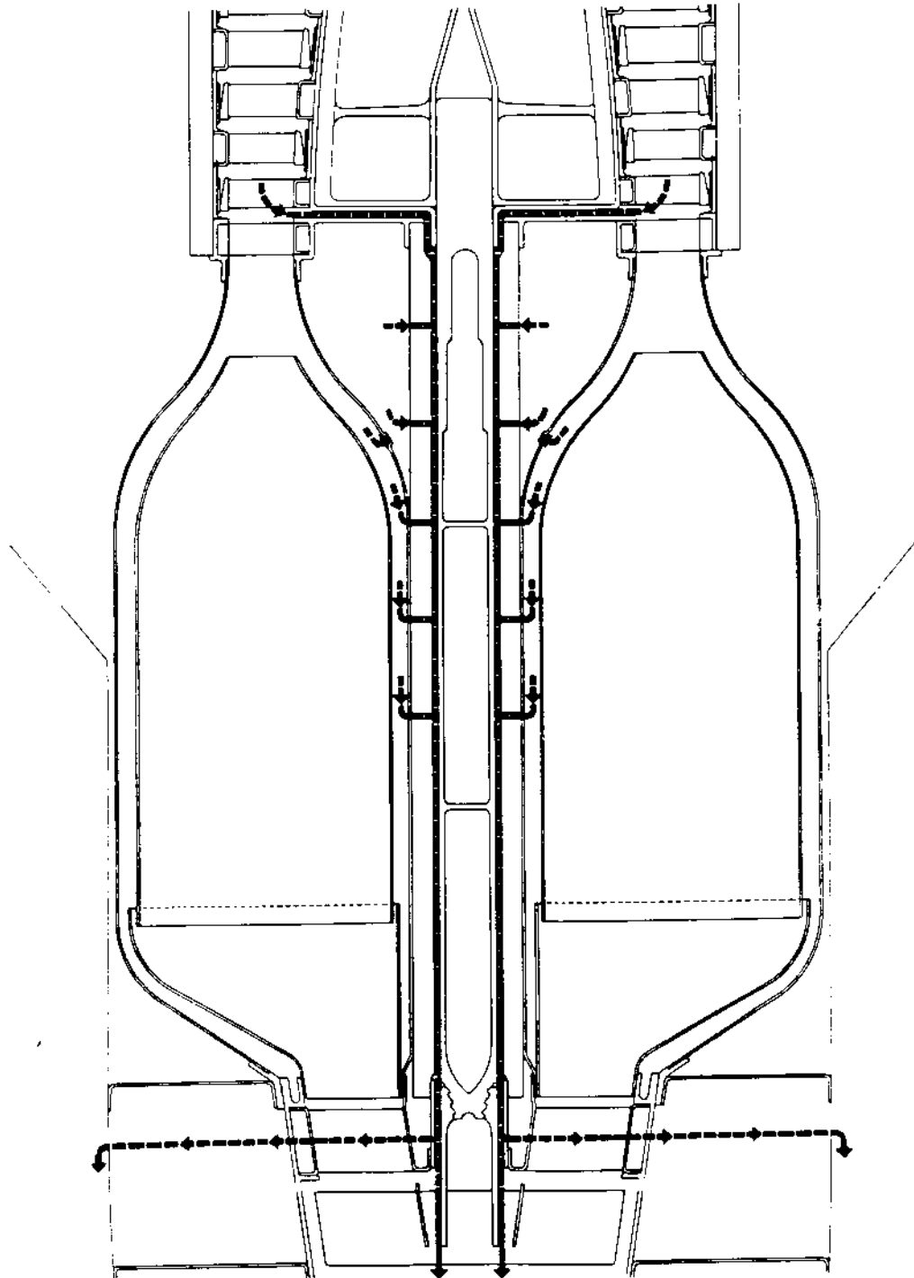
Fig. 12 Cross-Section Showing Bearing Airflow
