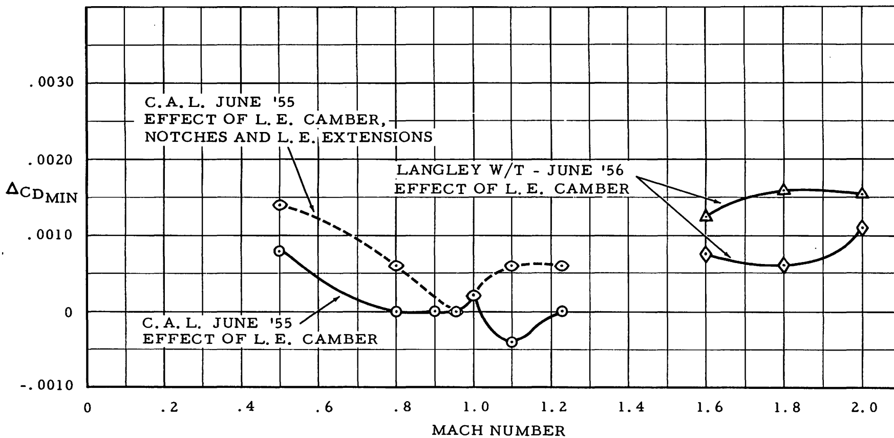
FIG. 4 CF-105 INCREASE IN C_{D\text{MIN}} DUE TO WING PLANFORM MODIFICATIONS
