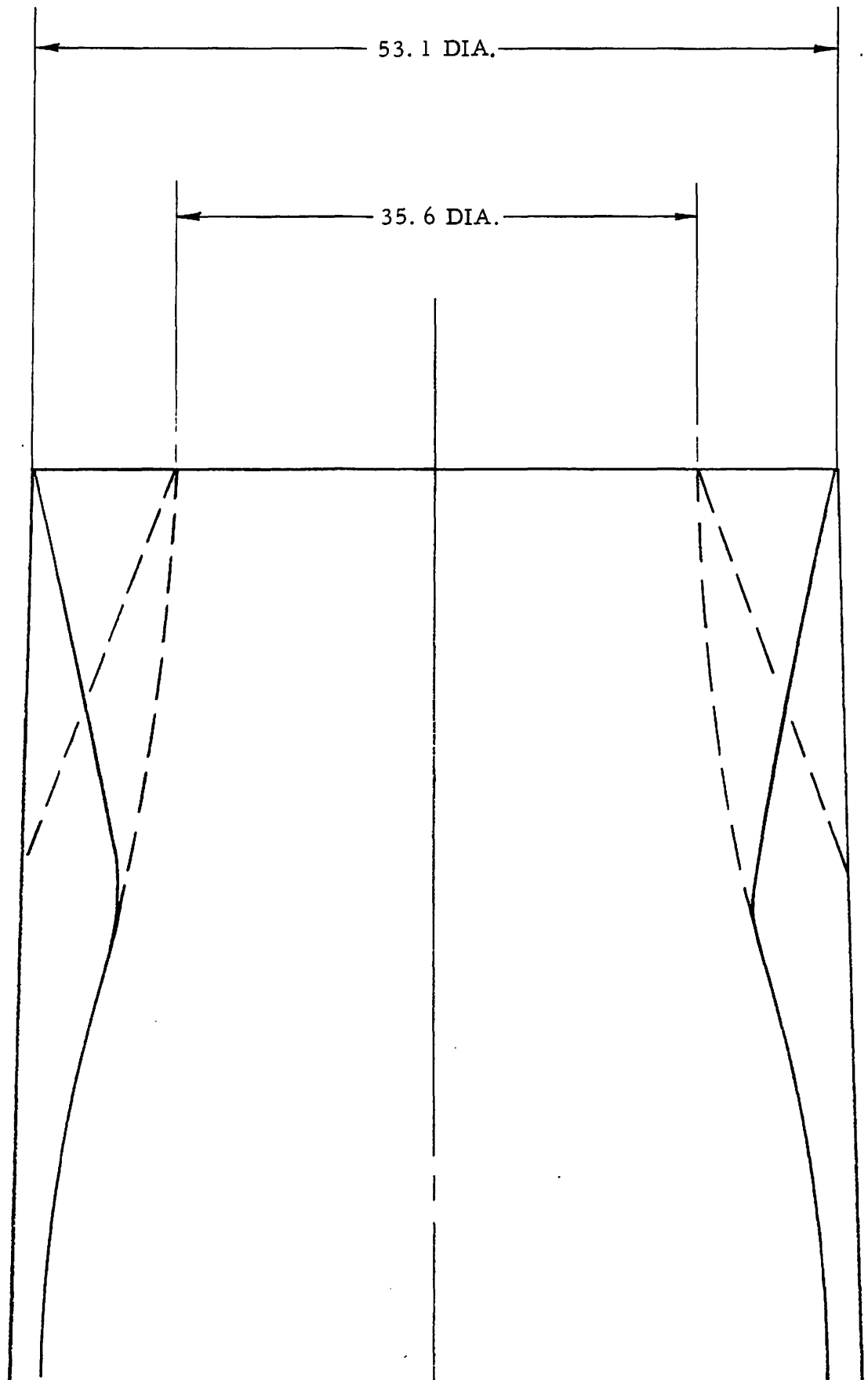
FIG. 8 DIAGRAM OF VARIABLE EJECTOR
