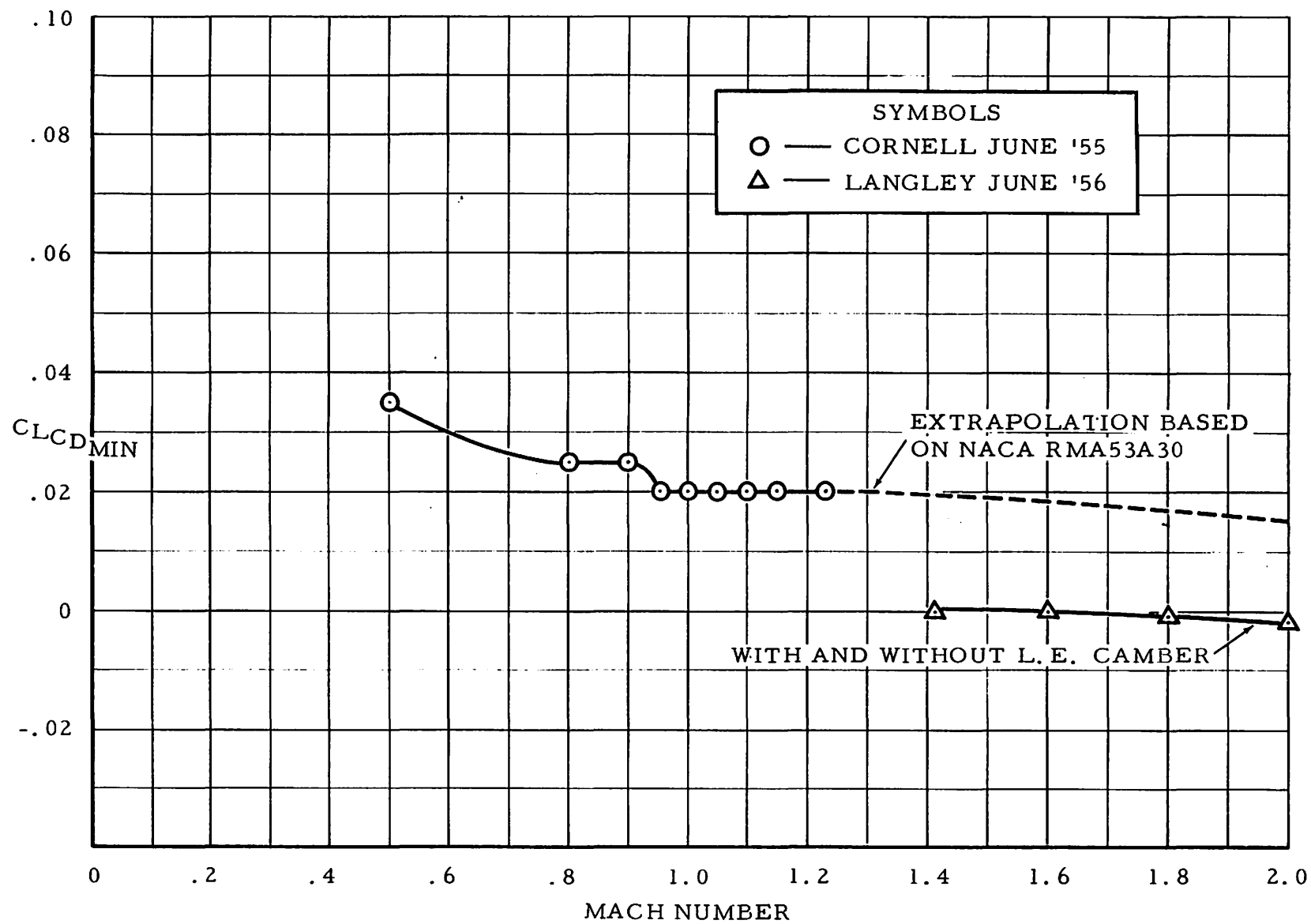
FIG. 2 VARIATION OF CF-105 LIFT COEFFICIENT AT C_{D\text{MIN}} WITH M. N.
