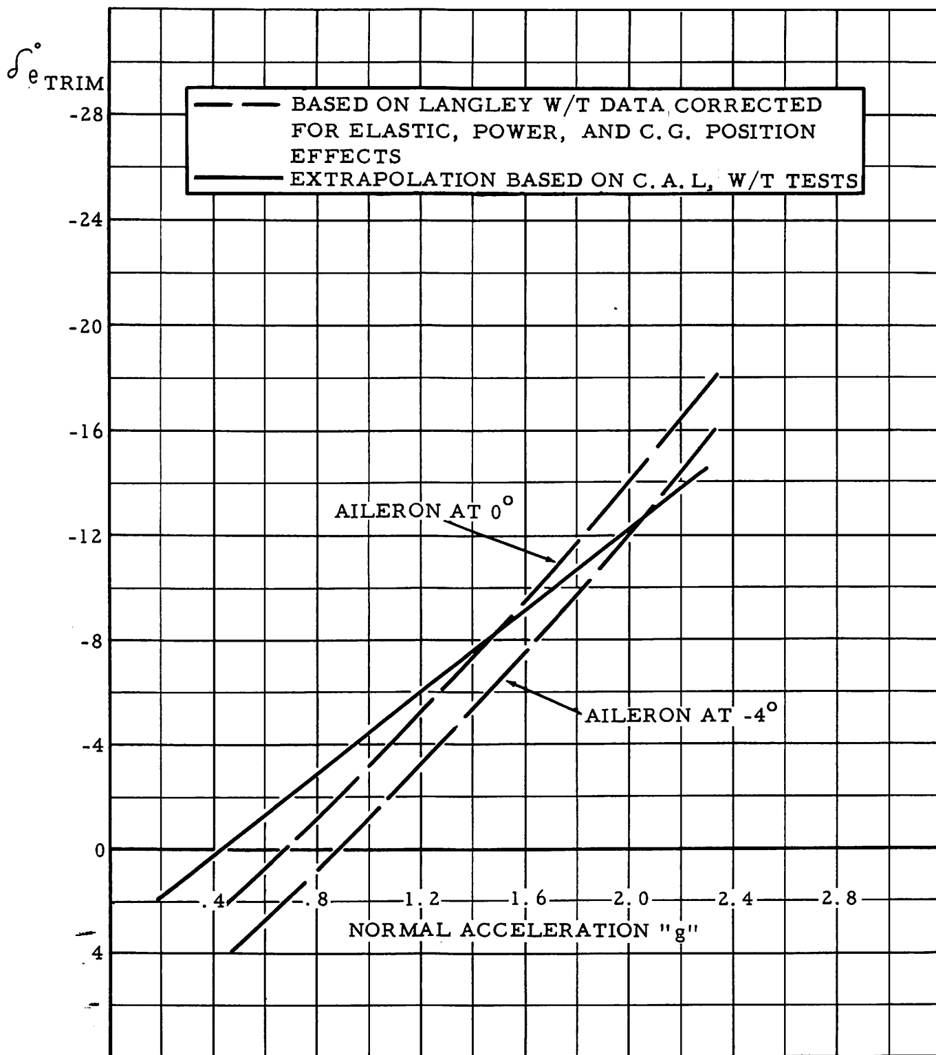
FIG. 6 CF-105 NORMAL ACCELERATION VS ELEVATOR ANGLE MACH NO. 1.5 C.G. AT 29.5% MAC
