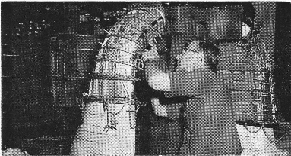
John Wilson of sub-assembly, is seen above fabricating a stainless steel heat exchanger duct.
