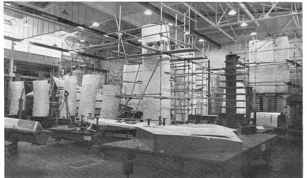
Master models of all skinned sections of the Arrow — basic forming tools for contour accuracy.
