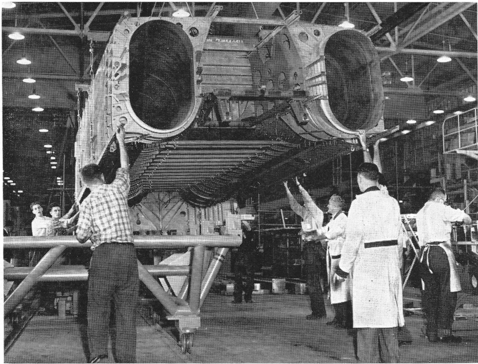
Fuselage Centre Section — the key section — for Arrow number one is seen being lowered on to its marry-up handling trolley for transfer to the main assembly jig for inner wing installation.
