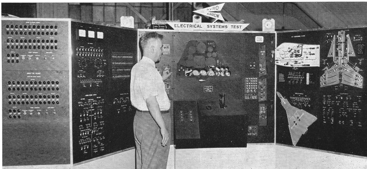
Arrow electrical system test rig simulates exactly the complete electrical system in the aircraft. Any production electrical component can be checked for serviceability in this rig. Ed Moore of systems test, is seen proving an electrical fitting for the first Arrow.
