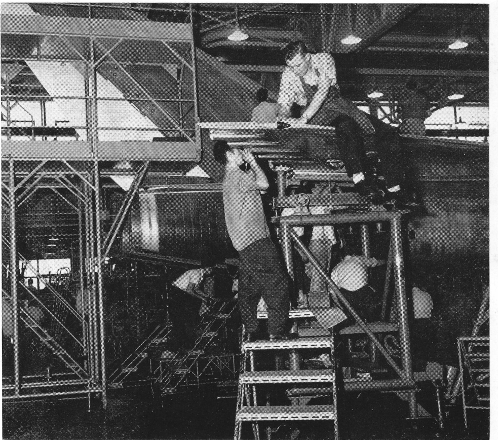
Quality Control inspectors okay each step of the complex Arrow assembly. Here, final adjustments are made to the starboard wingtip by Wally Grandey, left, and Bill Osborn of assembly.
