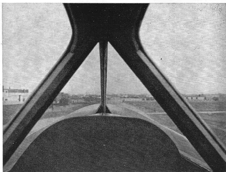
Pilots' view from the cockpit of the Arrow shows excellent visibility despite slight nose-up attitude while taxiing. Photo was taken from mobile cockpit mock-up.
