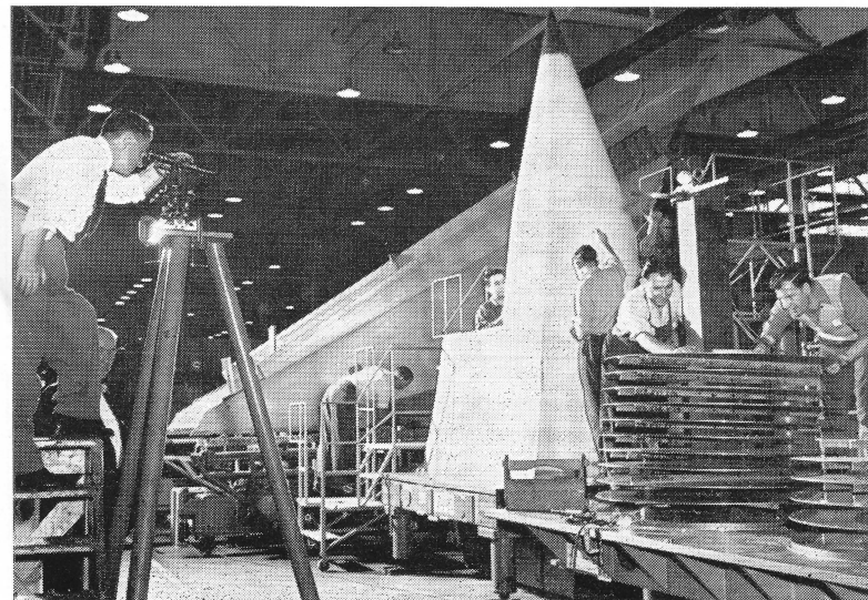
Transit is used to line up correct aerofoil forms of master models to horizontal and vertical datum lines. Work on these specially-fabricated tools began in July, 1954.
