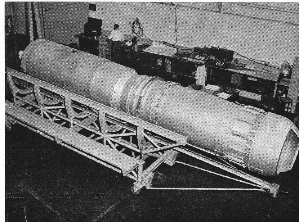
This mockup of a Pratt and Whitney J75 jet engine was used in the design of the Arrow's engine bays in order to accommodate it. Shown above cradled in its handling dolly, the mock-up is now used to aid in the development of field service techniques for engine changes.
