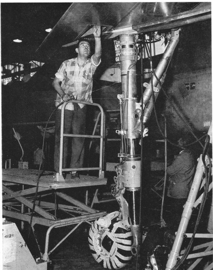
Sam Gray is shown at work on an inspection panel on the port outer wing. Detail of Arrow's bogey landing gear can be seen plainly above.
