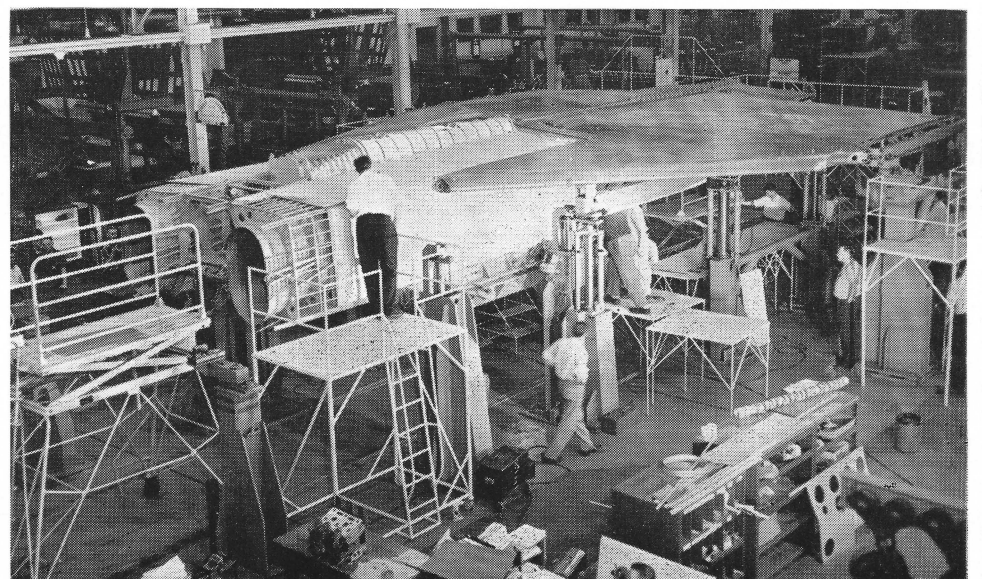
Initial stages of final assembly—skin is rivetted on centre section; inner wings are installed.
