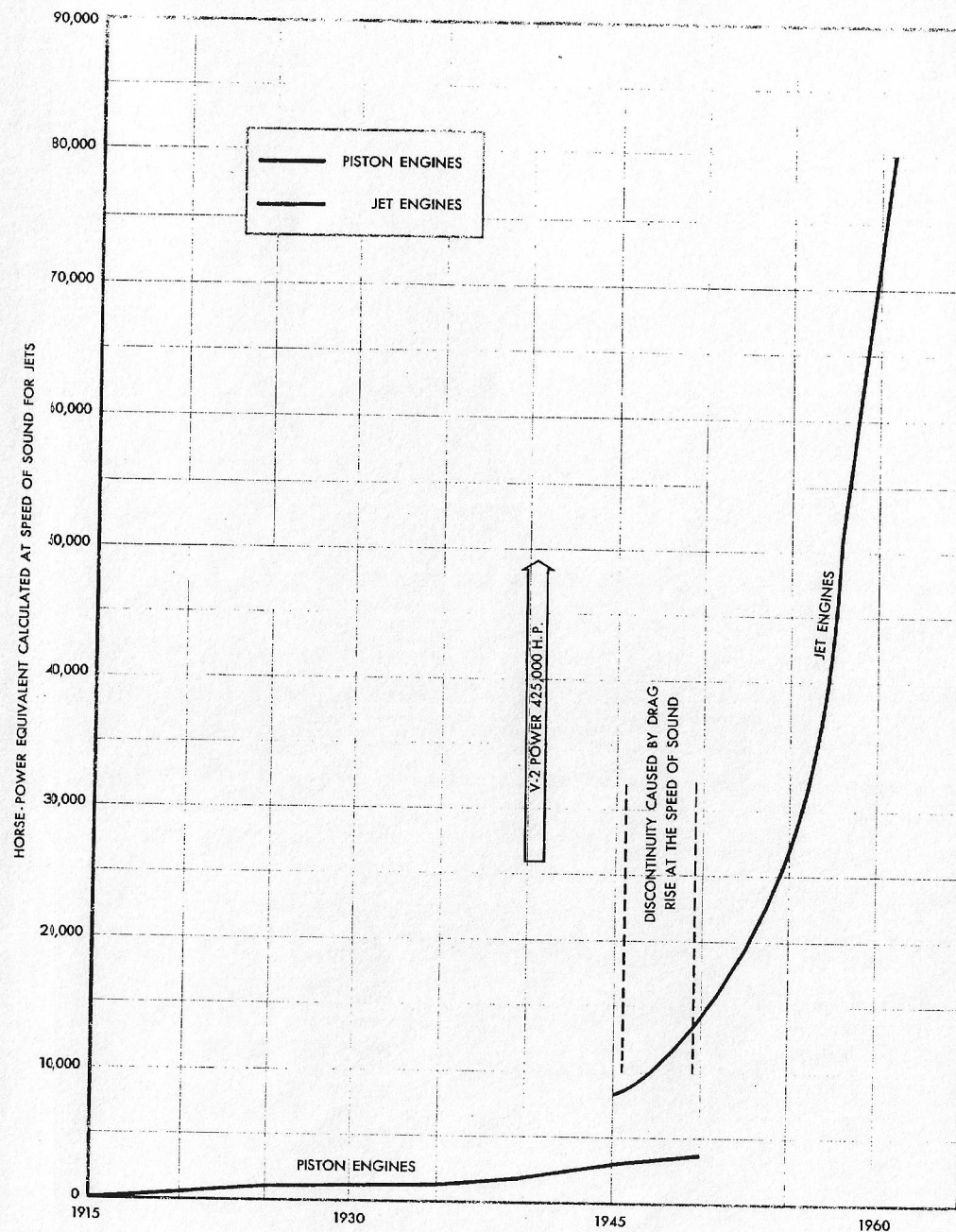
AVIATION ENGINE POWER
