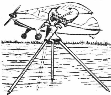
Mooring device
