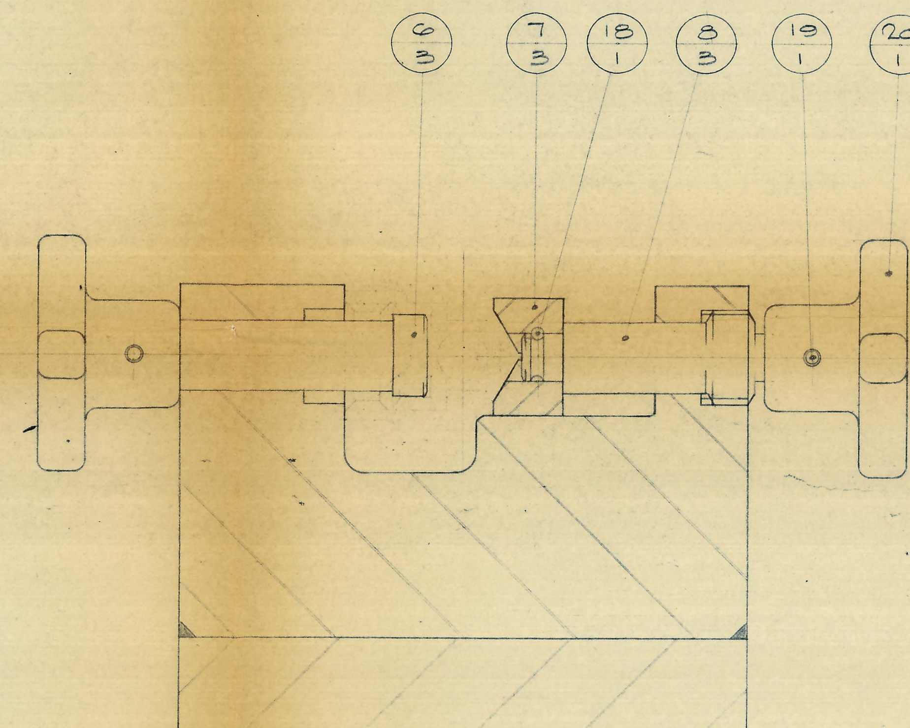
SECTION B-B
