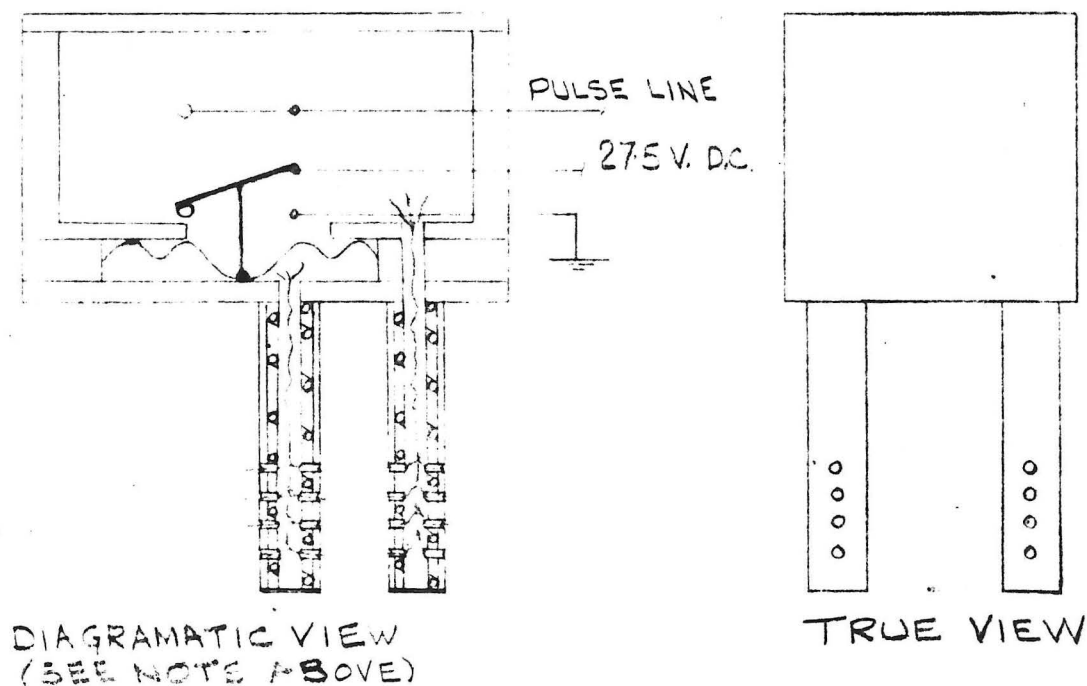
ICE DETECTOR IN DE-ICED CONDITION.
