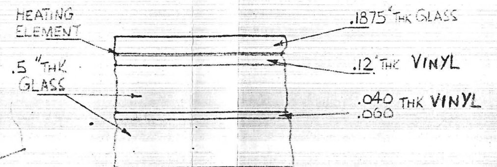
SECTION THRU LAMINATED WINDSCREEN
