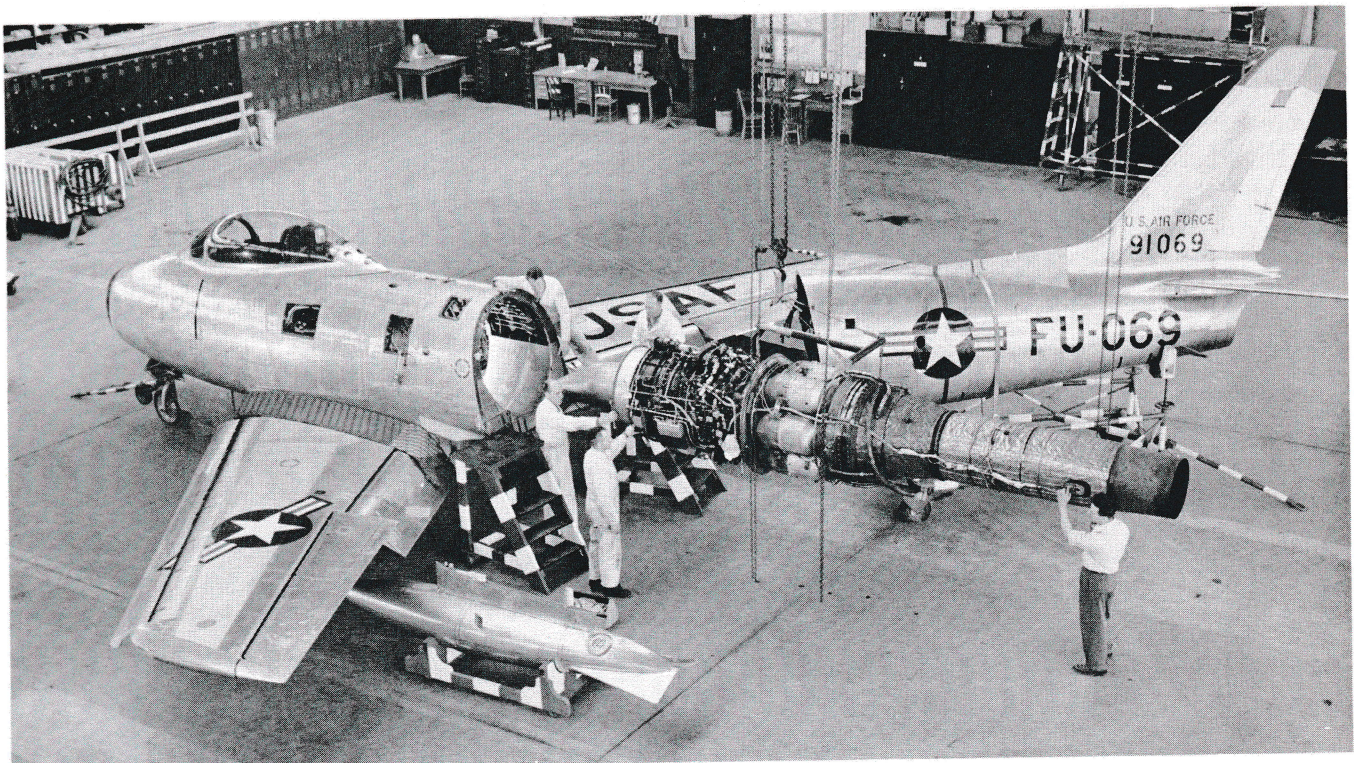
First marriage of an early Orenda engine into a U.S.A.F. Sabre in California (note the droop snoop intake modification on the engine). May 1950. This aircraft was finally flown to Canada breaking some unofficial city-to-city speed records.
