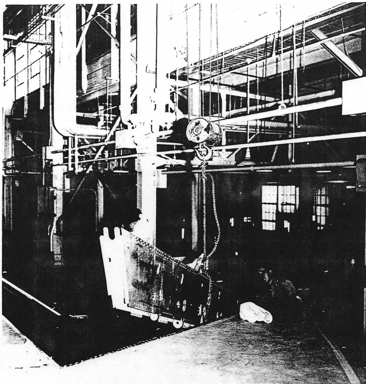
FIG. 26 REMOVAL OF ALERON CONTROL BOX
