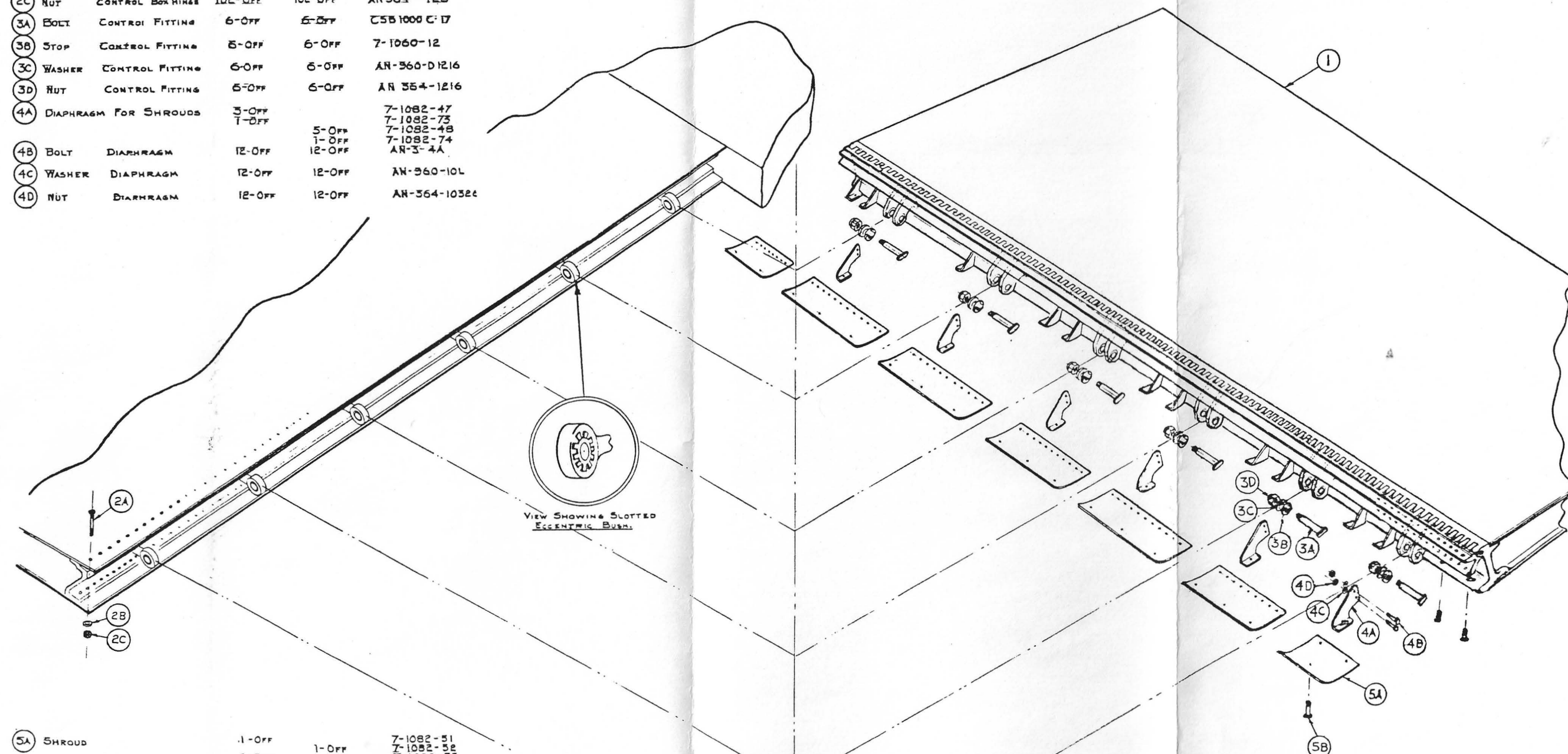
FIG.6 EXPLODED VIEW OF ELEVATOR TO ELEVATOR CONTROL BOX JNT.
