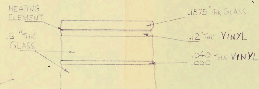
SECTION THRU LAMINATED WINDSCREEN
