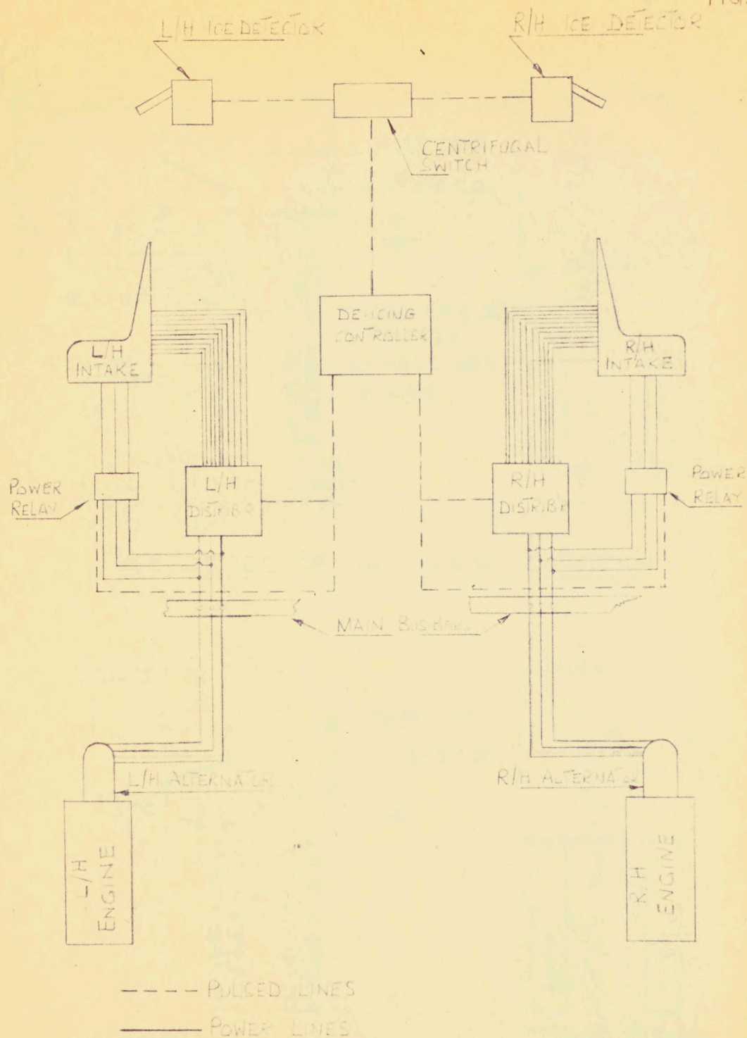
BLOCK DIAGRAM OF INTAKE DE-ICING.
