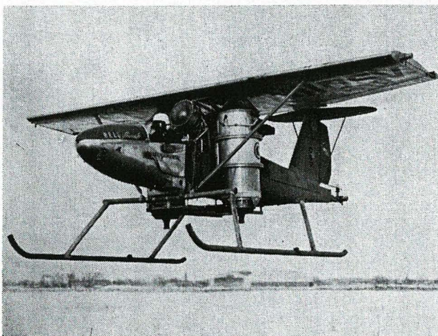
Bell's new VTO jet, above, rises vertically, then pivots jets 90 deg. to fly like a conventional fixed-wing aircraft. Another application of the same idea was revealed recently in the Bell Convertiplane (right) which has pivoting rotor-propellers.
