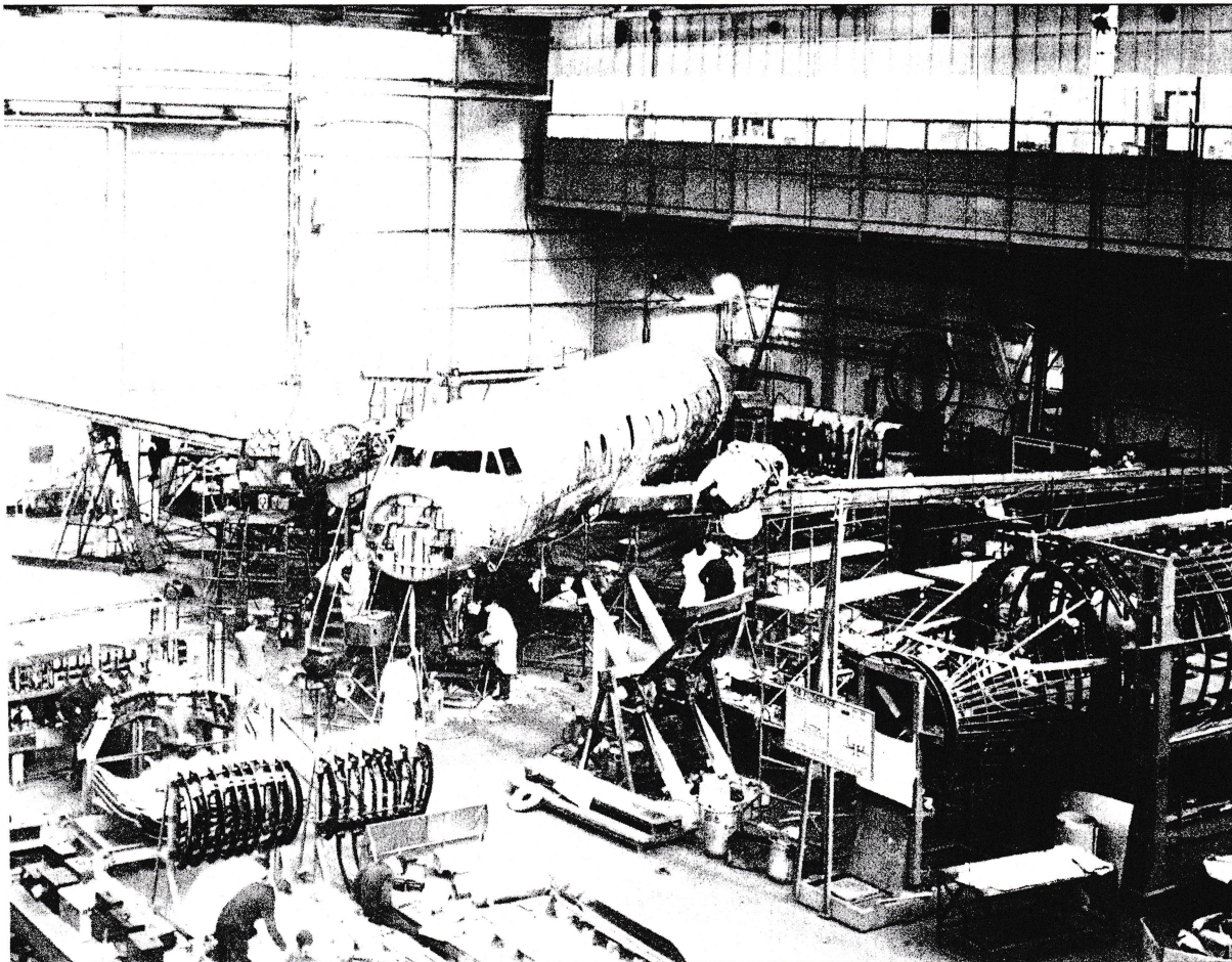
Under construction in Chadderton's experimental department in January 1960, the prototype Avro 748 was completely assembled for a variety of tests before it was dismantled for its road journey to Woodford.
