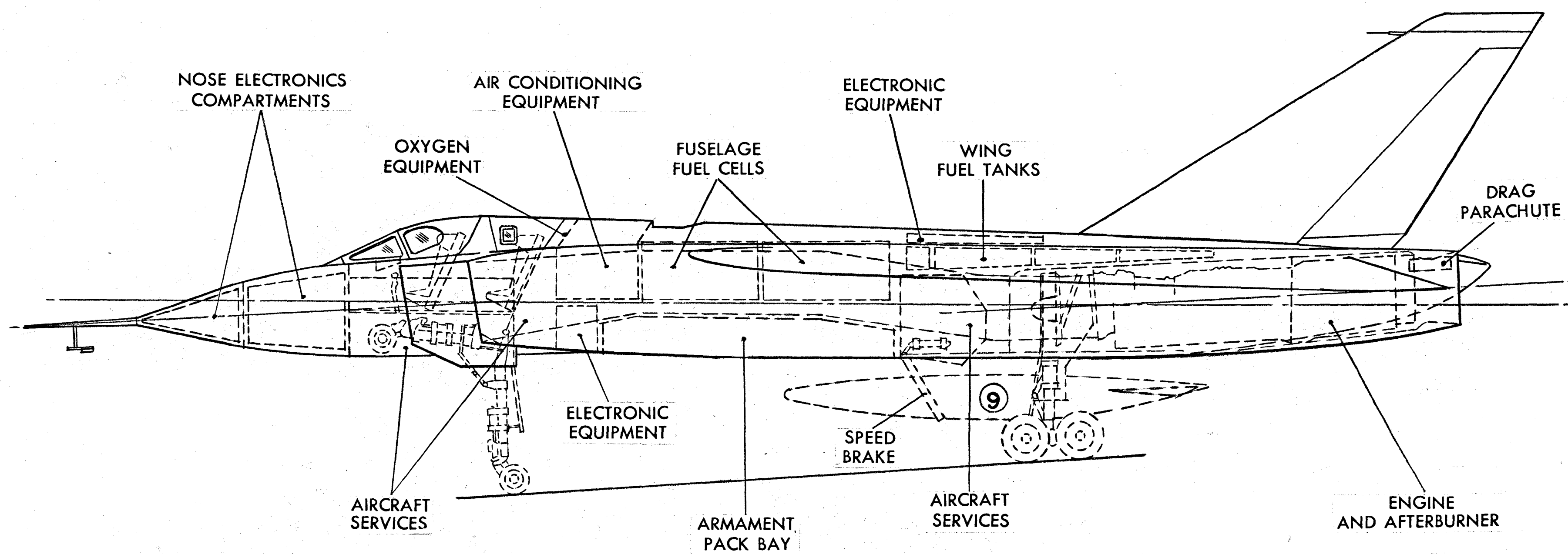
ARROW 2 LOCATION OF MAJOR EQUIPMENT
