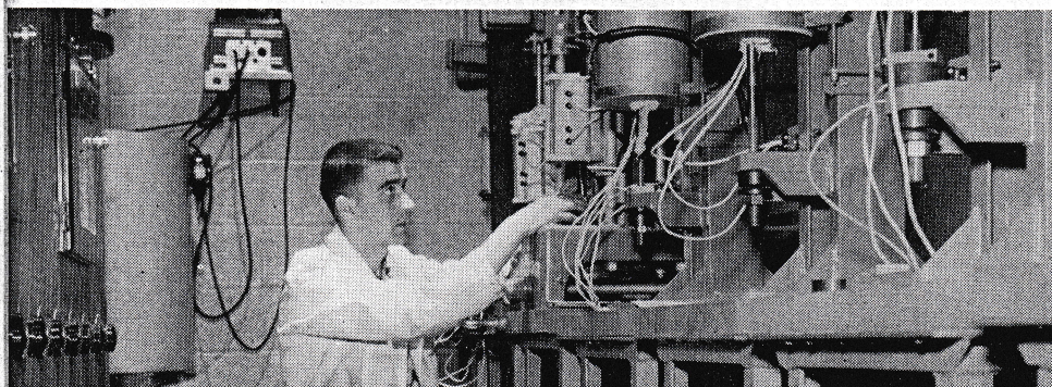
CREEP testing machine is used by lab for measuring the amount of "creep" when metal is under stress at high temperature:
