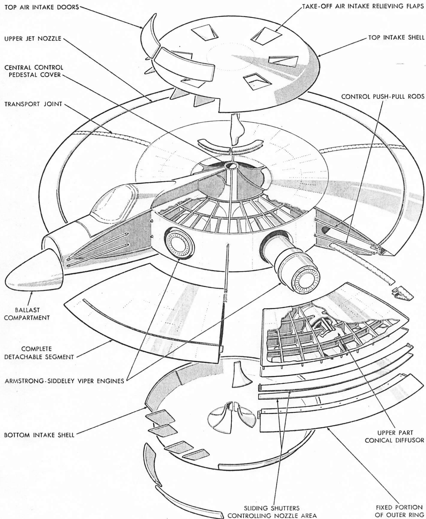
FIG. 19 EXPLODED VIEW OF TEST AIRCRAFT
