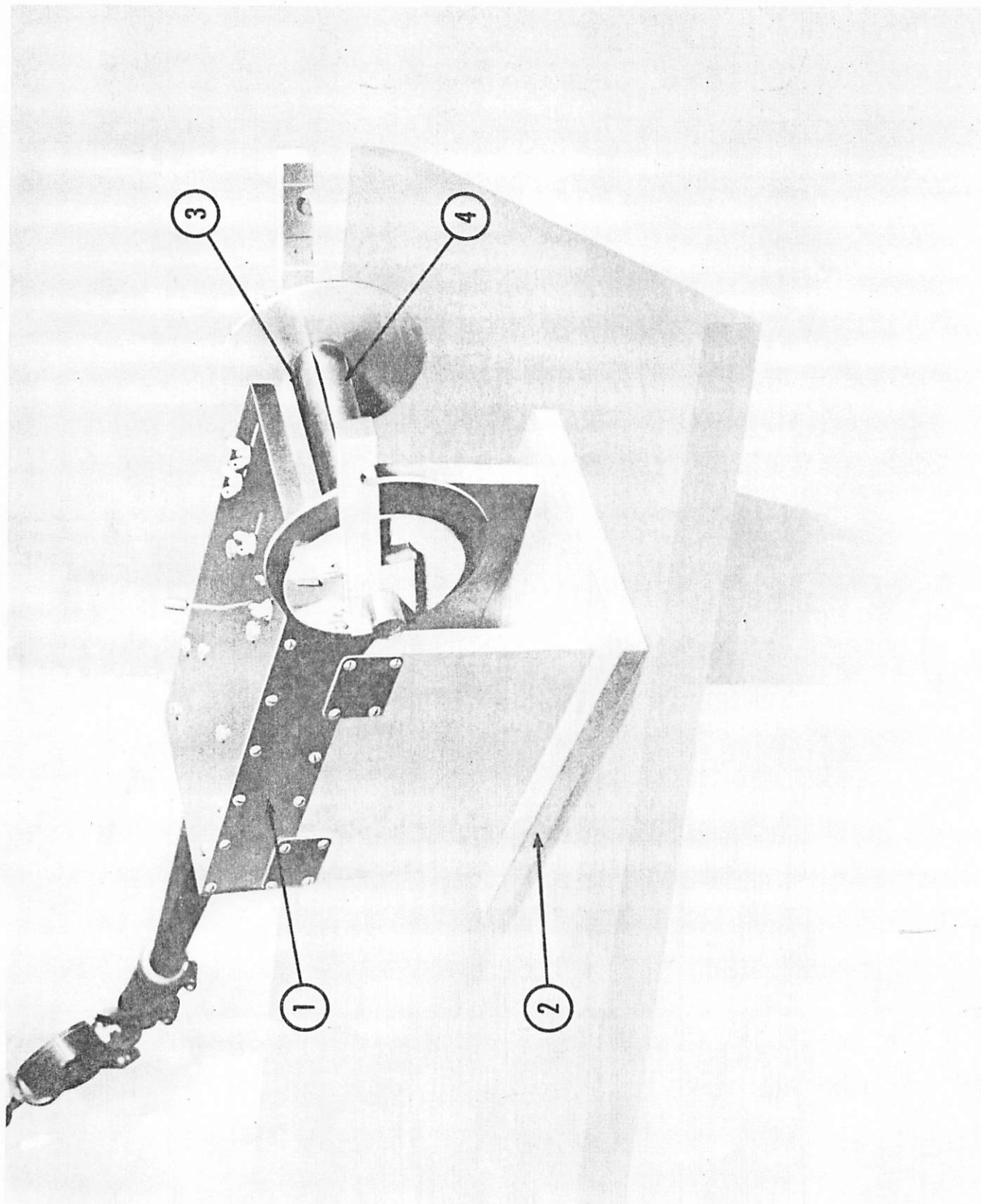
FIG. 5 COANDA EFFECT TEST RIG
