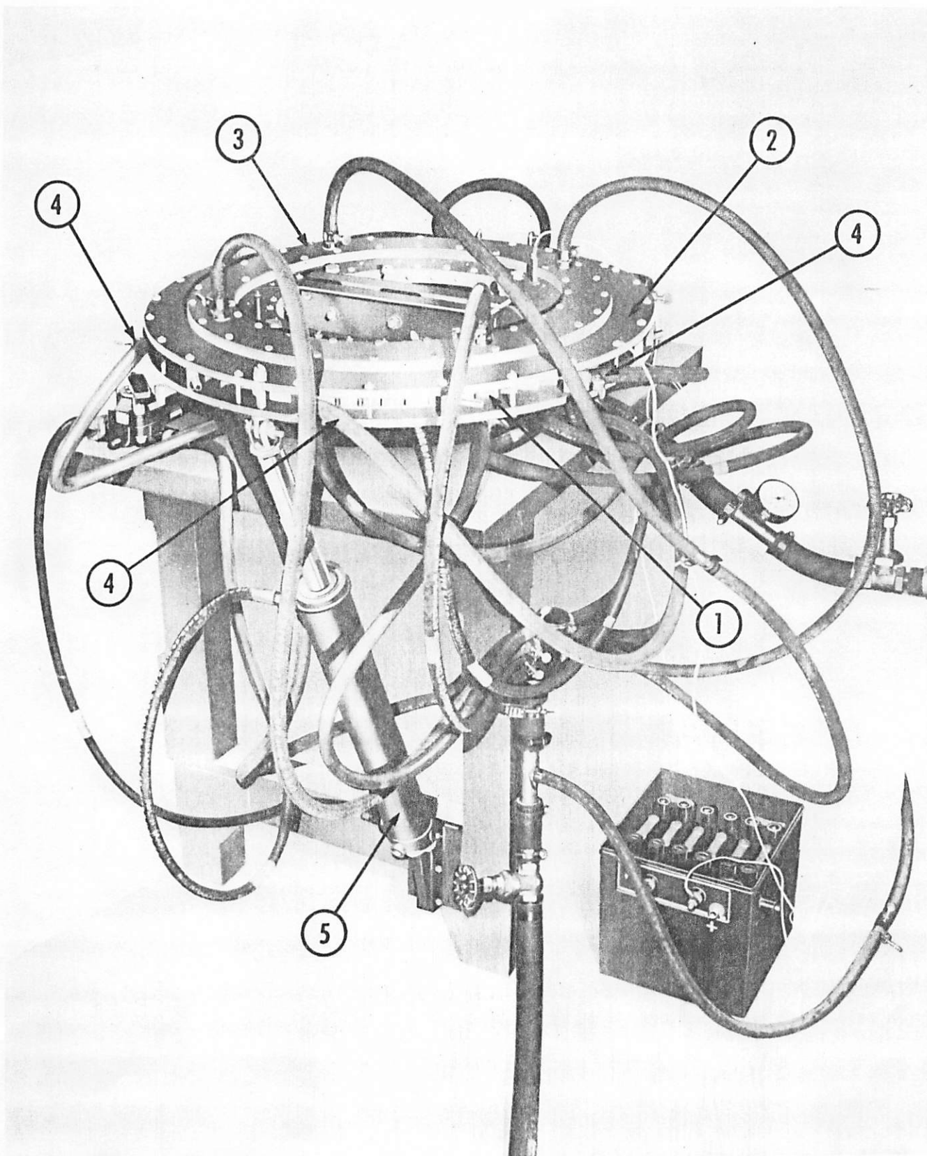
FIG. 16 AIR BEARING TEST RIG OF 1/10 SCALE MODEL
