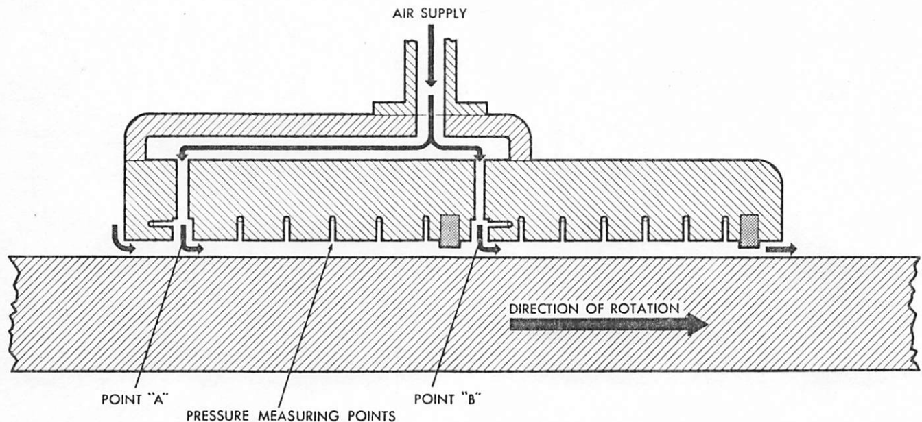
FIG. 15 SECTION DIAGRAM OF BEARING PAD
