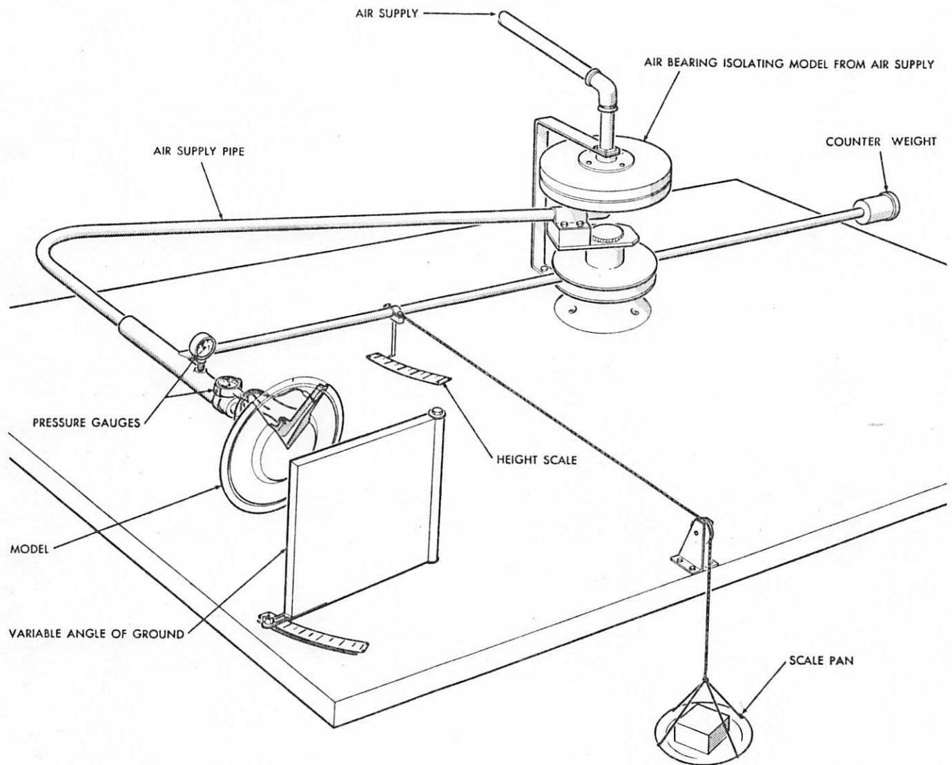
FIG. 10 GROUND EFFECT TEST RIG
