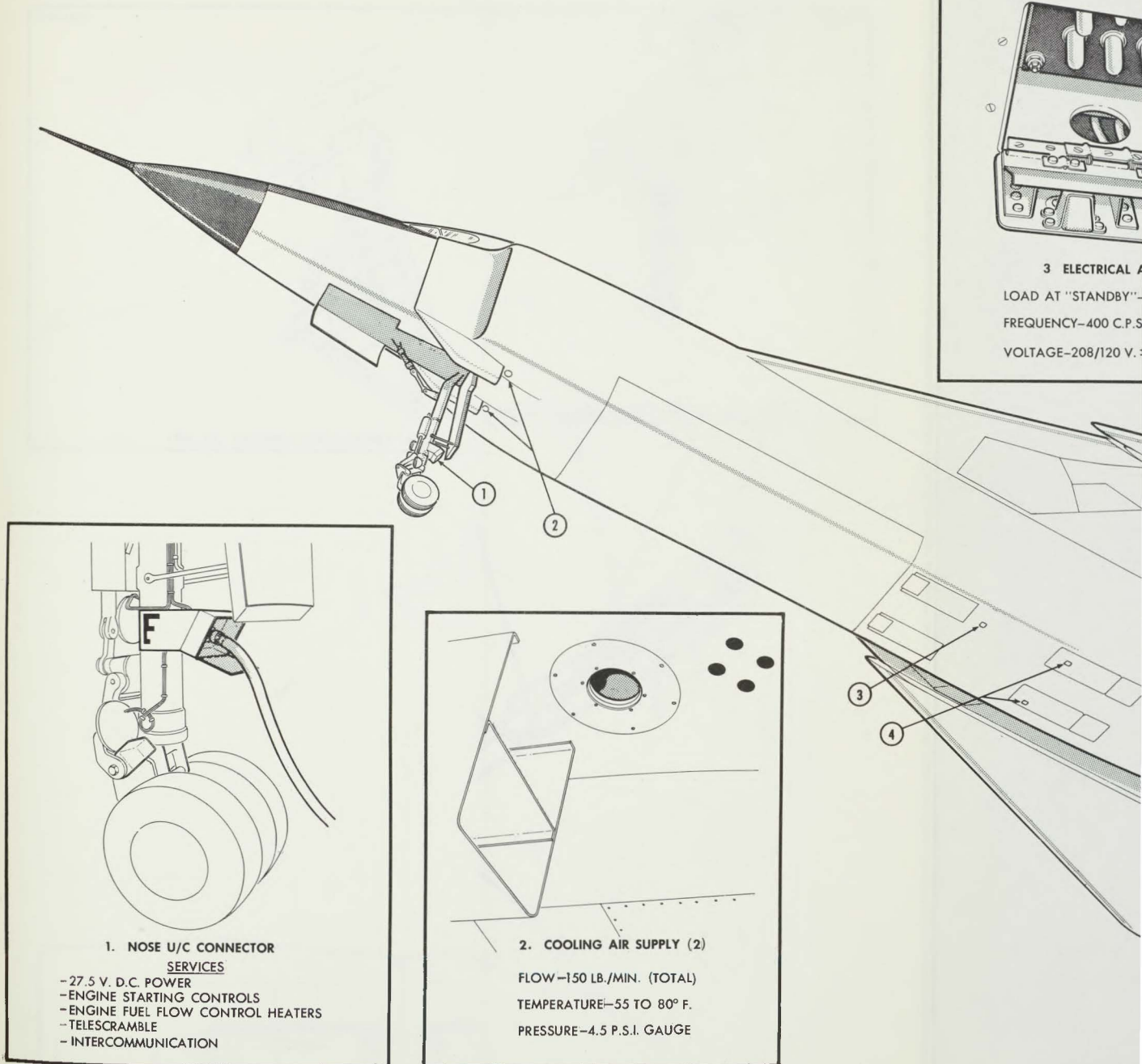
FIG. 2 ARROW 2 CONNECTIONS FOR GROUND SUPPORT SERVICES
