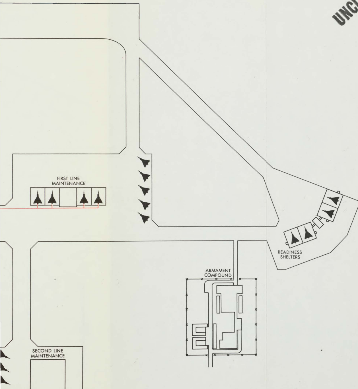
FIG. 4 TYPICAL AIR BASE LAYOUT
