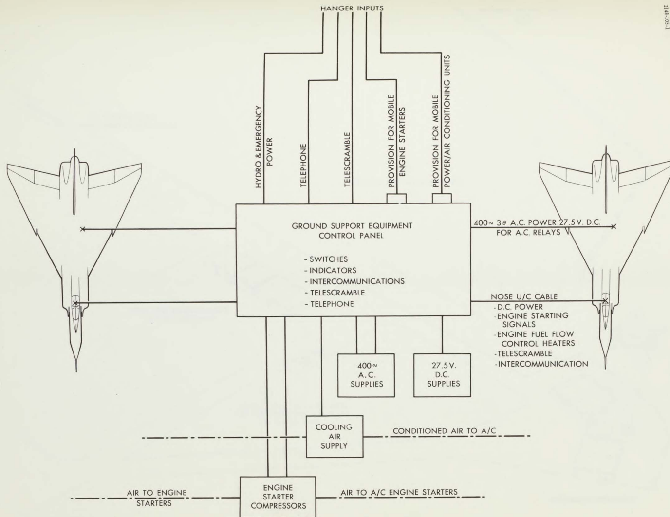
FIG. 8 SCHEMATIC DIAGRAM - ARROW 2 READINESS SERVICES
