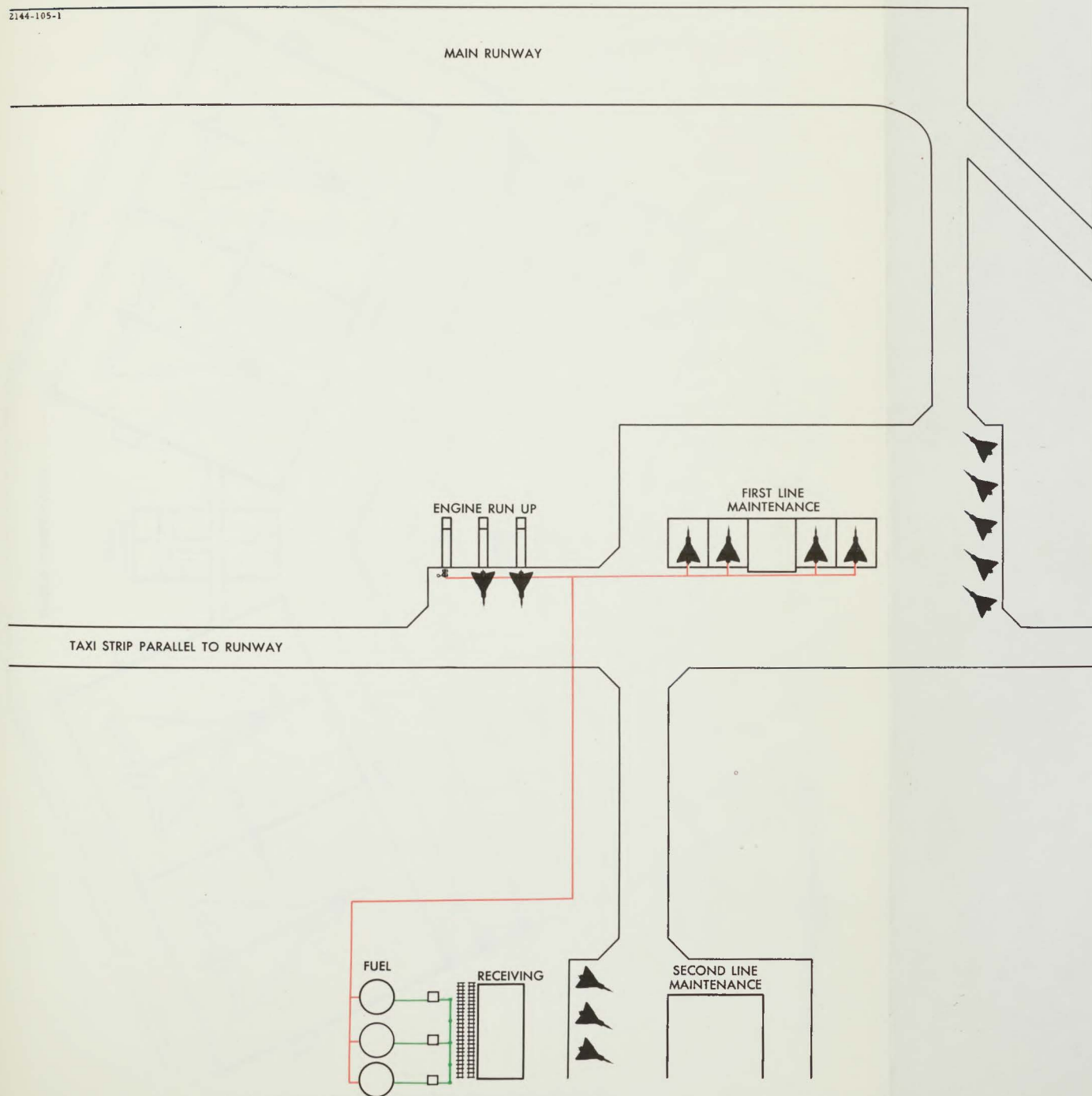
FIG. 4 TYPICAL AIR BASE LAYOUT
