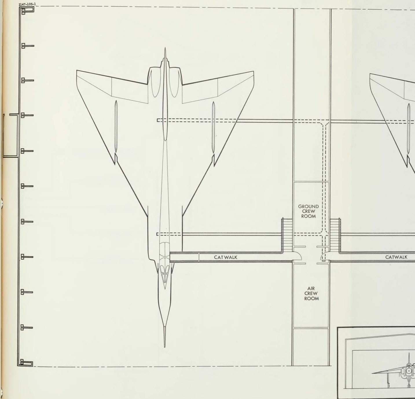
FIG. 7 ALTERNATIVE LAYOUT FOR READINESS HANGARS
