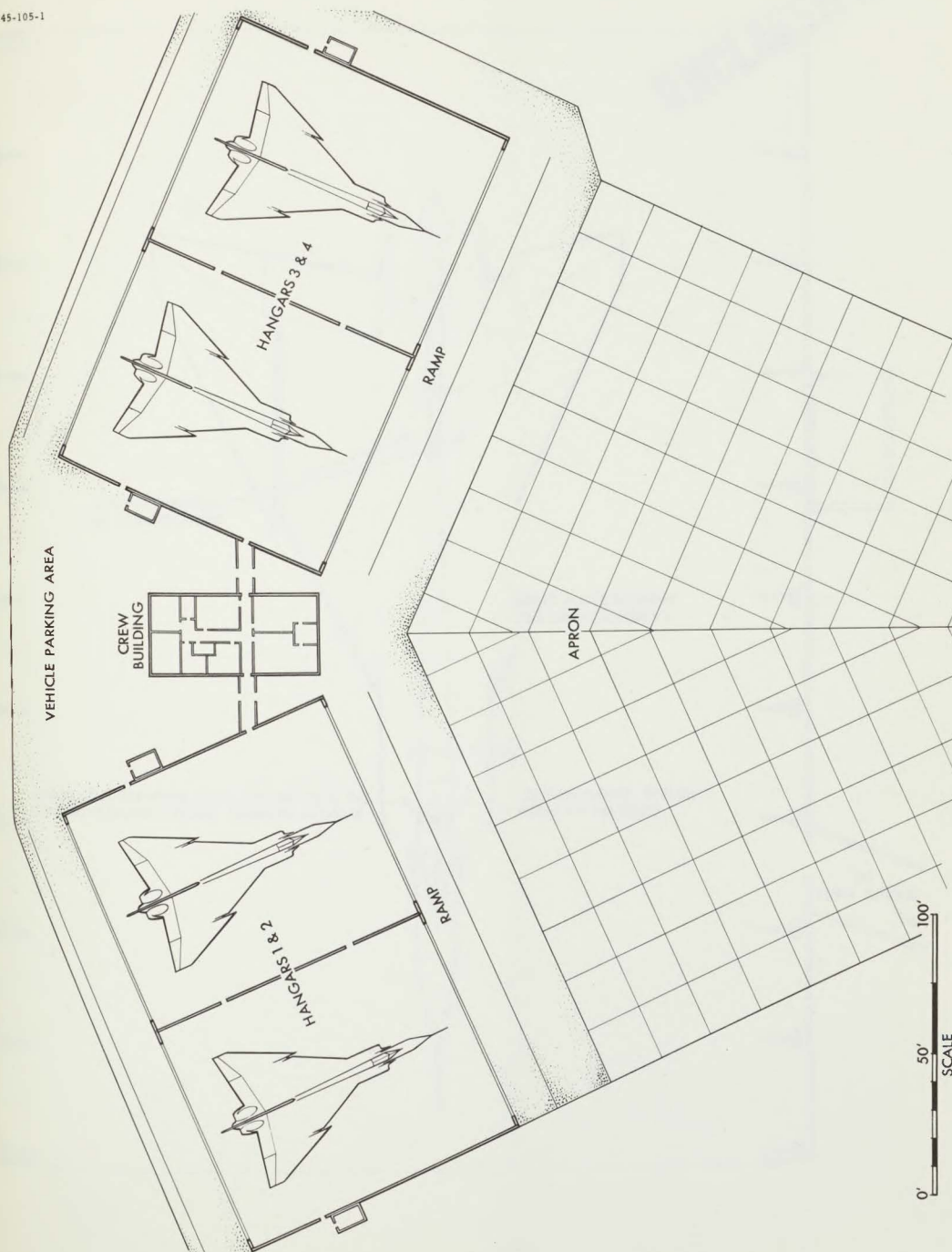
FIG. 5 LAYOUT - R.C.A.F. STANDARD READINESS HANGARS
