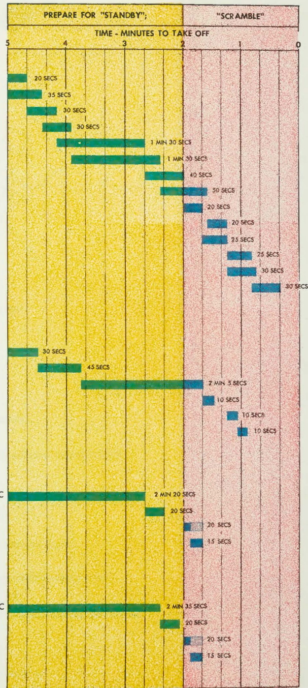
FIG. 10 TIMES & MOTIONS - PREPARATION FOR "STANDBY"; "SCRAMBLE"
