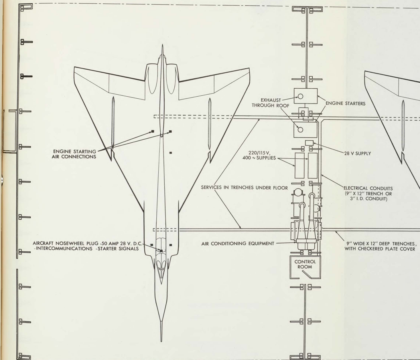
FIG.6 LAYOUT OF GROUND SUPPORT EQUIPMENT & SERVICES IN R.C.A.F. STANDARD READINESS
