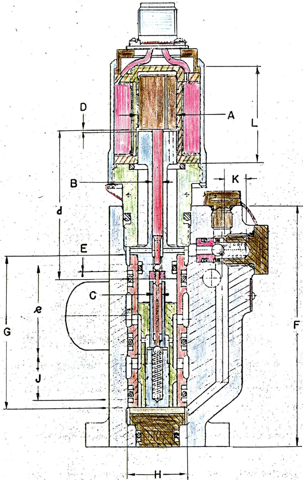
AVRO ARROW NOSE WHEEL STEERING SOLENOID CONTROL VALVE Sid Broadbent, Program Manager and Designer while at Aviation Electric Co. Montreal circa 1955
